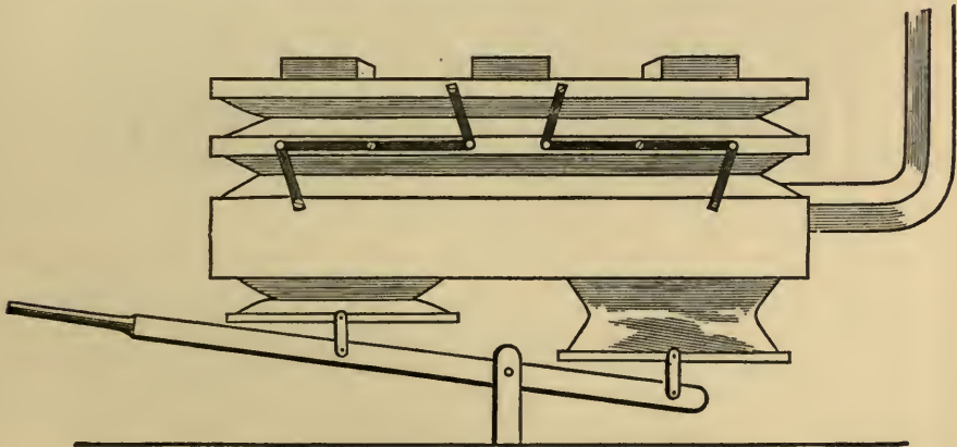
FIG. I.—BELLOWS.
