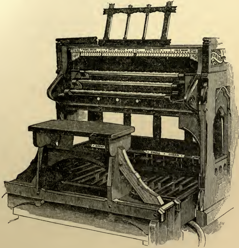
FIG. 9.—CONSOLE OF HOPE-JONES ELECTRIC ORGAN (With connecting Cable).
