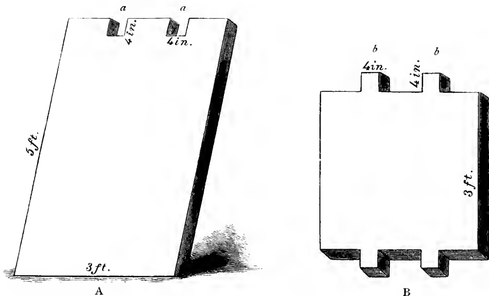
NO. 1907. PATTERN OF THE SLABS, FORMING THE DOUBLE PARALLEL CIRCLE ENCLOSING THE AGORA.
