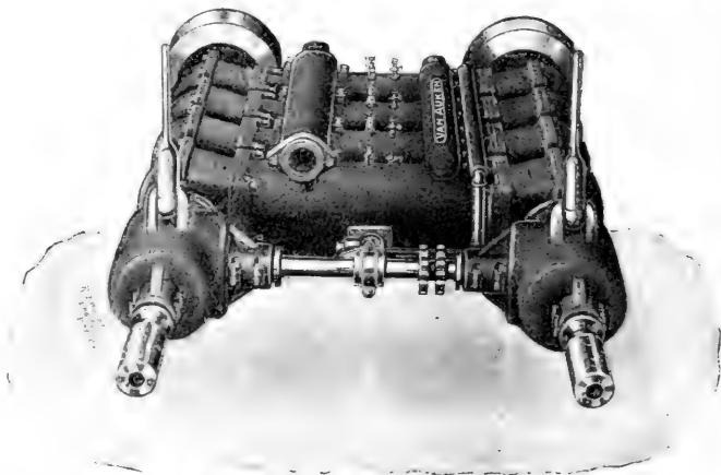
35 AND 65 H. P., 4 CYLINDER
