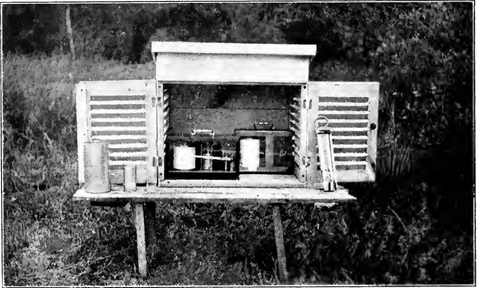
Keewatin, M. H. S. Evaporation Station. Meteorological Instrument Shelter.
