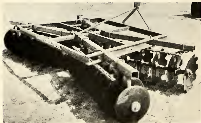
The Massey Ferguson tandem disc harrow joins MF's line of tillage equipment for 1980. MF 320 features easy gang-adjustment and heavy-duty U-bolt bearing supports.
