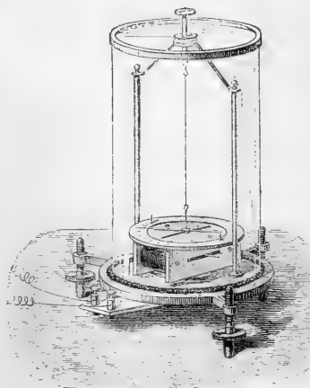
FIG. 8.—Astatic Galvanometer.
