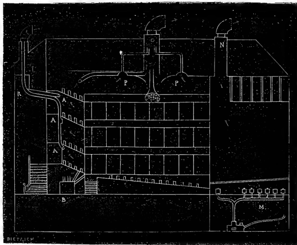
FIG. 1.—Ventilation of a Theatre (Chavannes' system).
