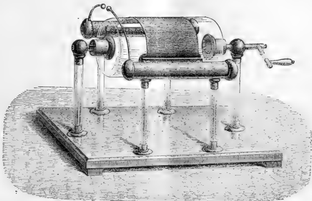
FIG. 11.—Nairne's machine, furnishing the two electricities.
