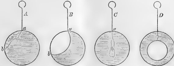
FIG. 1.—Experiments in liquid films.
