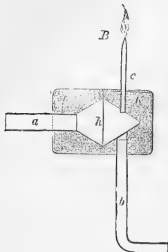
FIG. 3.—The Flame Manometer.
