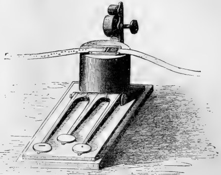
FIG. 19.—The "Perforator," for cutting out the message on the paper ribbon.
