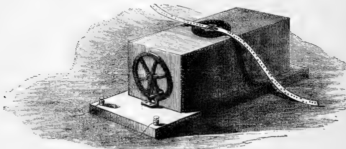
FIG. 21.—Wheatstone's Automatic Tel. graph. The "Transmitter."
