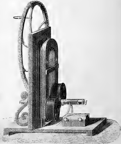
FIG. 15.—Magneto-electric machine.
