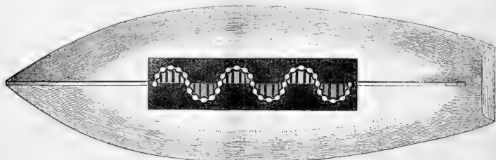
FIG. 3.—The same boat looked at from below, the apices of the rods forming undulating propeller being seen.
