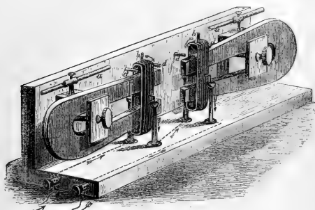
FIG. 18.—Mr. William Sykes Ward's Telegraph, September 1847.
