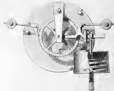
FIG. 2.—Dial Mechanism of Street and Private Clocks.
