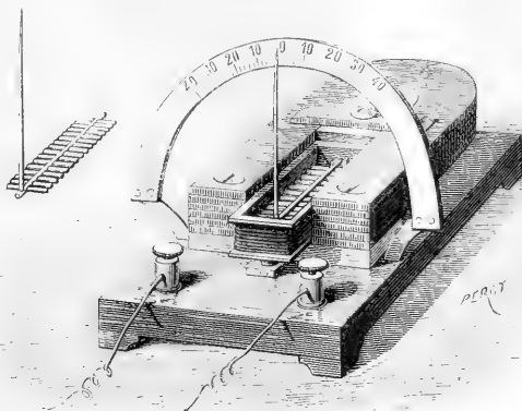
Marcel Deprez's Galvanometer for very strong currents.
