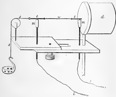
w , fine wire; t , thicker copper terminals; m , mercury cups over which l pass; s , string kept tight by small load; l , line wires to microphone; d , drum head which distributes the sound.
