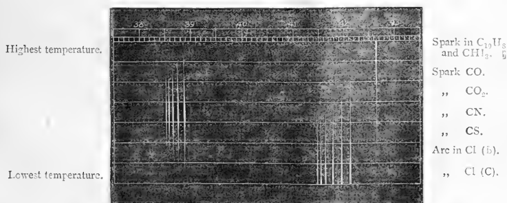
FIG. 5.—The photographed spectra of some carbon compounds.
