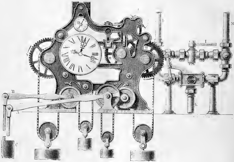
FIG. 1.—Distributing Clock of Compressed Air.
