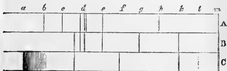
FIG. 1.—A. Highest temperature. C. Lowest temperature.
