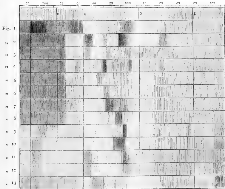
1, Water; 2, Ammonia; 3, Ammonia in Alcohol; 4, Ethylamine; 5, Amyl Alcohol; 6, Ethyl Alcohol; 7, Aldehyd; 8, Acetic Acid; 9, Benzene; 10, Toluene; 11, Aniline; 12, Turpentine; 13, Turpentine.
