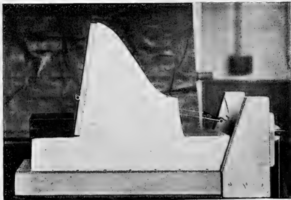
FIG. 1.—Vyrvny-type dam, moderate water pressure.
