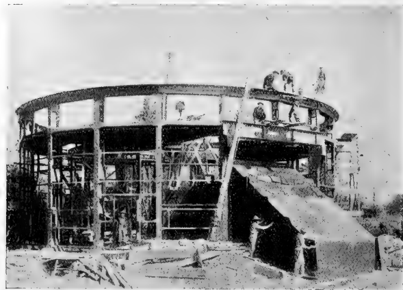
FIG. 1.—Steel Building for 60-inch Reflector, Mount Wilson Solar Observatory.
