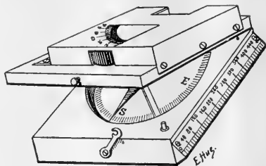
FIG. 5.—M. Hue's combined compass and clinometer.
