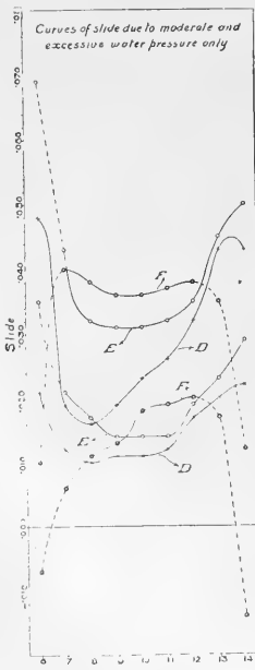
Curves of slide on the horizontal sections D, E, F, G.
