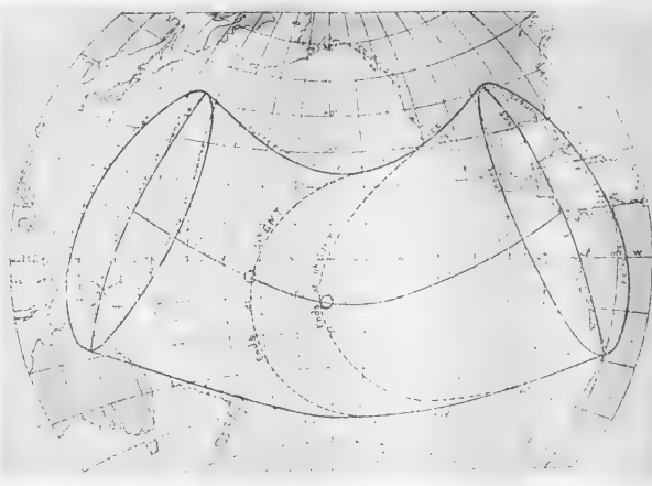
FIG. 1.—The track of the total solar eclipse of January 3, 1908. The small circles on the central line denote the positions of the two islands from which totality can be observed.
