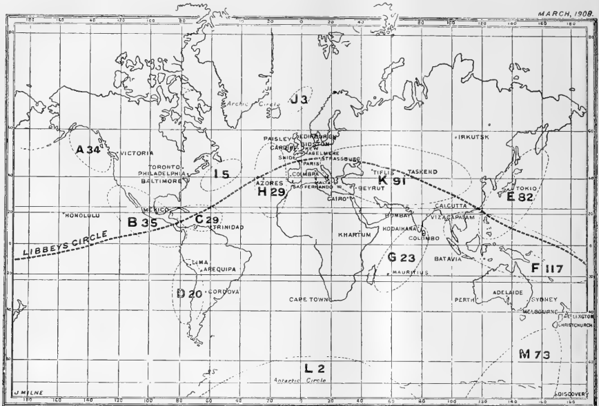
FIG. 1.—Stations in cooperation with the British Association working with similar instruments (Milne pendulum). Number of world-shaking earthquakes since 1899 which have originated in districts marked A, B, C, &c., are indicated.
