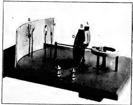
FIG. 1.—Skeleton apparatus showing the principle of the optophone.
