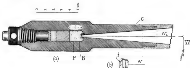
FIG. 1.—Chamber used in early experiments.
