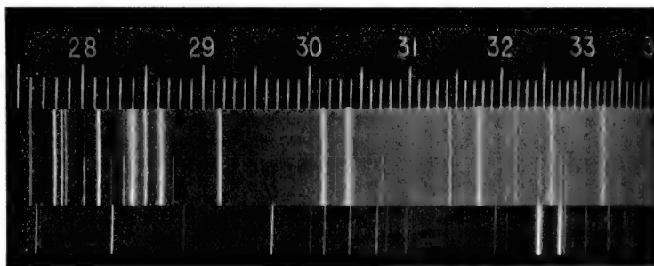
FIG. 2.—Print from negative taken on spectrograph with wave-length scale. Top strip, sample of reputed "pure tin." Middle strip, sample of commercial tin. Bottom strip, short exposure of copper spectrum. The presence of copper in the commercial tin is shown by the presence in the corresponding spectrum strip of the two copper lines at 3247 and 3274. A trace of copper is present in the "pure" tin.
