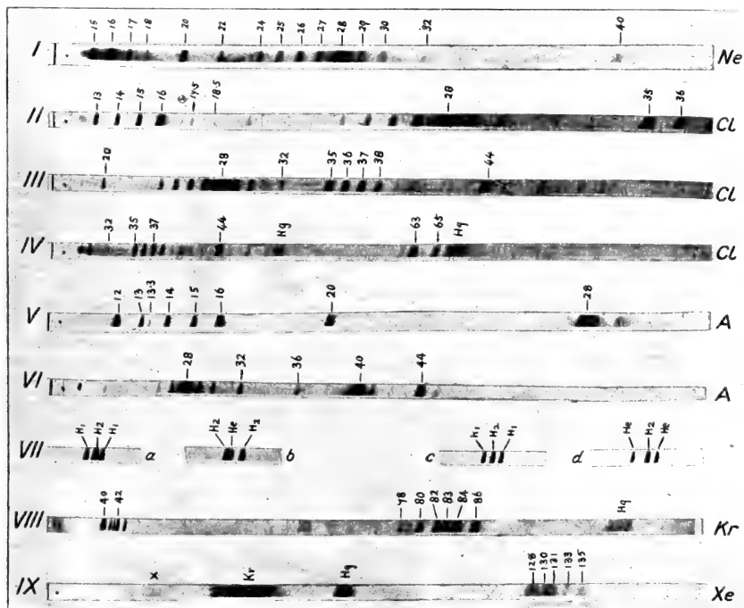
FIG. 2.—Typical mass-spectra.
