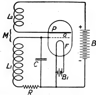
FIG. 2.—Connections for generator valve.
