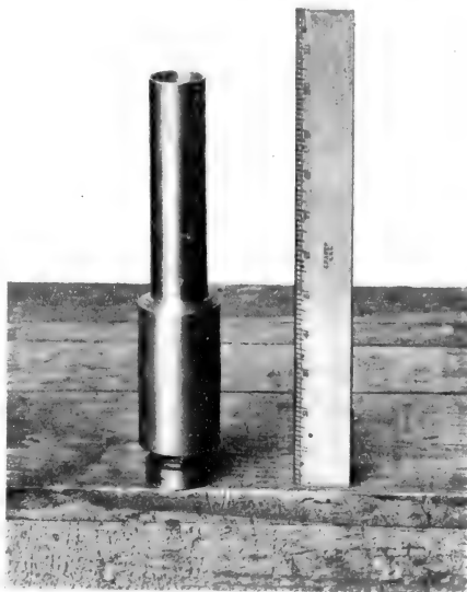
FIG. 2.—Chamber by which ejected gases were given a velocity of nearly 8000 ft. per sec.
