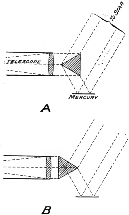
FIG. 1.—Principle of construction of the prismatic astrolabe.
