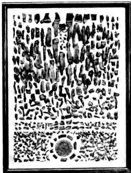
FIG. 3.—Fragmentation of 18-pr. shell by 80/20 amatol.
