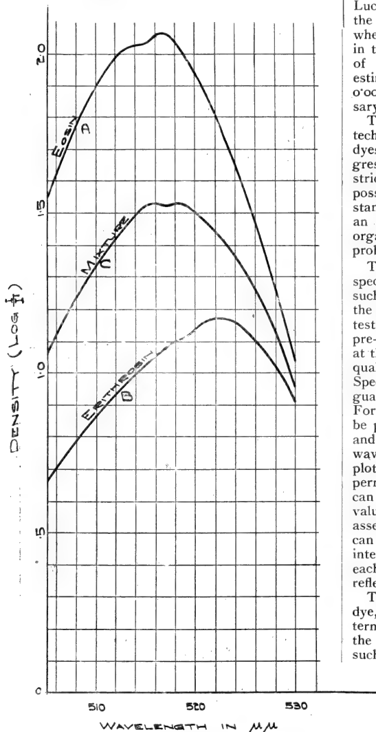
FIG. 3.—Curves plotted from results obtained in examining dyes with the spectrophotometer.
