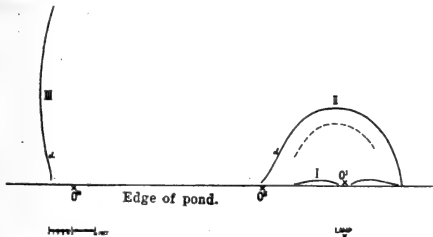
FIG. 1.—O, OII, OIII, three positions of the observer's eye; I, II., III., the bows seen in these positions; a, points of double curvature.
