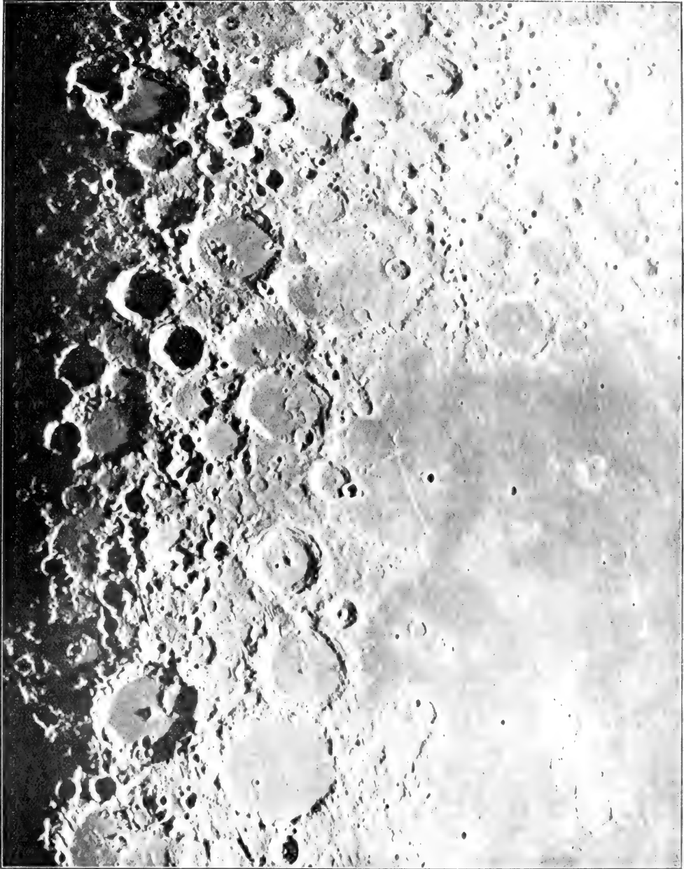
FIG. 1.—North central portion of the moon at last quarter. Photographed with the Hooker telescope of the Mount Wilson Observatory September 15, 1919, by Mr. F. G. Pease. Scale: 1 in. = about 90 miles.
