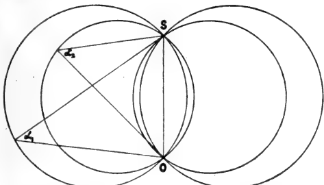
FIG. 2.—S, source of light; O, eye of observer; a_1, a_2 , angles of minimum deviation for primary and secondary bows respectively.
