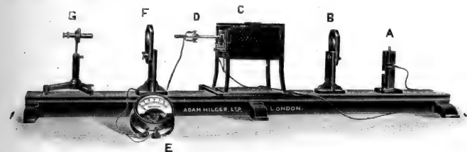
FIG. 1.—Twyman's apparatus for the determination of annealing temperatures. A, B, F, G, optical system; C, electrical furnace; D, pyrometer; E, temperature recorder.
