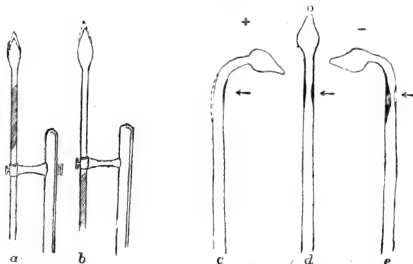
FIG. 5.—Effects of direct and indirect stimulus: a, Stimulus applied directly at the growing region inducing retardation of growth or contraction as represented by dotted line (stimulated area in this and in following represented as shaded); b, stimulus applied indirectly (at some distance from growing region) gives rise to acceleration of growth and expansion; c, stimulus applied at right side of organ causes contraction of that side and expansion of the opposite side, thus giving rise to positive curvature towards stimulus; d, excitation transmitted to the opposite side causes neutralisation; e, excitation caused by intense stimulation is transmitted across and thus reverses the normal curvature to negative, i.e. away from stimulus.
