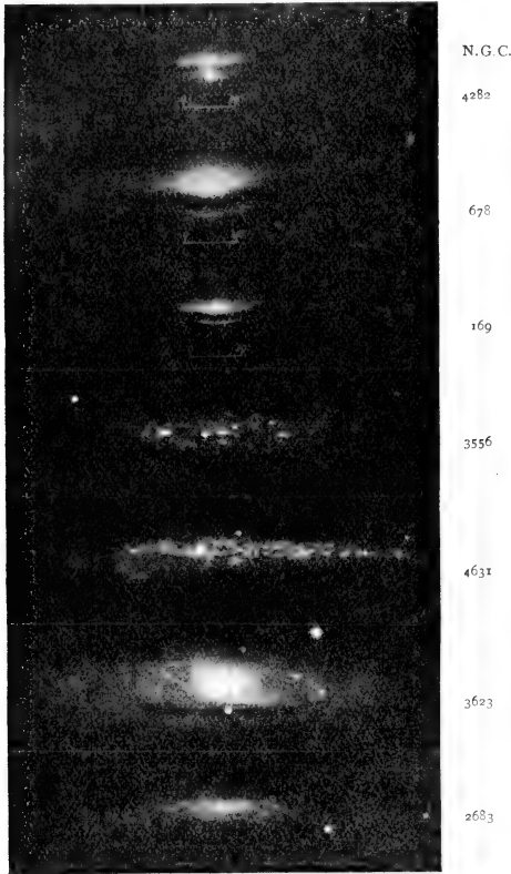
FIG. 2.—Spiral nebulae seen almost, but not exactly, edgewise, and some the planes of which make a small but appreciable angle with the line of sight, showing clear evidence of dark lanes. (H. D. Curtis.)
