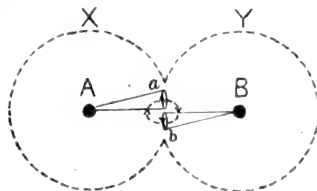
Model of hydrogen molecule.
