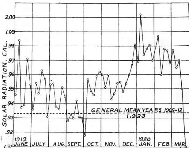
FIG. 2.—Five-day means observed at Calama, Chile, 1919-20.
