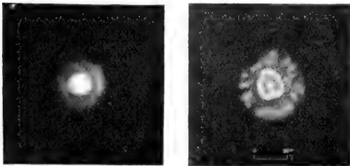
FIG. 5.—On the left a photograph of N.G.C. 2392, a double-ring planetary nebula; and on the right a composite drawing of the same made from several photographs to show details of the structure not attainable from any single photograph. (H. D. Curtis.)
