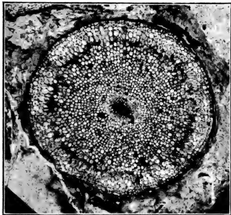
Photo] [Dr. Kidston. FIG. 2.—Aerial stem of Rhynia major seen in transverse section ( \times 20 ).
