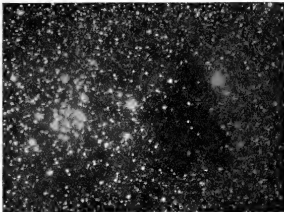
FIG. 4.—A "dark nebula" (17h. 57m., -27°50') visible through its projection upon the background of stars, and not considered to be "a hole" in the Milky Way. Note the circular protuberance at the south-west corner, as clear-cut as an ink-drop and perfectly dark. (H. D. Curtis.)
