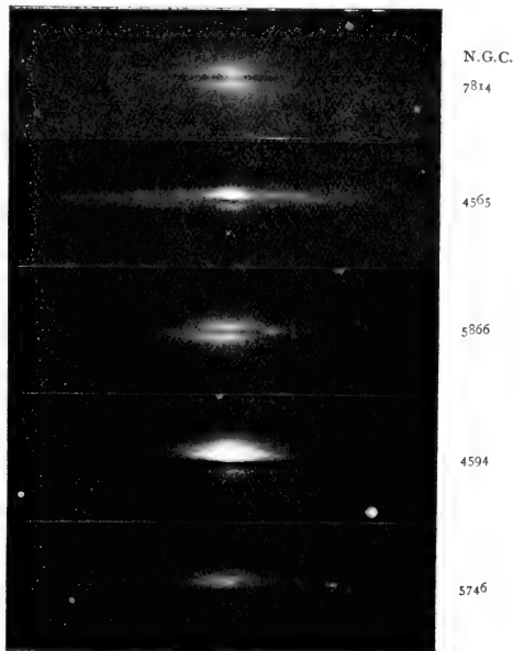
FIG. 1.—Spiral nebulæ seen almost exactly edgewise and showing indubitable evidence of dark lanes. (H. D. Curtis.)
