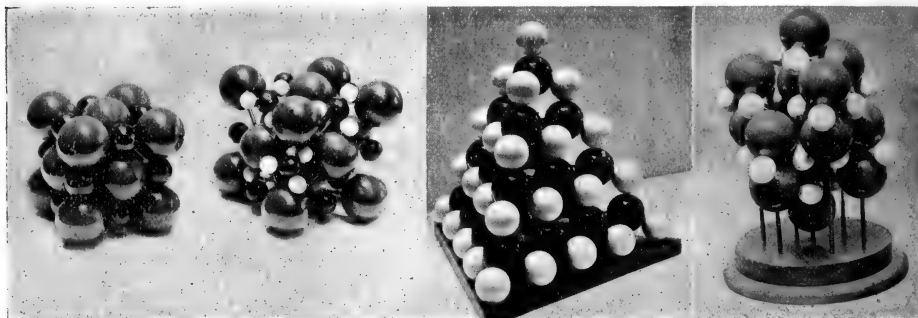
Potassium chloride, KCl.
