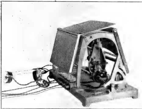
FIG. 3.—The optophone complete with book-rest.
