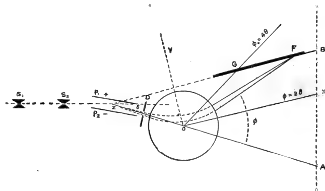
FIG. 1.—Diagram of positive-ray spectrograph.
