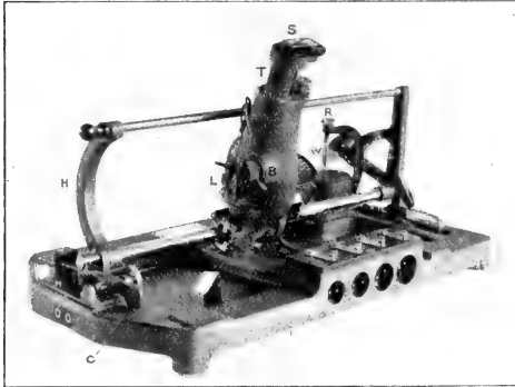
FIG. 2.—The optophone with book-rest removed.
