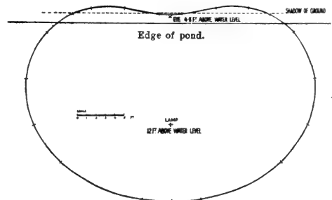
FIG. 3.—Primary bow, position I., as calculated.
