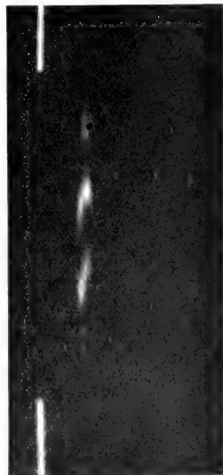
FIG. 6.—A photograph of the chief nebular line in N.G.C. 2392. The slit of the spectroscope was placed along the major axis of the nebula. (W. W. Campbell and J. H. Moore.)
