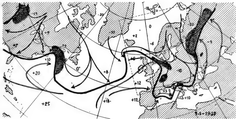
FIG. 2.—Line of demarcation between polar and equatorial air, January 1, 1907.
