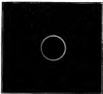
FIG 3—The eclipse just before the mid-phase of annularity.
