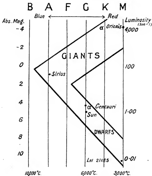
FIG. 2.—Luminosity-temperature diagram.
