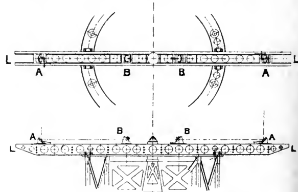
FIG. 2.—Plan and elevation of stellar interferometer.
