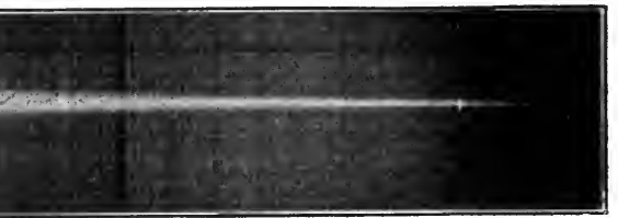
FIG. 2.—The spectrum of the chromosphere, showing, amongst other bright lines, the lines of hydrogen and calcium.
