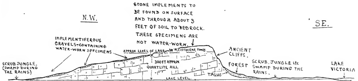
FIG. 1.—Rough diagrammatic sections (not drawn to scale) through Msozi Hill, Sango Bay, Buddu, Uganja.
