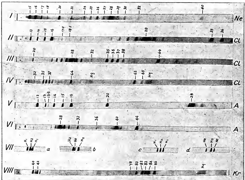
FIG. 2.—Typical mass-spectra.
