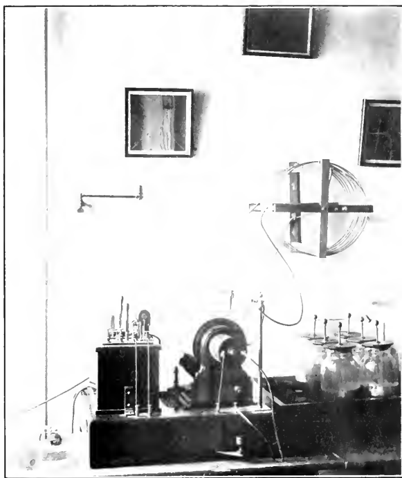
The wireless telegraphy apparatus set up and operated by boys interested in the museum.
