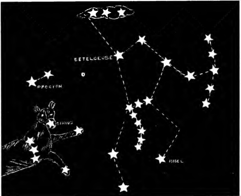
Procyon—The little dog Star. Sirius—The big dog Star.
