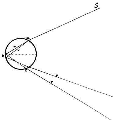
The light-ray is refracted at a , reflected at d , and again refracted at c .
