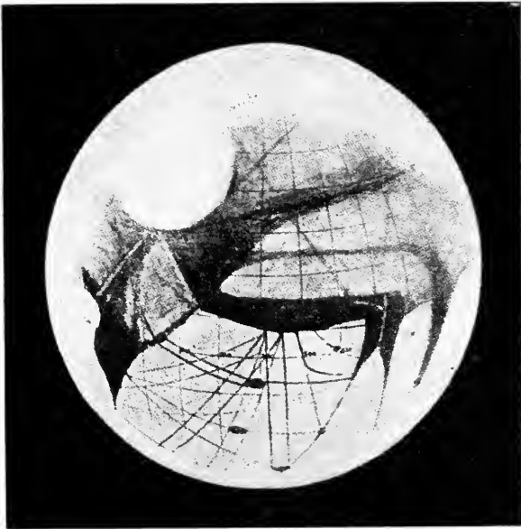
Mars, Showing the Double Canals. After a drawing made at the Lowell Observatory.
