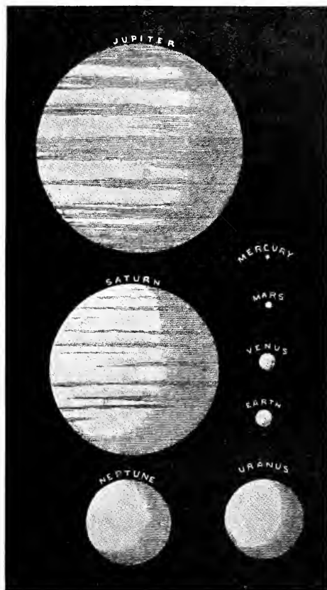
Relative size of the Planets
