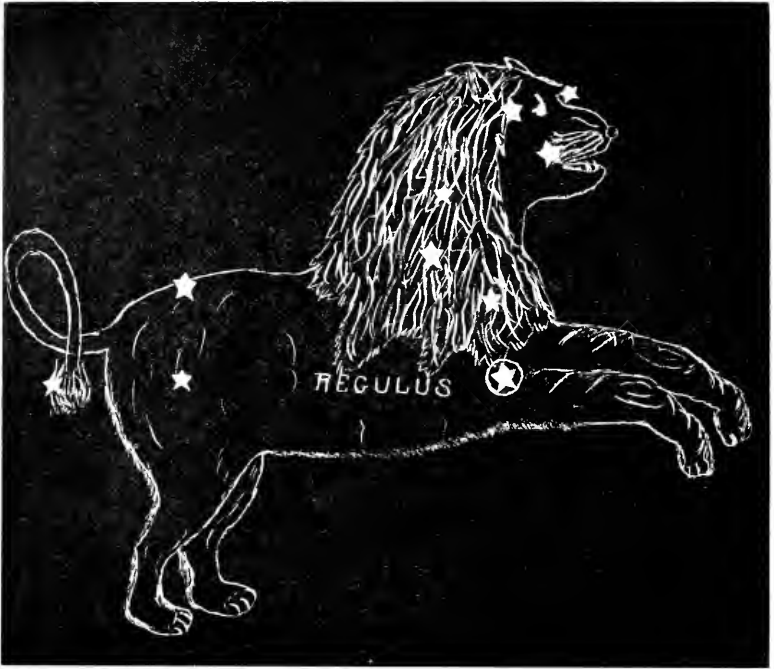
The constellation of Leo—The Lion
