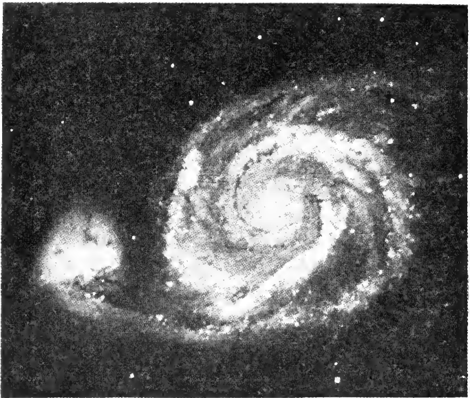
The SUN AND HIS FAMILY may have appeared at the beginning similar to this Spiral Nebula photographed at the Lick Observatory.
