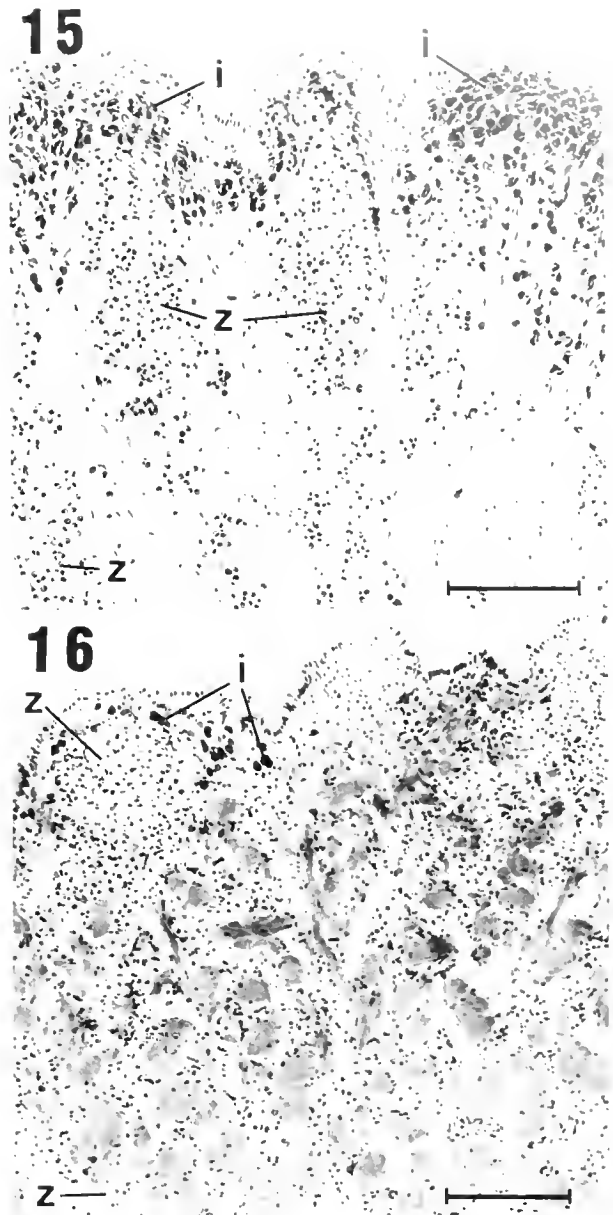
Figures 15, 16. Cross-sections of surface layers of mantle tissues. 15. T. derasa . 16. T. tevoroa . i, iridophores; z, zooxanthellae. Scale bars = 100 micrometers.
