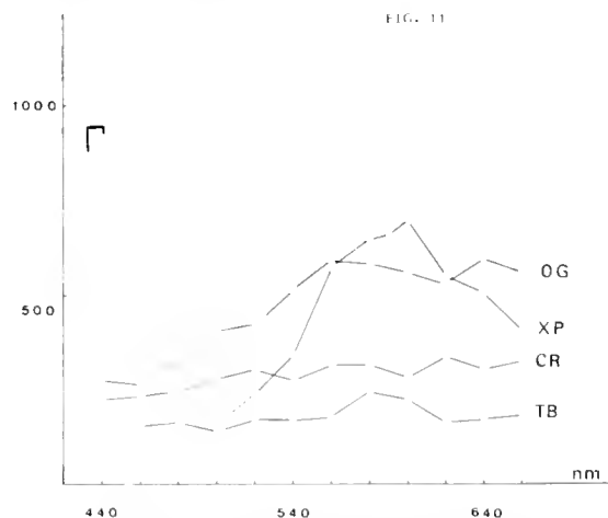
FIG. 11. Curves of the dispersion of the birefringence. \square = optical path differences (nm)
