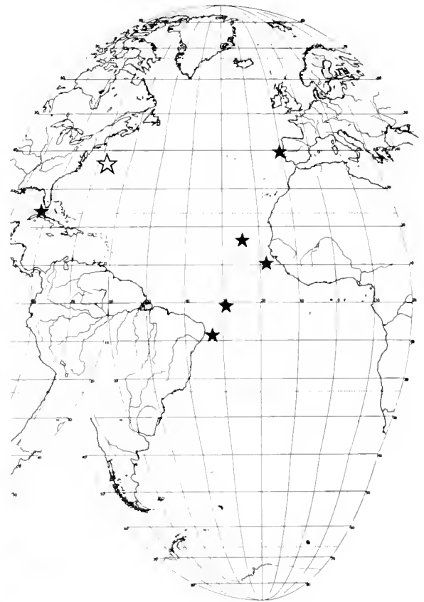
FIG. 4. The distribution of Epitonium nitidum (Verrill and Smith, 1885) in the Atlantic Ocean. Solid stars indicate individual records, and the open star in the western North Atlantic represents a composite of the first nine new records presented in Table 1 and two previous records from Verrill discussed in the text.
