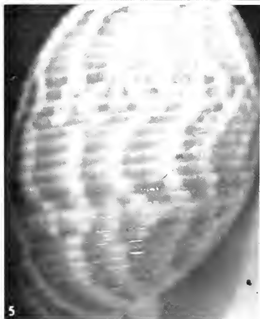
FIG. 4. Acteon eloiseae Abbott, new species. Paratype, details of sculpture and color pattern. X6. FIG. 5. Details of sculpture and color pattern of Acteon flammeus (Gmelin, 1791) from Praia de Chocas, Mozambique. X6. Photos by the author.
