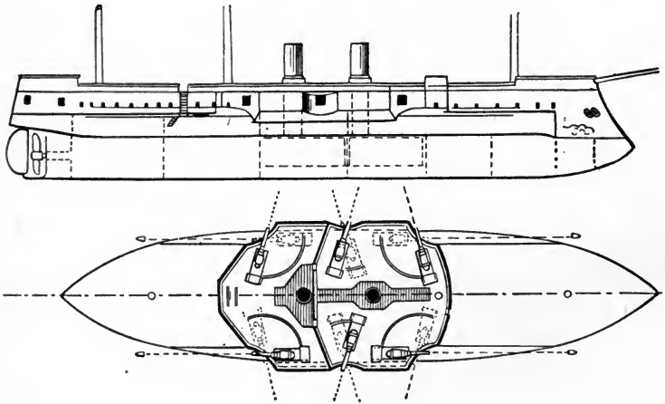
TEGETTHOFF.
