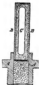
Chemical Fuse.
