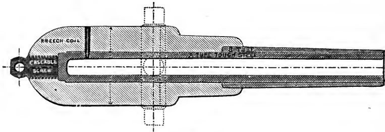
7-inch Mark III.
