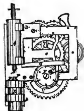
Clockwork Fuse.
