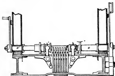
Elswick Compressor.
