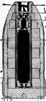
Armstrong Segment Shell.
