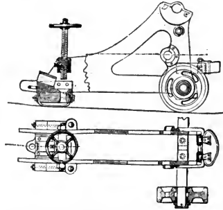
Broadside-Carriage for 8-cm. Boat-Gun.
