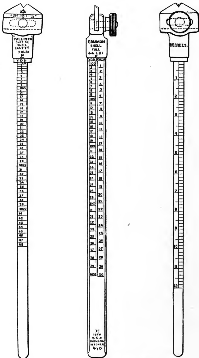
Sliding Leaf Tangent Sight—Muzzle-Loaders.
