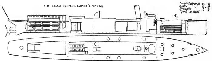
Thornycroft Torpedo-Launch.
