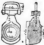
Vent-Piece.
