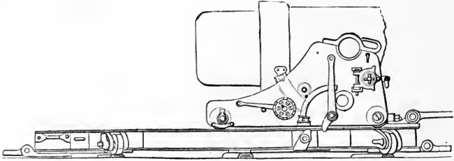
Carriage and Slide for 21-cm. Gun.
