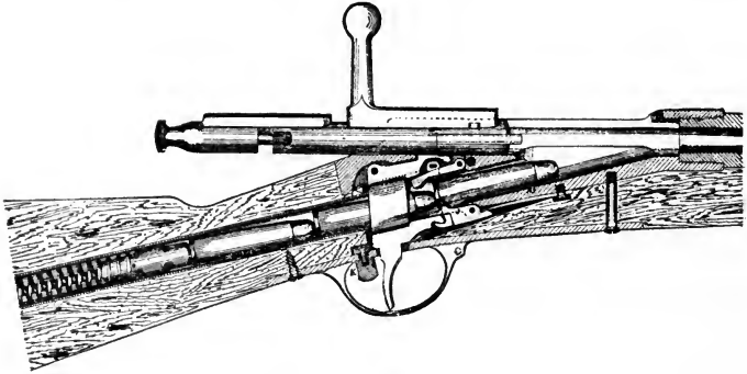
Hotchkiss Magazine.
