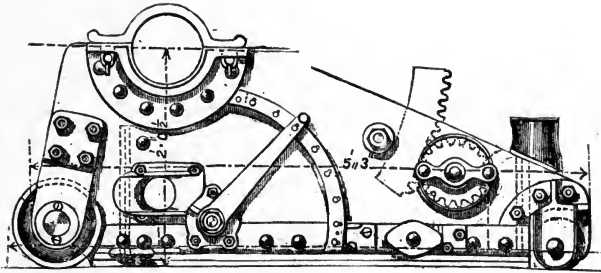
7-inch Carriage.
