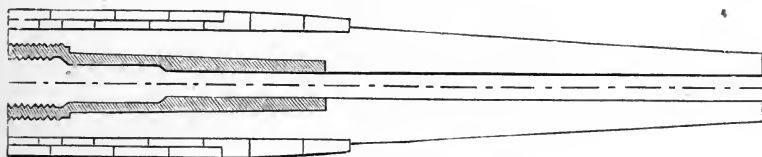
27-cm. French Gun, Model 1870.
