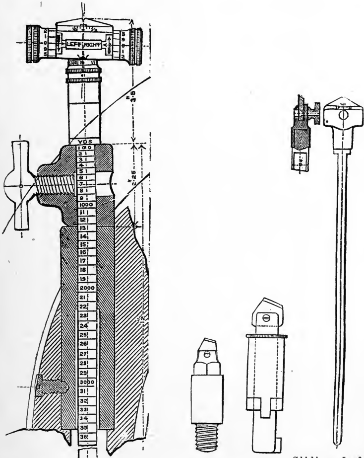
(Screw.) (Drop.) Fore-Sight.
