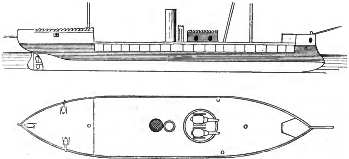
HUASCAR.
