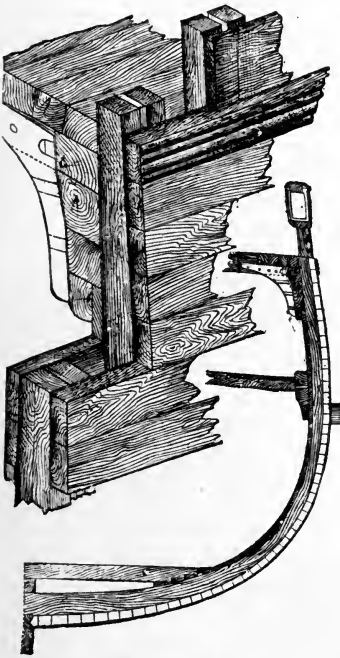
French Corvette La Clocheterie (Wooden System.)
