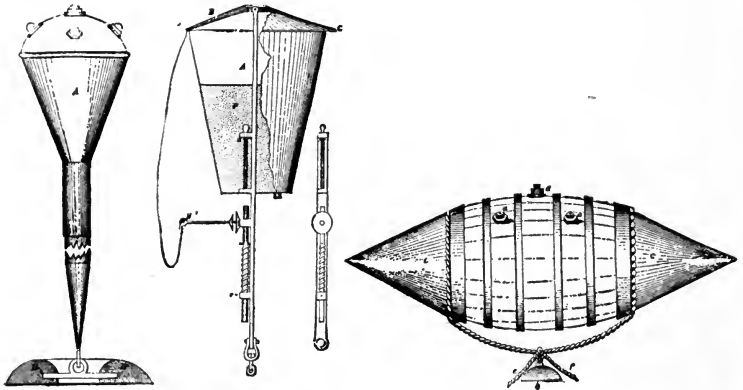
Brooks's Torpedo.
