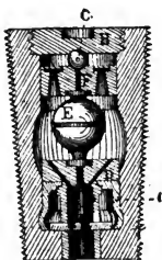
Pettman Percussion-Fuse.
