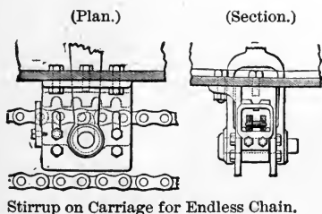
Stirrup on Carriage for Endless Chain.
