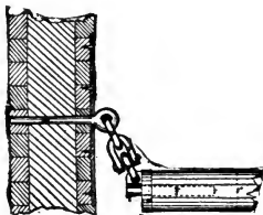
Fitting for Heel of Spar Ship-Torpedo.
