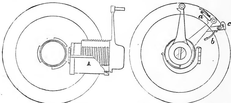
Breech-Block (Gun open).
