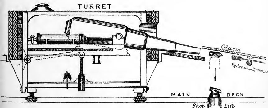
51-ton Gun-Slide and Trunnion Saddles—Hydraulic Loading Arrangements.
