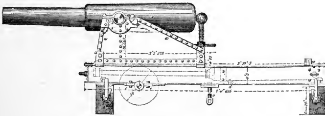
9-pdr. Boat-Carriage.
