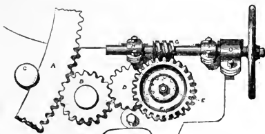
9-inch Elevating-Gear.
