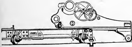
Half-Slide Carriage for 17-cm. Gun.
