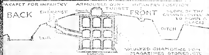
SECTION THROUGH ONE OF THE GUN POSITIONS
