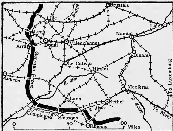
Sketch showing importance of Douai and Valenciennes Junctions in the German Railway Communications on the Western Front.
