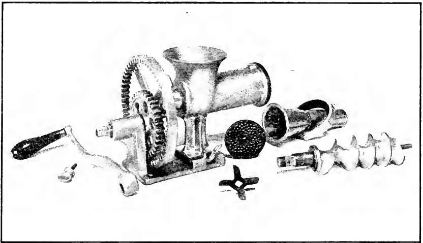
FIG. 8.—Grinding and molding equipment.
