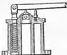
SWANN'S PATENT SAFETY VALVE.
