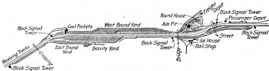
PLAN OF FREIGHT YARD ON ERIE R.R., PORT JERVIS, N. Y.
