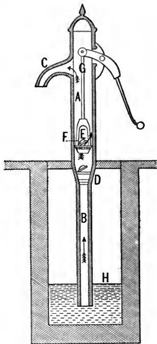
SINGLE SUCTION PUMP.
