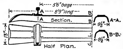
STEEL CROSS-TIE.
