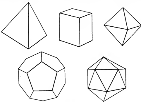
POLYHEDRA.
