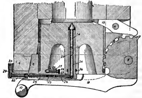
FLETCHER RAPID-FIRE BREECH MECHANISM.—HORIZONTAL SECTION.
