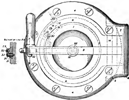
FLETCHER RAPID-FIRE BREECH MECHANISM.—END VIEW.
