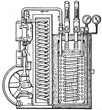
FIG. 4. MARINE TYPE OF CARBONIC-ACID COMPRESSION REFRIGERATING MACHINE.
