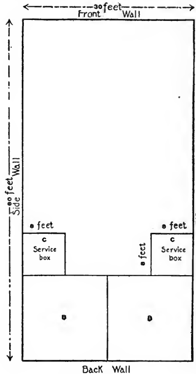
PLAN OF RACQUET COURT.
