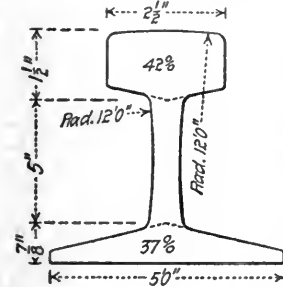
STANDARD AM. SOC. C. E. 80-LB. RAIL.
