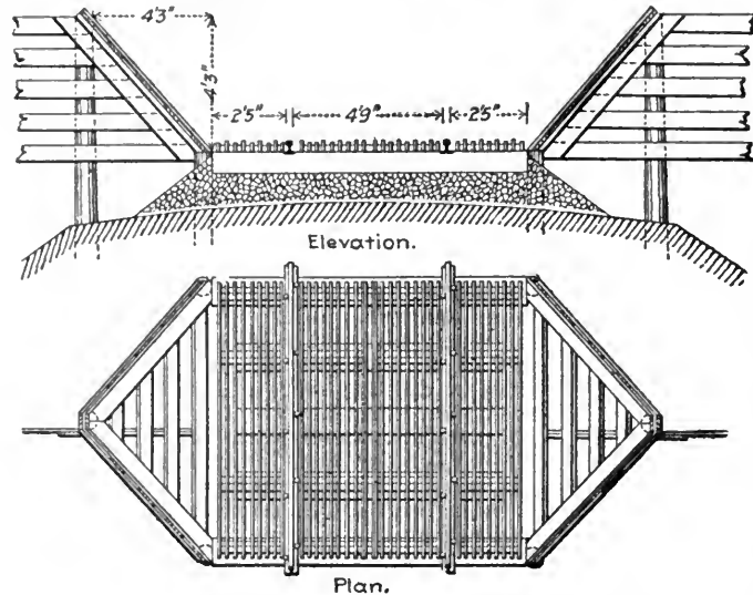
CATTLE GUARD WITH METAL SURFACE.
