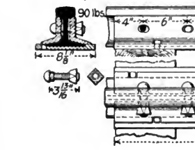
ANGLE-BAR RAIL JOINT.
