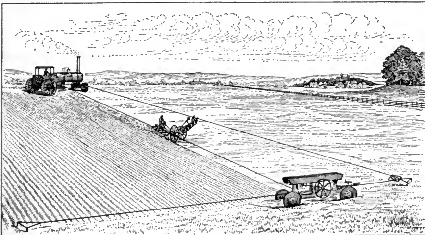
FIG. 8. SINGLE-ENGINE OR ROUND-ABOUT METHOD OF STEAM PLOWING.
