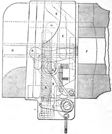
HOTCHKISS RAPID-FIRING GUN.
