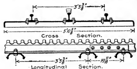
TRACK CONSTRUCTION OF STRUB RACK RAILWAY.
