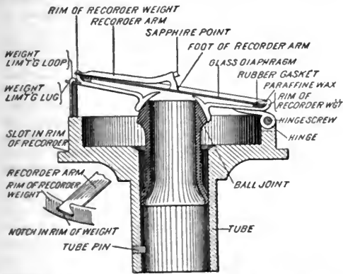
SECTION OF RECORDING APPARATUS OF EDISON PHONOGRAPH.
