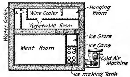
FIG. 5. ARRANGEMENT OF REFRIGERATING PLANT ON LARGE PASSENGER STEAMER.
