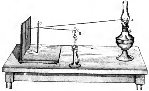
FIG. 3. RUMFORD PHOTOMETER.
