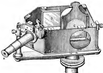
FIG. 6. LUMMER-BRODHUN PHOTOMETER.
