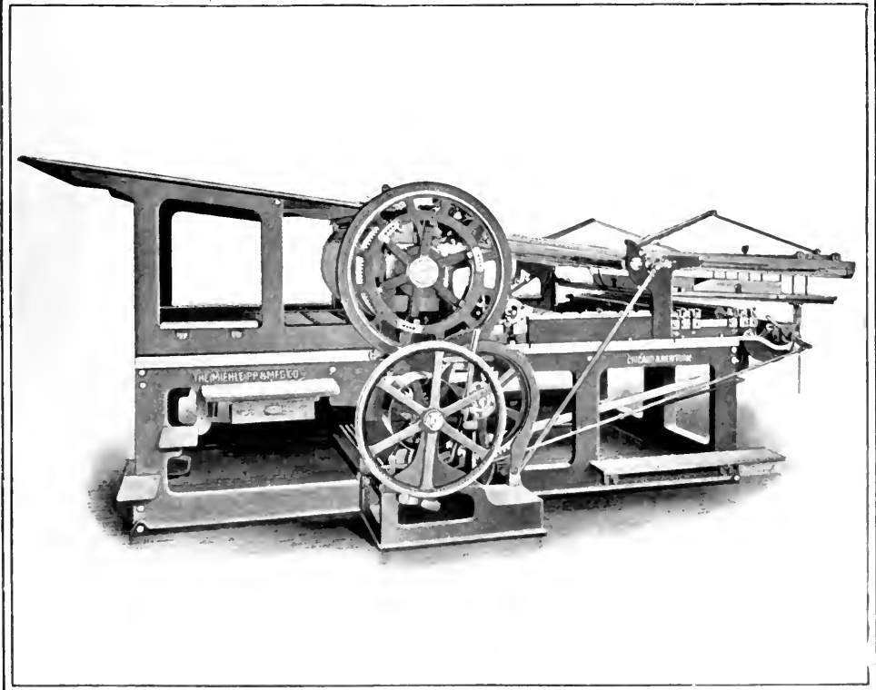
1. HOE ROTARY PERFECTING PERIODICAL AND BOOK PRESS. 2. MIEHLE TWO-REVOLUTION CYLINDER BOOK AND MAGAZINE PRESS.
