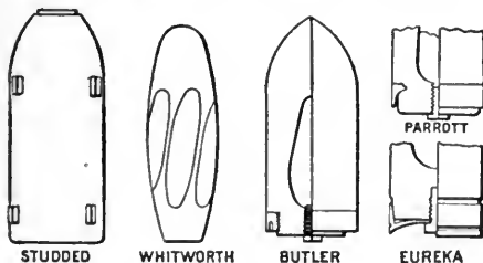
Muzzle-loading projectiles.
