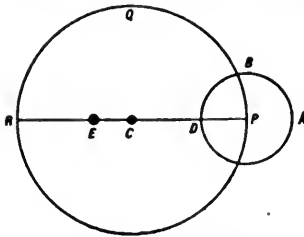
PTOLEMAIC SYSTEM.
