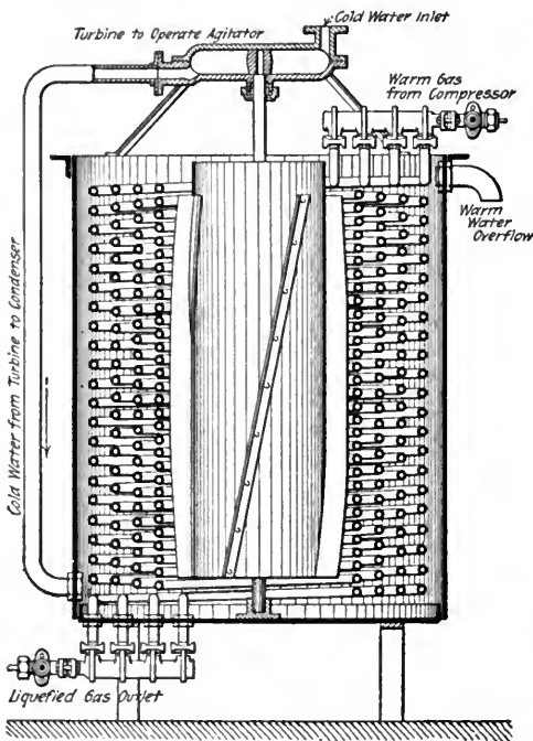
FIG. 3. DIAGRAM SECTION OF CONDENSER FOR LIQUEFYING AMMONIA GAS IN COMPRESSION SYSTEM.
