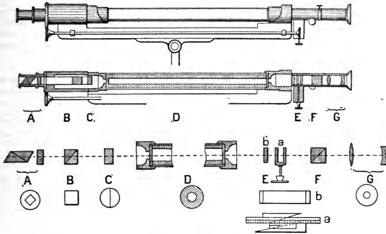
FIG. 5. POLARISCOPE FOR LIQUIDS.
