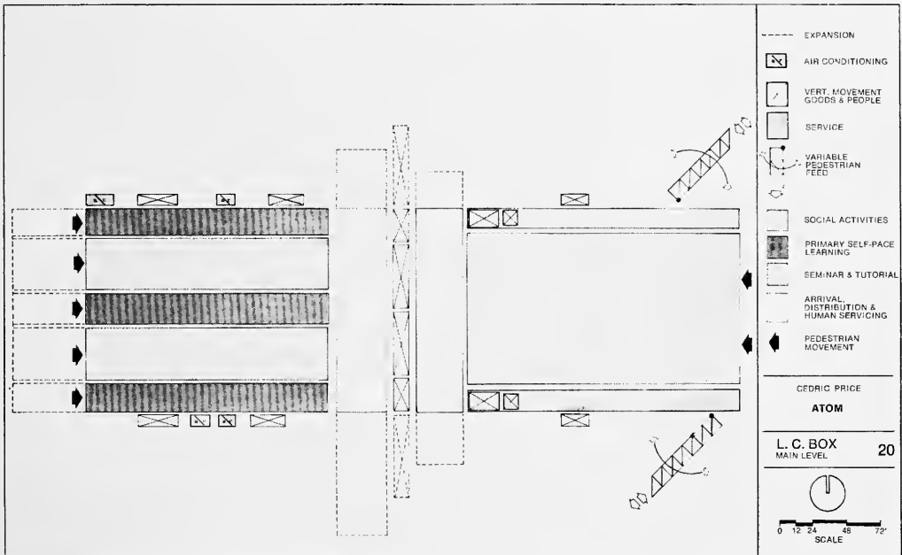
(LC) The Life Conditioner Box straddling the expressway.
