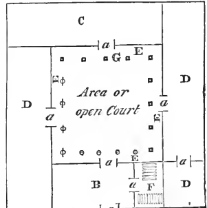
PLAN OF ORIENTAL HOUSE.
