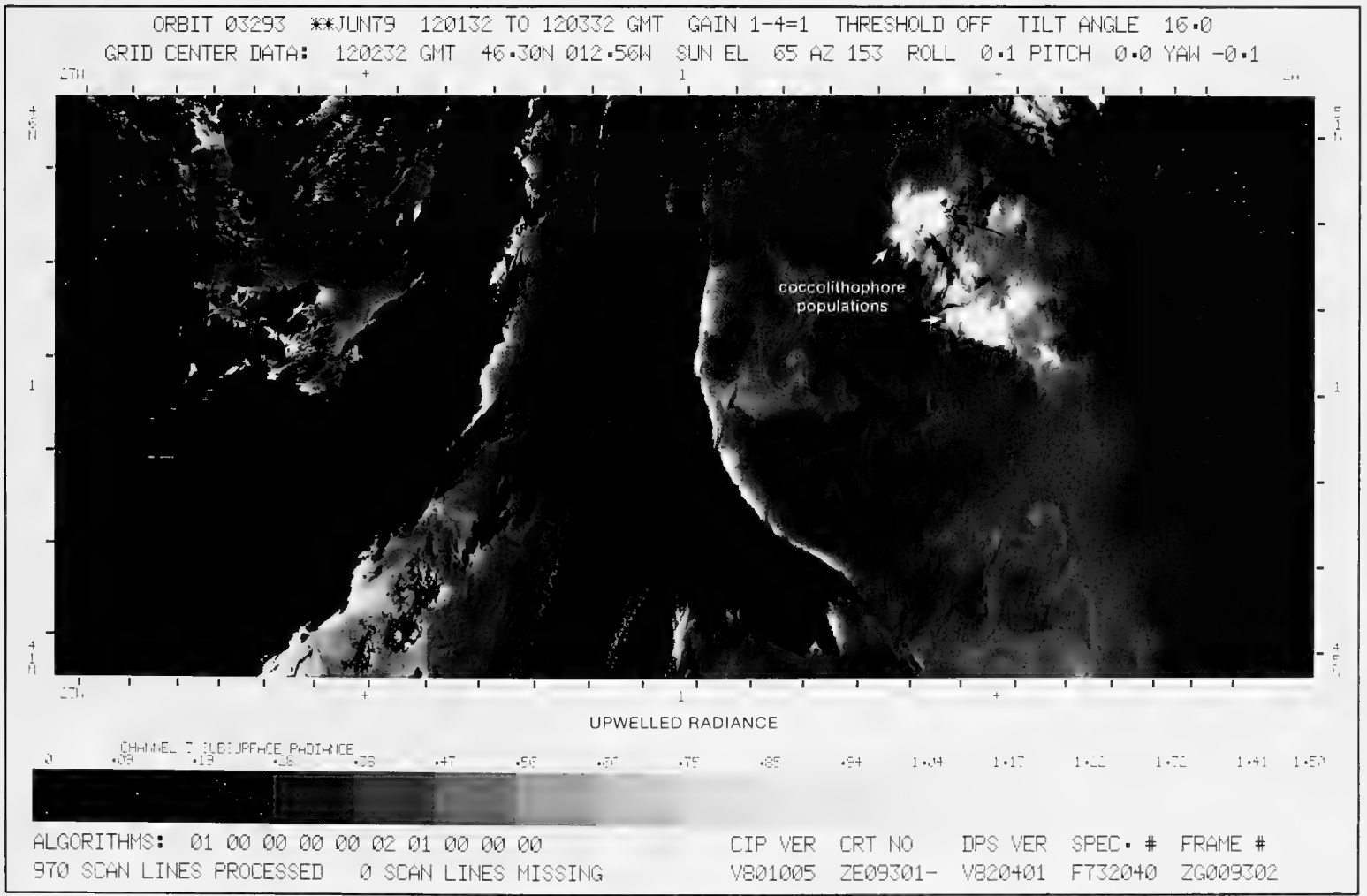
77-2. Nimbus-7. Orbit 3293. 19 June 1979. CZCS Upwelled Radiance Image.
