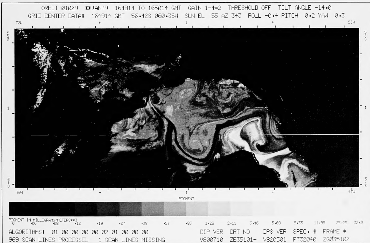
99-2. Nimbus-7. Orbit 1029. 6 January 1979. CZCS Pigment Image.
