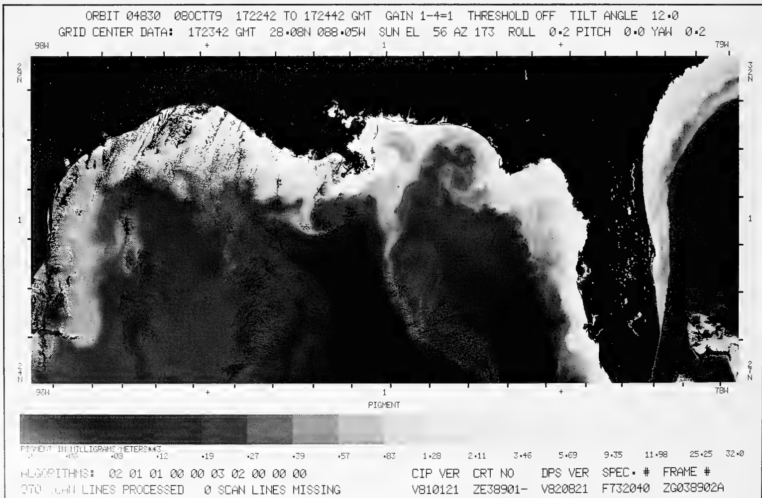
70-2. Nimbus-7. Orbit 4830. 8 October 1979. CZCS Pigment Image.
