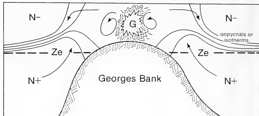
58-1. Schematic of Mixing Process in Shoal Regions.
