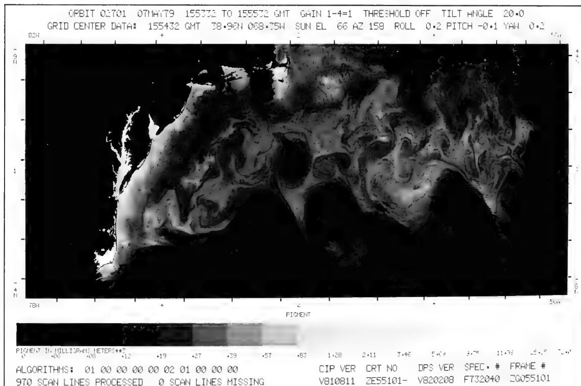
46-2. Nimbus-7, Orbit 2701, 7 May 1979. CZCS Pigment Image.
