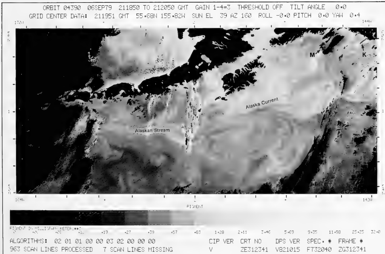
5-2. Nimbus-7. Orbit 4390. 6 September 1979. CZCS Pigment Image. (M-Middleton Is., K-Kayak Is.)
