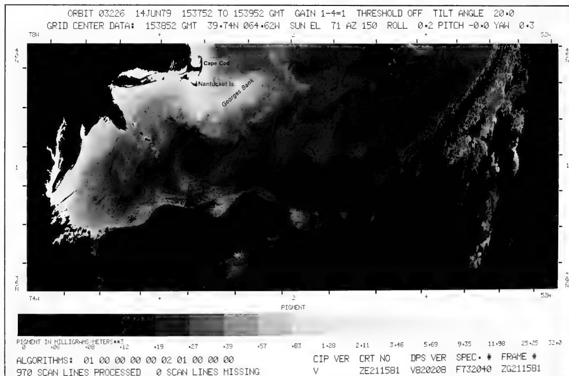
58-2. Nimbus-7. Orbit 3226. 14 June 1979. CZCS Pigment Image.
