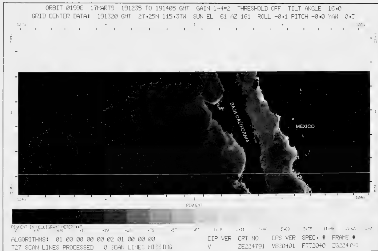
14-1. Nimbus-7, Orbit 1998, 17 March 1979, CZCS Pigment Image.
