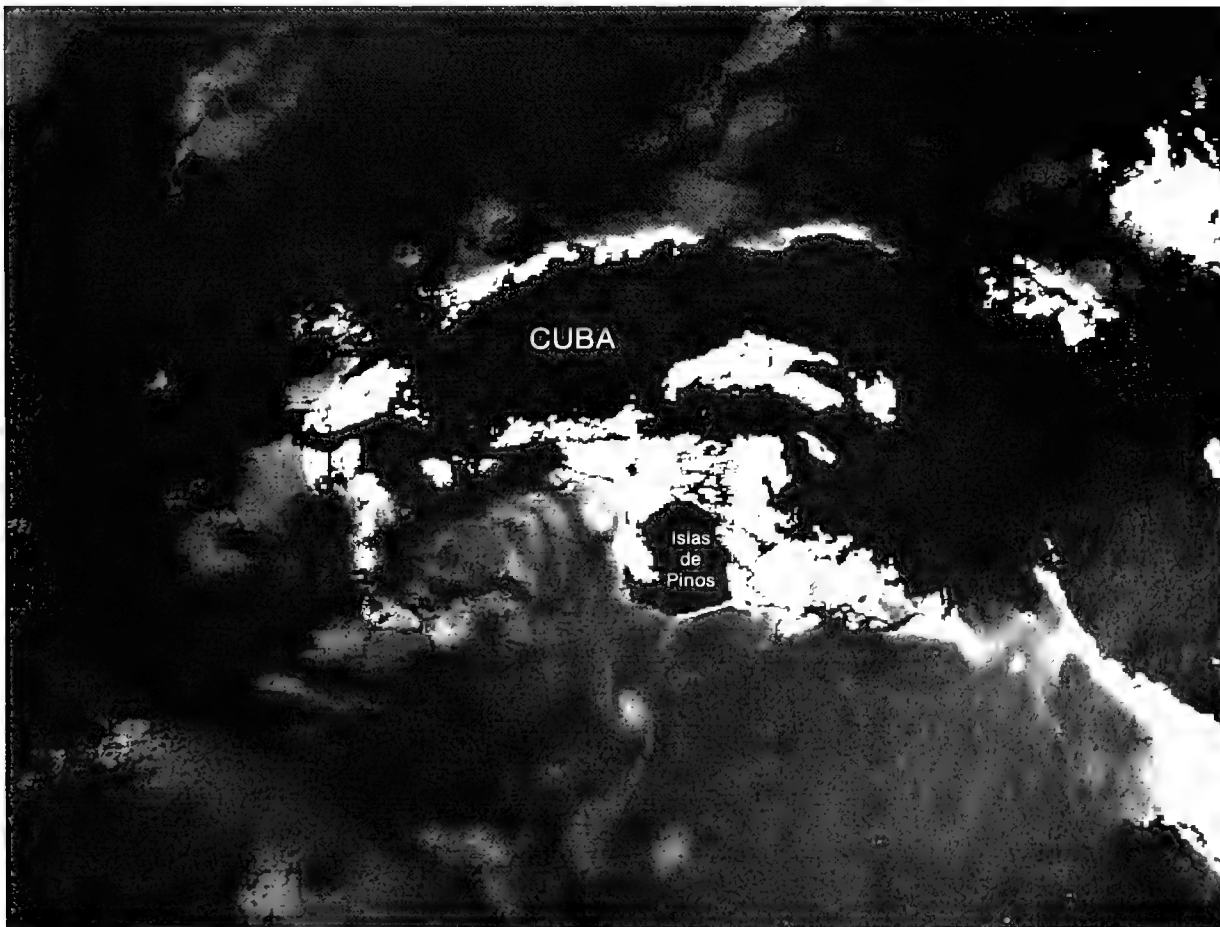
69-2. Enlarged View of Inset B. Nimbus-7. Orbit 4761. 3 October 1979. CZCS Pigment Image.
