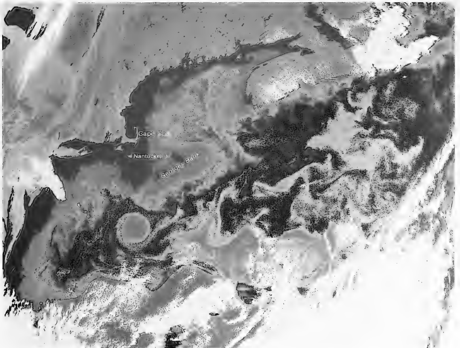
59-1. Nimbus-7. Orbit 3226. 14 June 1979. CZCS False-Color Pigment Image.
