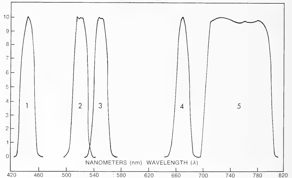
Figure 1. CZCS Spectral Response for Channels 1-5.
