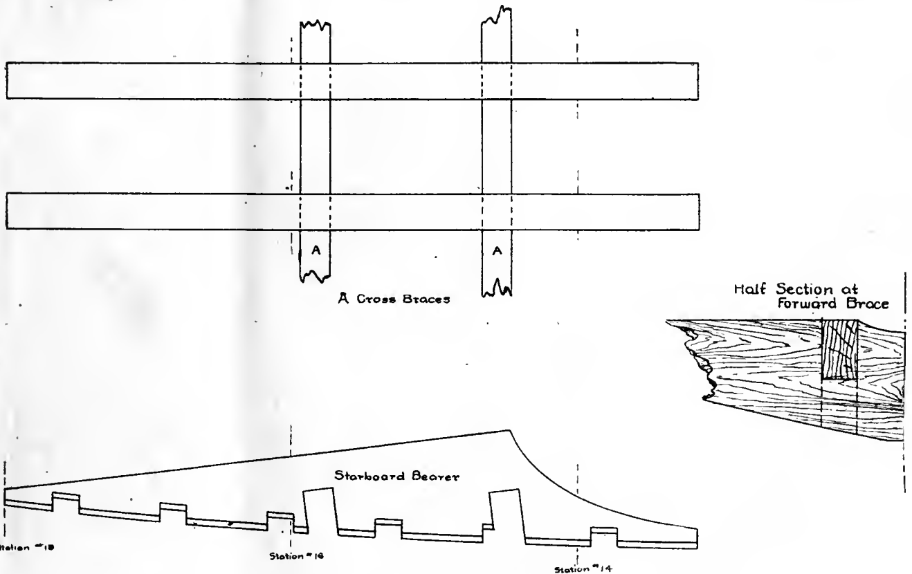
Engine Bed Details
