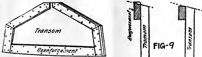
Showing how the reinforcement is fastened around the edge of the transom to give a broader nailing surface for the sides and bottom boards.
