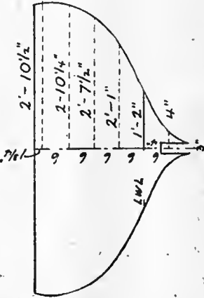
MOLD NO. 6.
