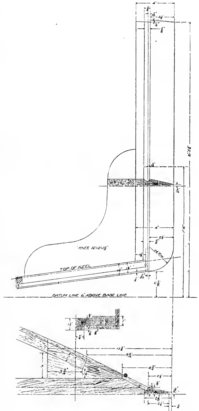
DETAILS OF KEEL, STEM, CHINE AND KNEES. SHOWING THEIR CONNECTION AT BOW
