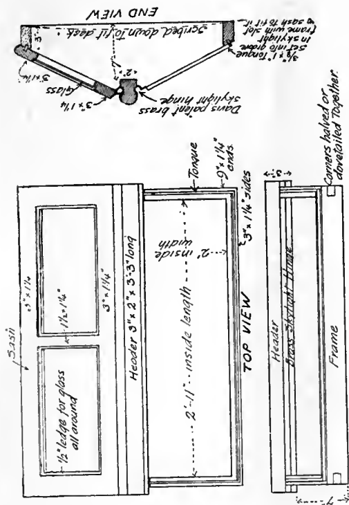
Details of skylight construction for BEAVER
