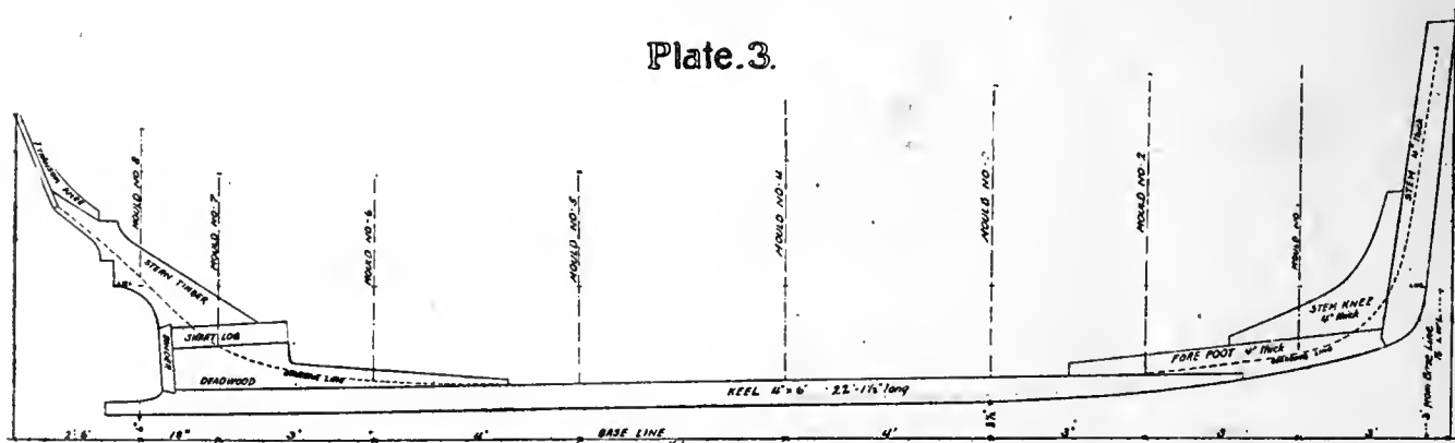
Names of the various pieces that, when all are bolted together, form the backbone of the boat's frame and the location for the various molds.
