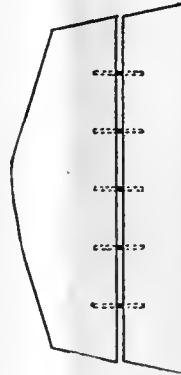
In doweling the two pieces of a transom together, be sure all the dowels are parallel to each other
