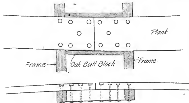
The proper way to butt planking
