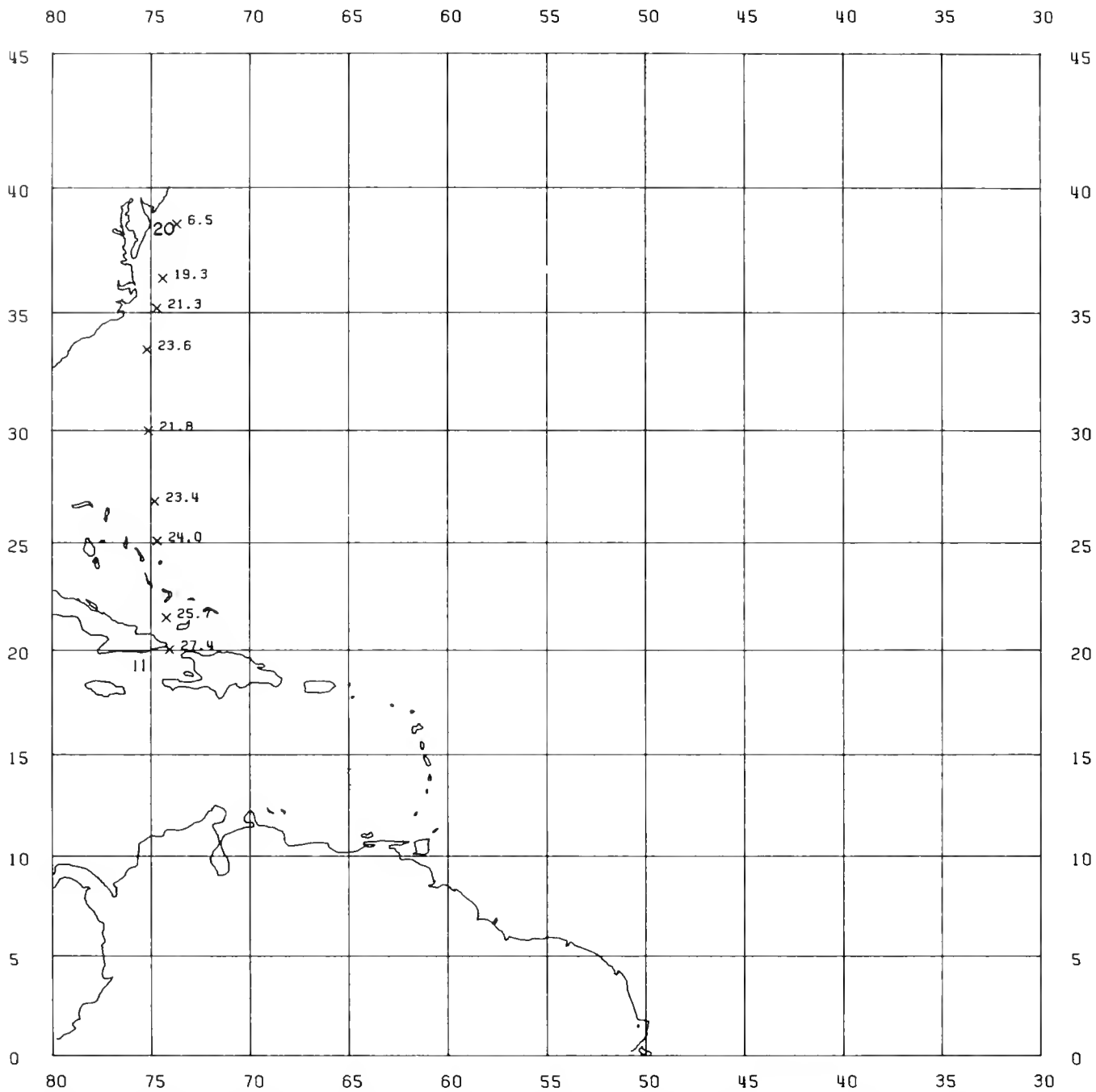
Figure 30.—Sea surface temperature (°C) along the cruise track with the first and last stations numbered. Santa Cruz , 26-29 March 1972.
