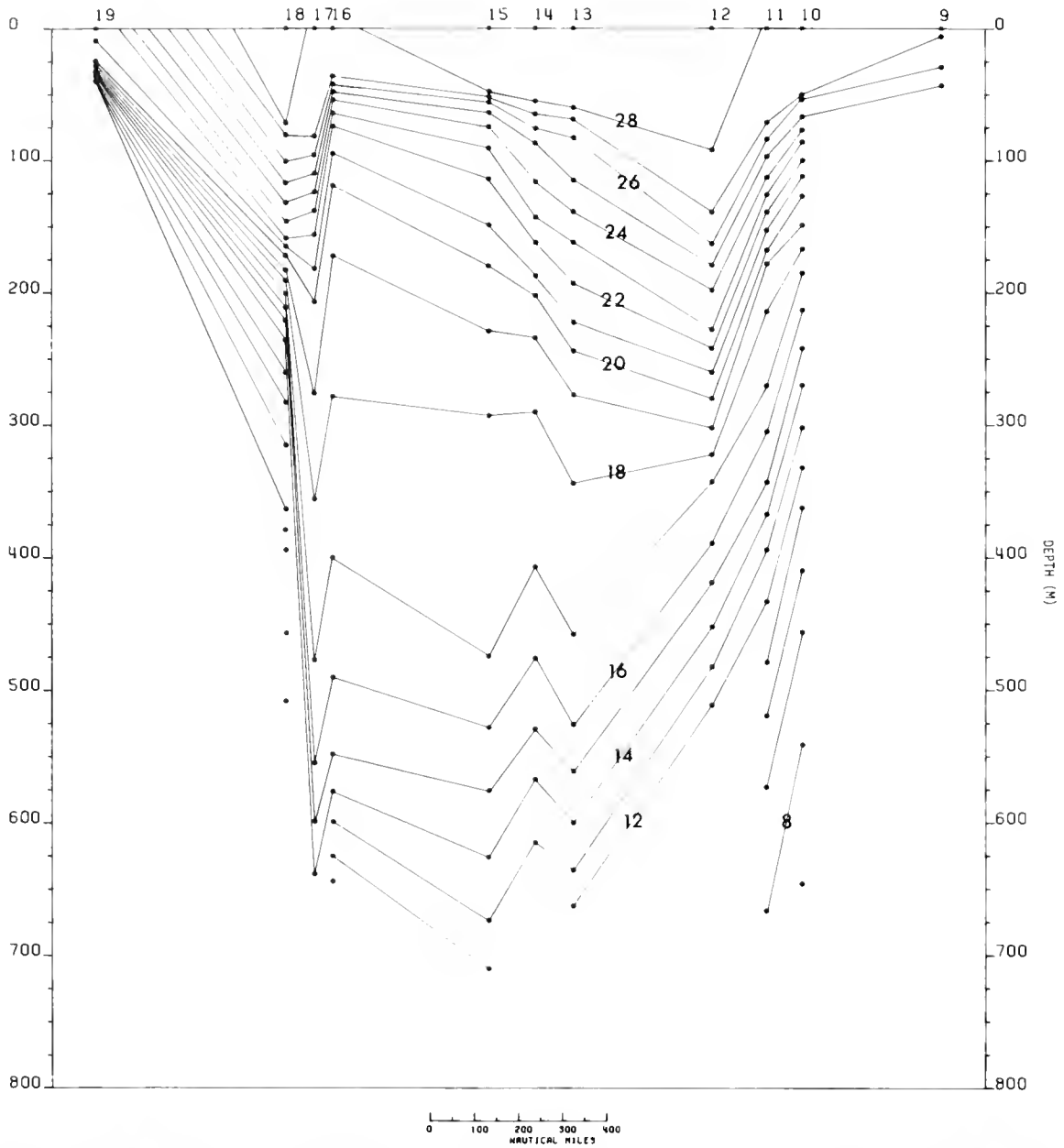
Figure 64.—Vertical distribution of temperature ( ^{\circ}\text{C} ) in the upper 750 m. Contour interval 1^{\circ}\text{C} . Santa Cruz , 2-13 September 1972.
