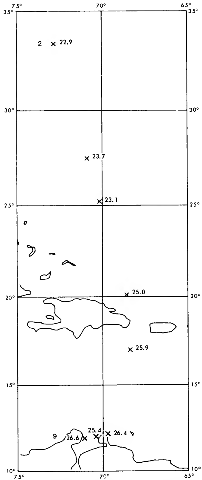
Figure 28.—Sea surface temperature (°C) along the cruise track with the first and last stations numbered. Santa Cruz . 13-25 March 1972.
