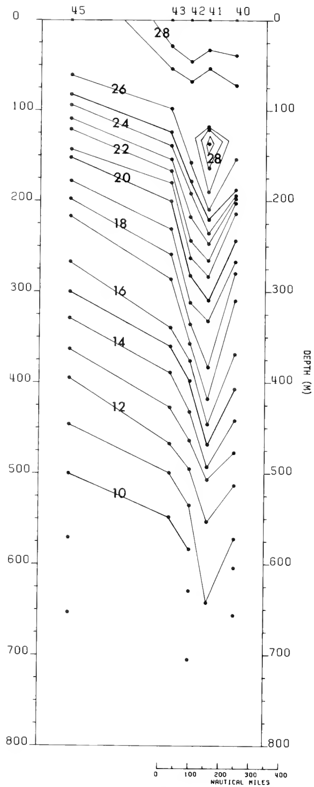
Figure 12.—Vertical distribution of temperature (°C) in the upper 750 m. Contour interval 1°C. Gulf Shipper , 6-7 June 1972.
