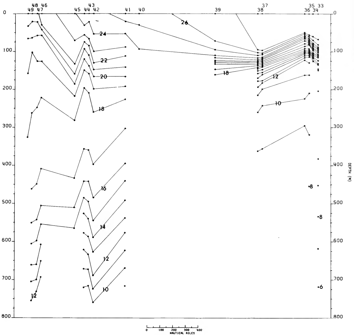
Figure 41. — Vertical distribution of temperature (°C) in the upper 750 m. Contour interval 1°C. Mormac Cape , 20-25 May 1972
