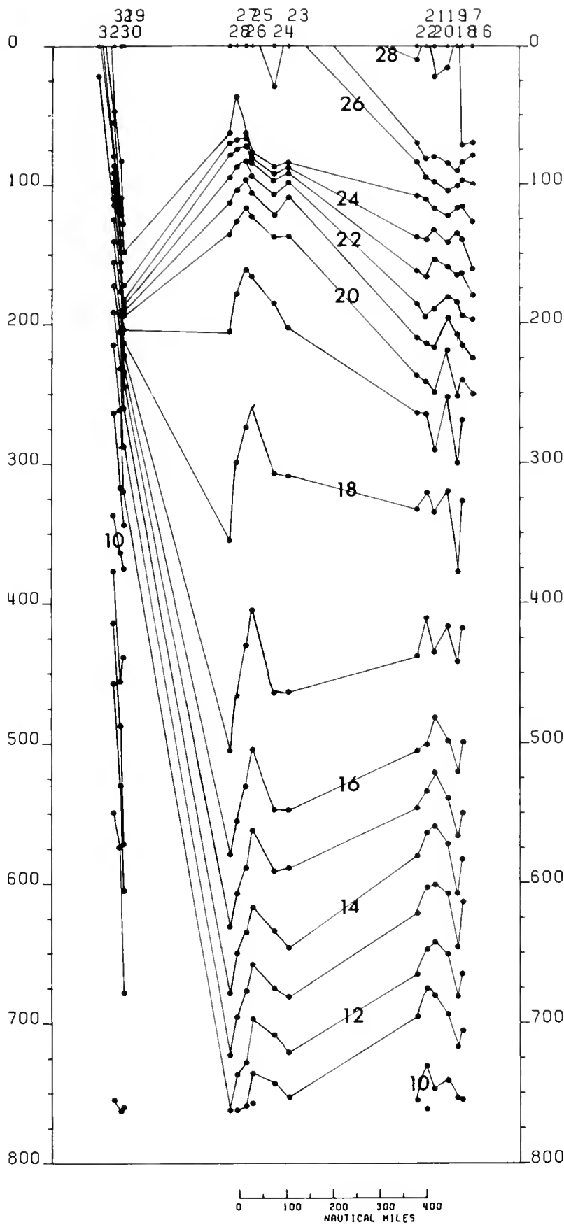
Figure 81.—Vertical distribution of temperature (°C) in the upper 750 m. Contour interval 1°C. Santa Cruz, 3-5 November 1972
