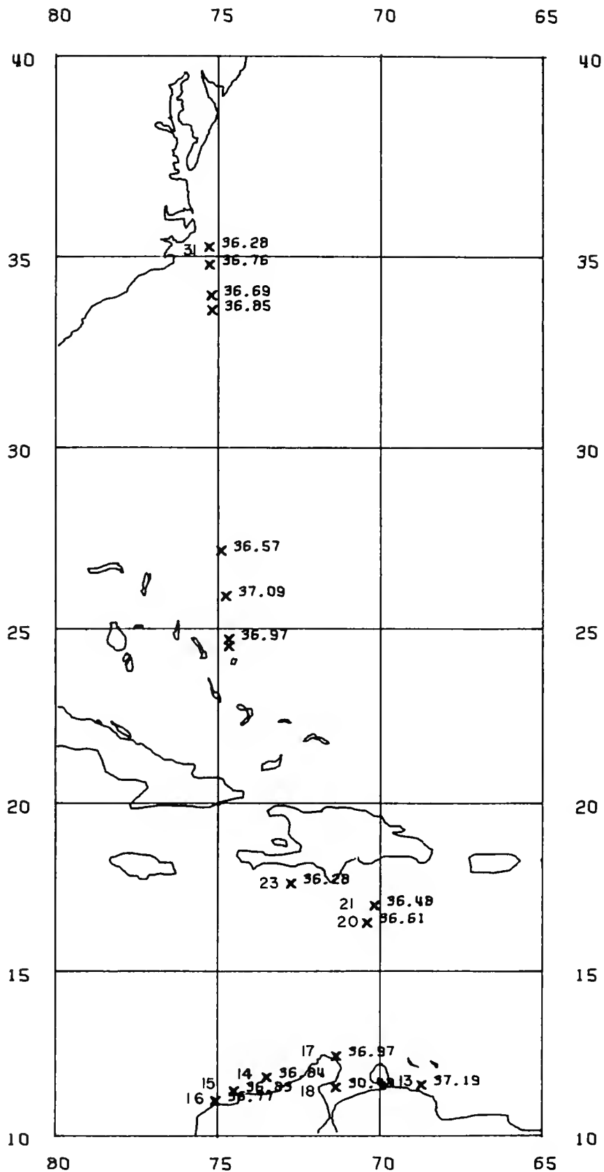
Figure 46.—Sea surface salinities (‰) along the cruise track with the first and last stations numbered. Santa Cruz, 8-18 June 1972.
