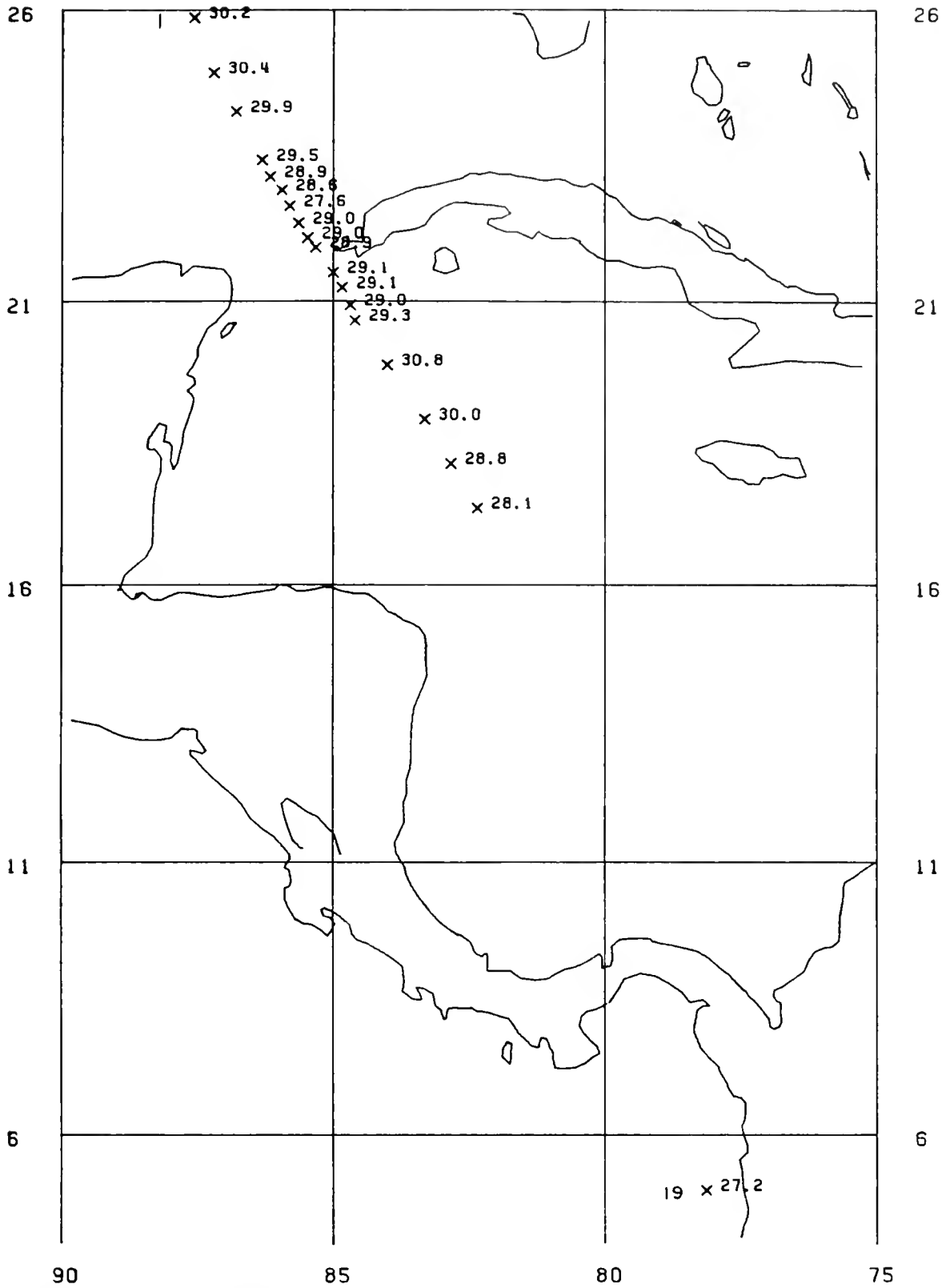
Figure 13.—Sea surface temperature (°C) along the cruise track with the first and last stations numbered. Gulf Shipper , 21-28 August 1972.
