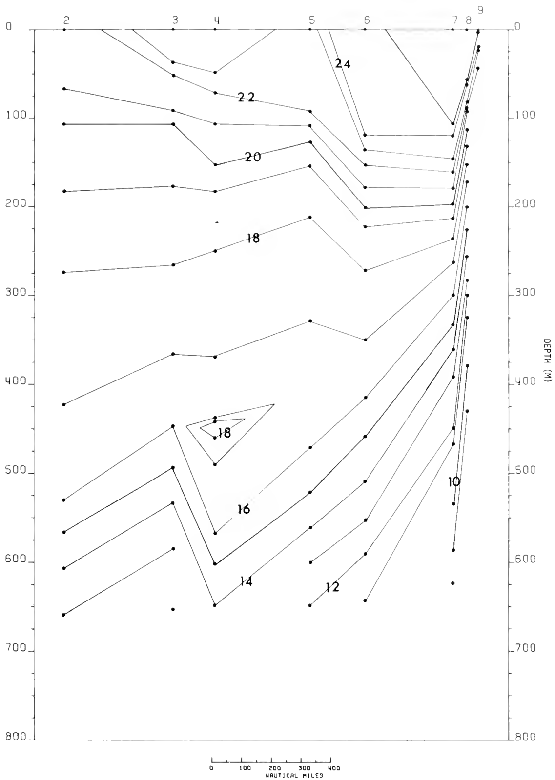
Figure 29. — Vertical distribution of temperature (°C) in the upper 750 m. Contour interval 1°C. Santa Cruz, 13-25 March 1972.
