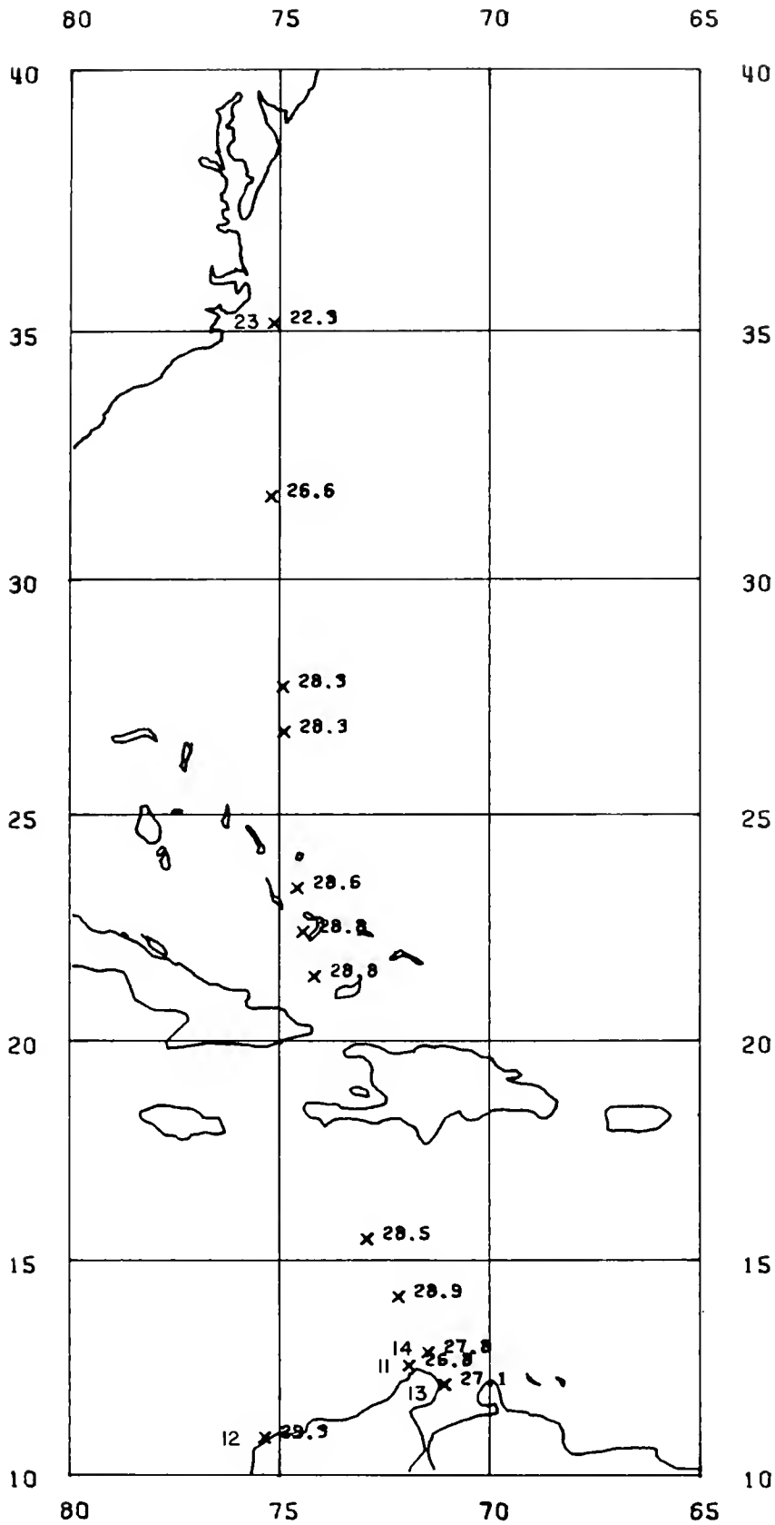
Figure 68.—Sea surface temperature (°C) along the cruise track with the first and last stations numbered. Santa Cruz, 30 September-9 October 1972.
