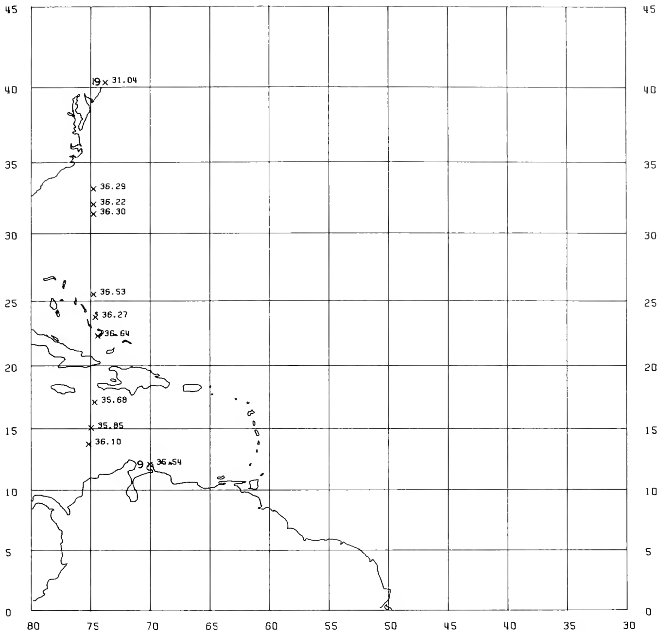
Figure 63.—Sea surface salinities (‰) along the cruise track with the first and last stations numbered. Santa Cruz , 2-13 September 1972.
