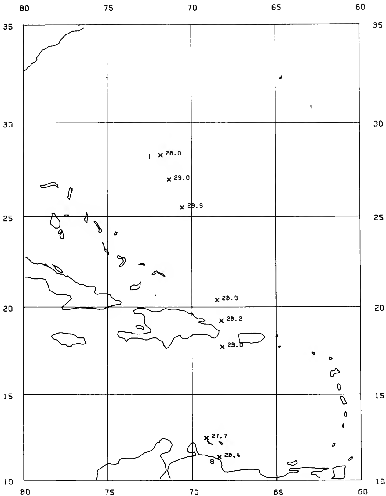
Figure 59.—Sea surface temperature (°C) along the cruise track with the first and last stations numbered. Santa Cruz , 21 August-1 September 1972.
