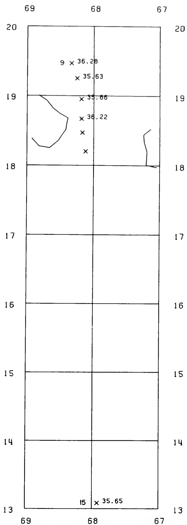
Figure 77.—Sea surface salinities (‰) along the cruise track with the first and last stations numbered. Santa Cruz , 15-18 October 1972.
