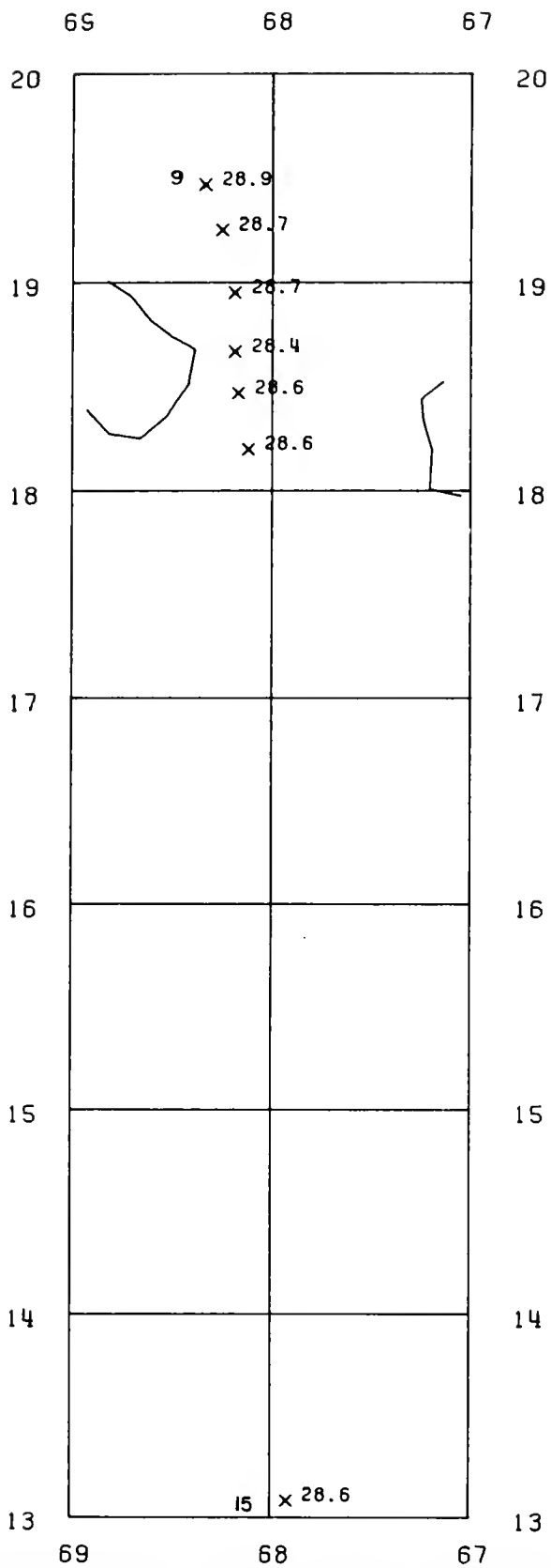
Figure 76.—Sea surface temperature (°C) along the cruise track with the first and last stations numbered. Santa Cruz , 15-18 October 1972.
