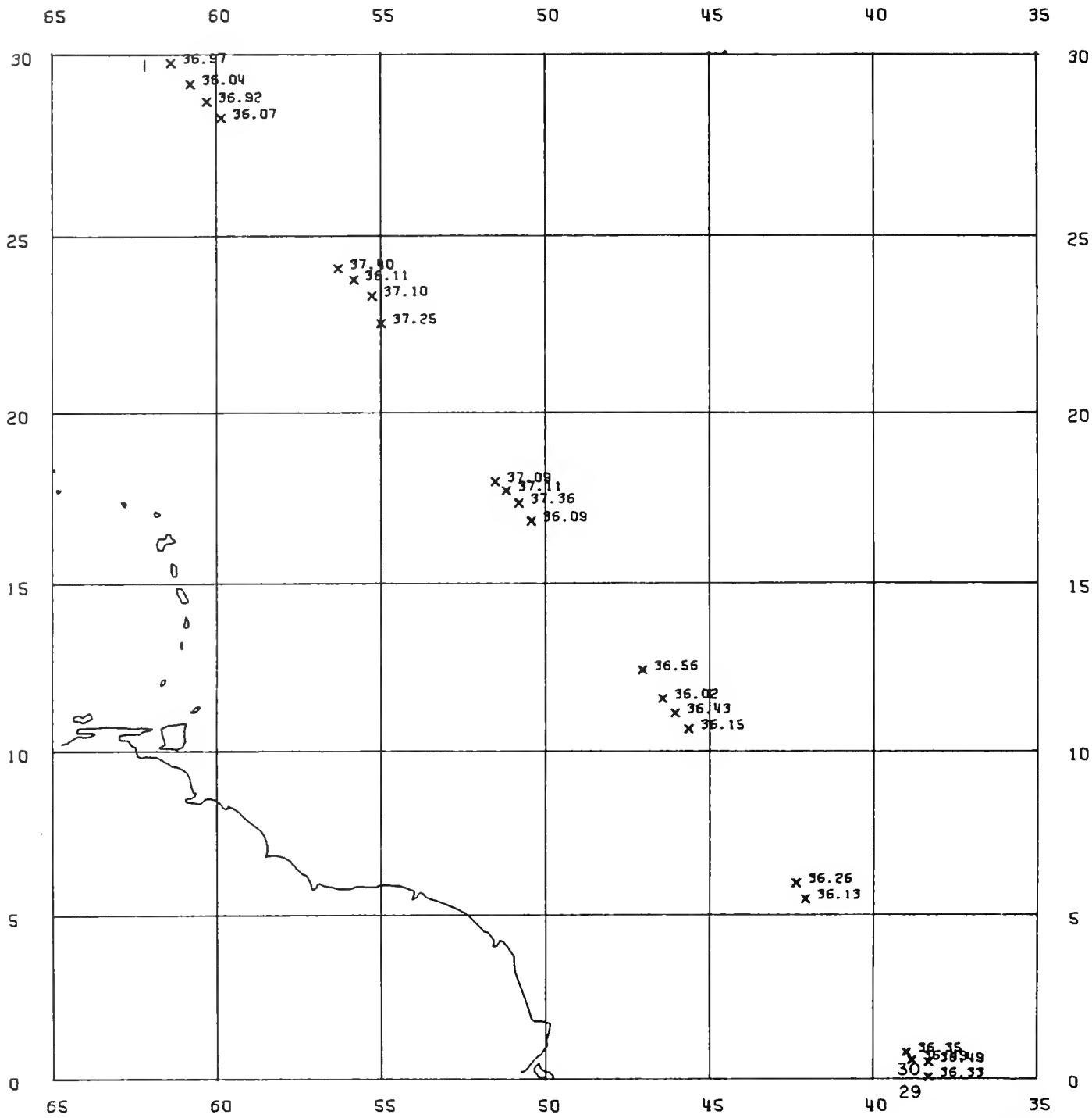
Figure 20.—Sea surface salinities (‰) along the cruise track with the first and last stations numbered. Mormac Trade , 27 January - 1 February 1972.
