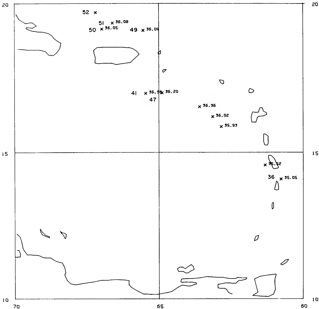
Figure 26.—Sea surface salinities (‰) along the cruise track with the first and last stations numbered. Bay State , 19-23 February 1972.
