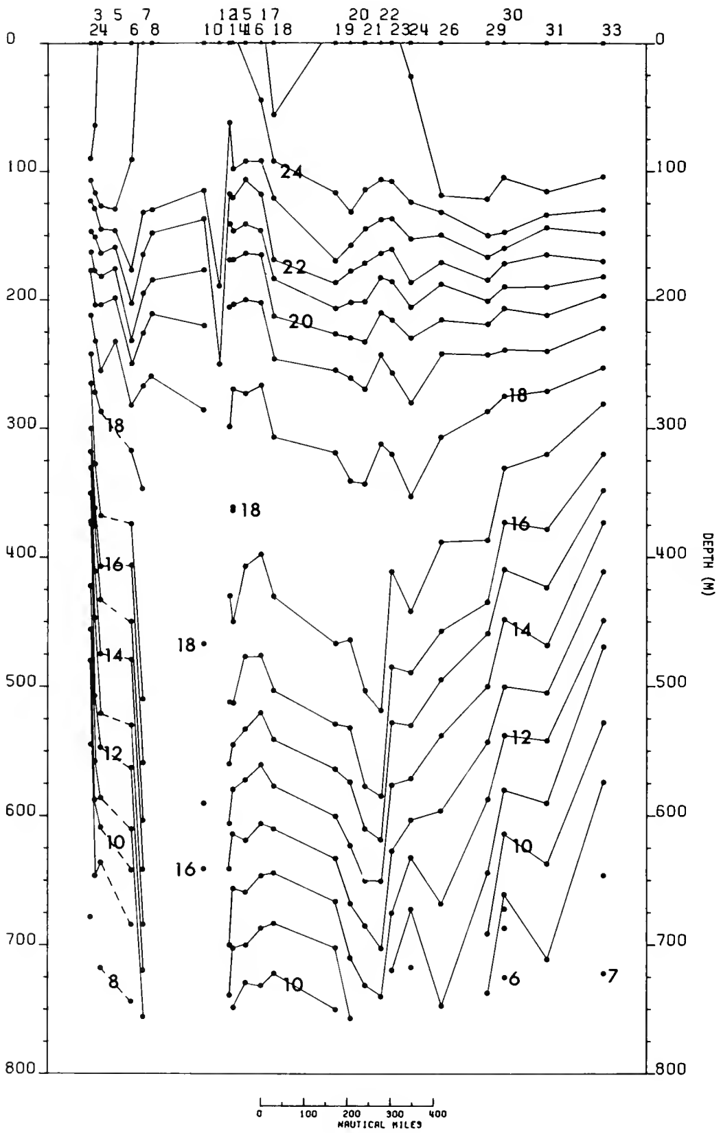
Figure 24.—Vertical distribution of temperature (°C) in the upper 750 m. Contour interval 1°C. Bay State, 10-14 February 1972.
