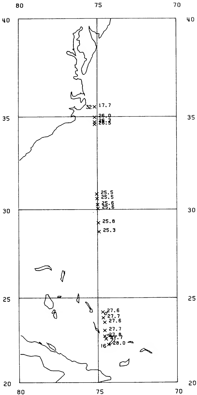
Figure 79.—Sea surface temperature (°C) along the cruise track with the first and last stations numbered. Santa Cruz, 3-5 November 1972.
