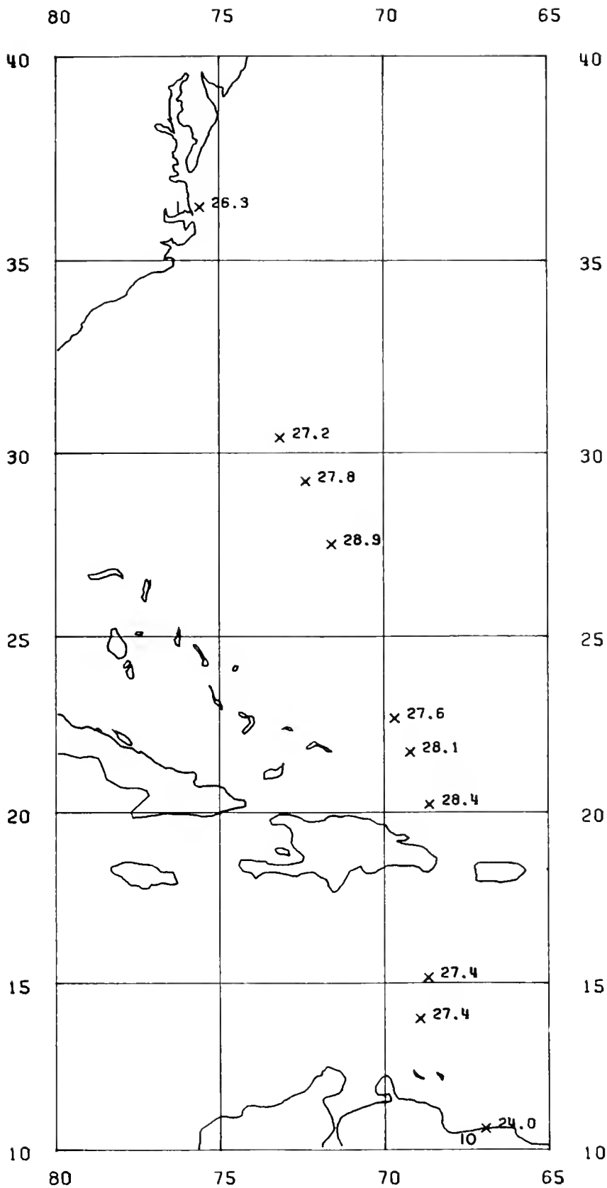
Figure 53.—Sea surface temperature (°C) along the cruise track with the first and last stations numbered. Santa Cruz , 25-31 July 1972.
