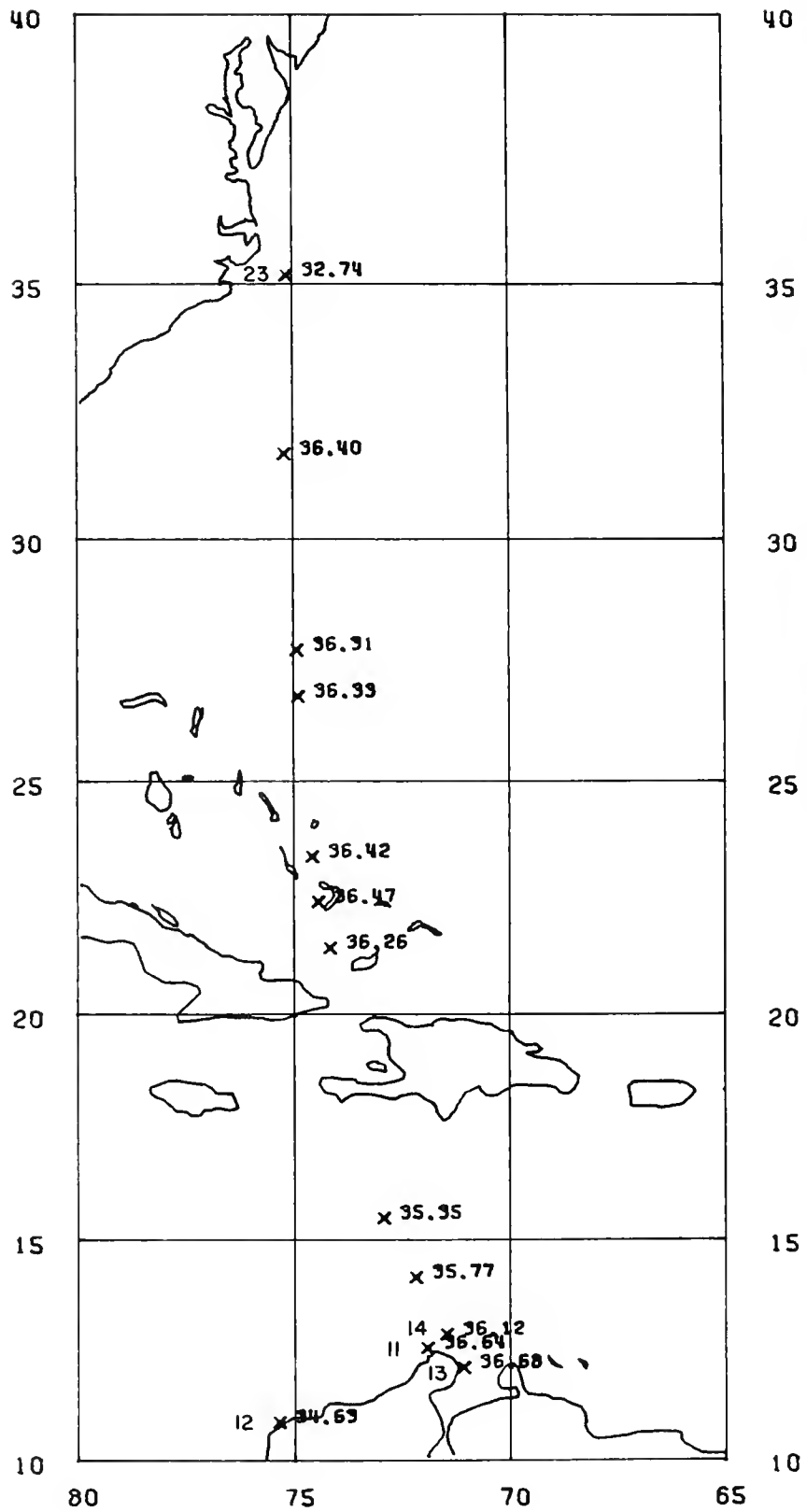
Figure 69.—Sea surface salinities (‰) along the cruise track with the first and last stations numbered. Santa Cruz, 30 September-9 October 1972.
