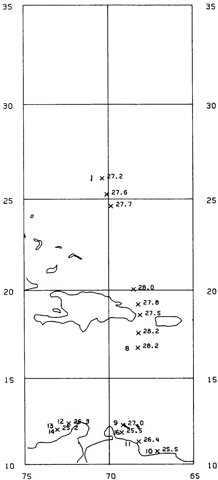
Figure 48. — Sea surface temperature (°C) along the cruise track with the first and last stations numbered. Santa Cruz, 28 June-14 July 1972.
