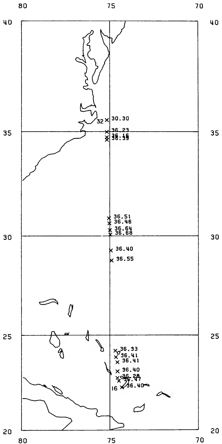
Figure 80.—Sea surface salinities (‰) along the cruise track with the first and last stations numbered. Santa Cruz, 3-5 November 1972.
