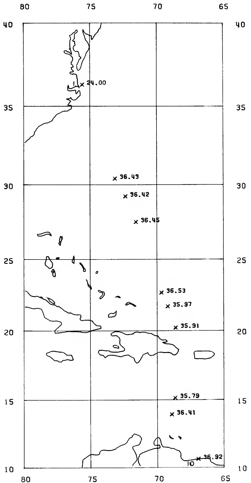
Figure 54.—Sea surface salinities (‰) along the cruise track with the first and last stations numbered. Santa Cruz, 25-31 July 1972.
