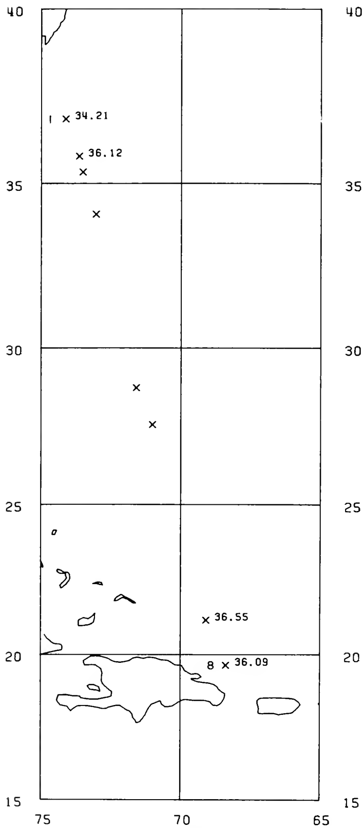
Figure 75.—Sea surface salinities (‰) along the cruise track with the first and last stations numbered. Santa Cruz , 15-18 October 1972.
