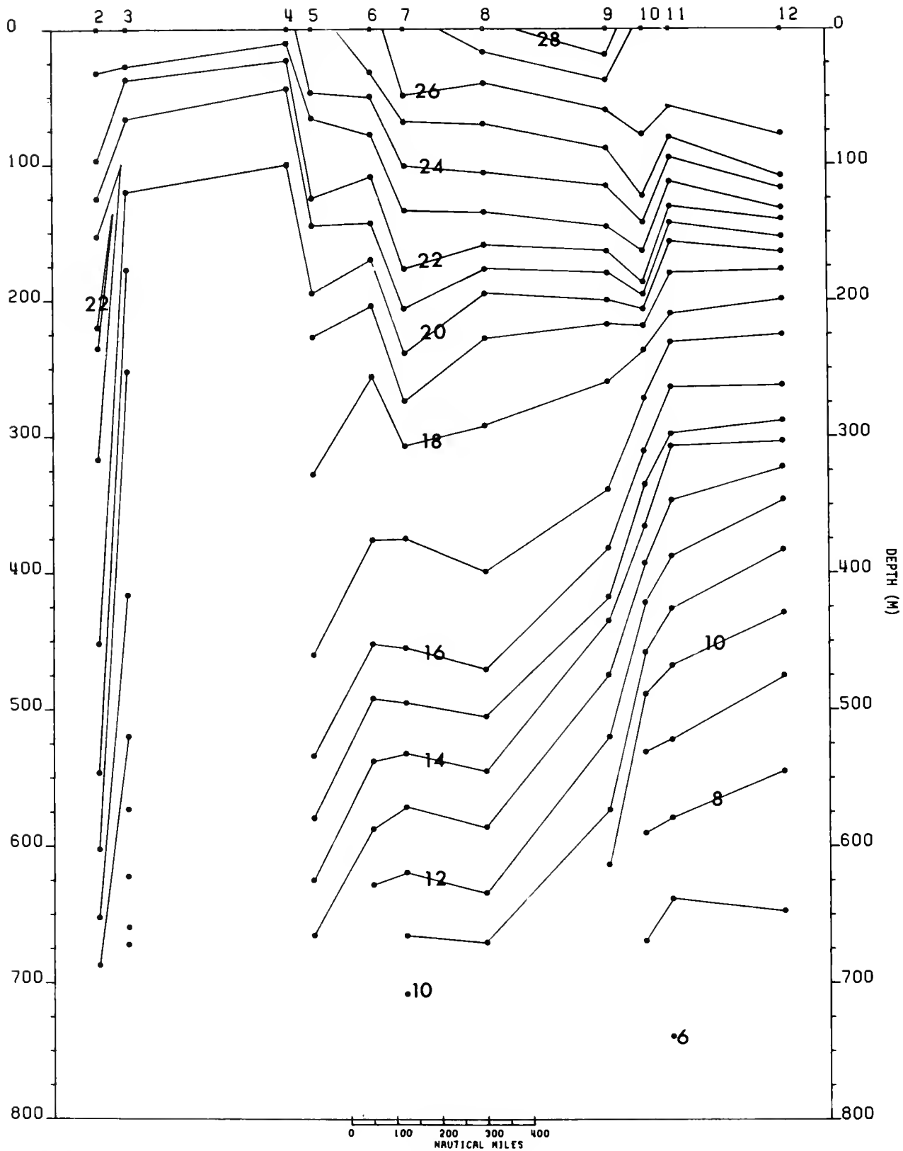
Figure 44.—Vertical distribution of temperature (°C) in the upper 750 m. Contour interval 1°C. Santa Cruz, 29 May-8 June 1972.
