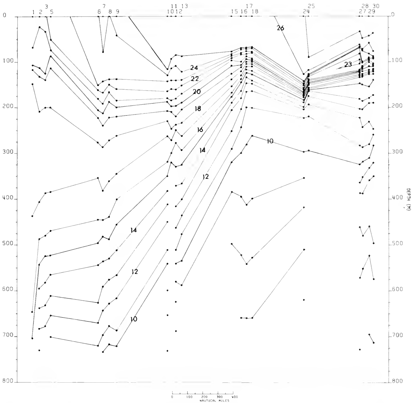
Figure 21.—Vertical distribution of temperature (°C) in the upper 750 m. Contour interval 1°C. Mormac Trade , 27 January-1 February 1972.
