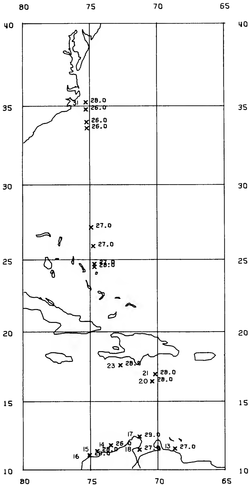
Figure 45.—Sea surface temperature (°C) along the cruise track with the first and last stations numbered. Santa Cruz, 8-18 June 1972.
