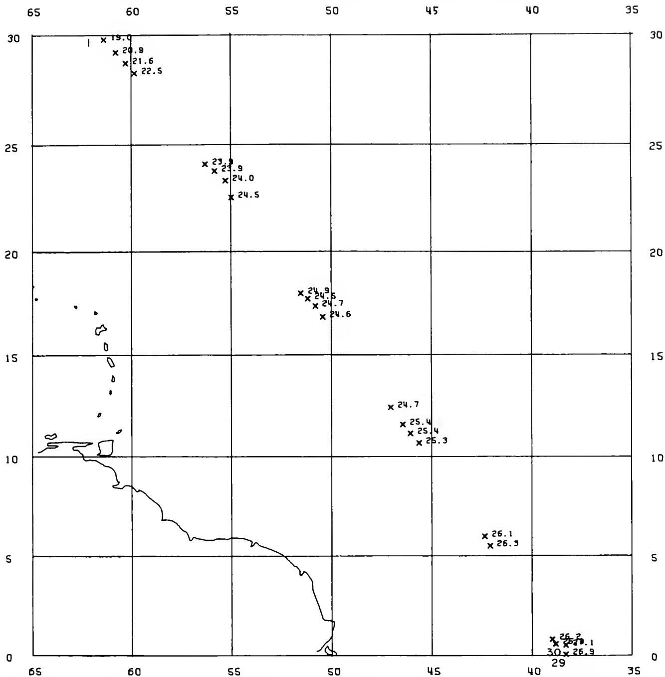
Figure 19.—Sea surface temperature (°C) along the cruise track with the first and last stations numbered. Mormac Trade , 27 January-1 February 1972.
