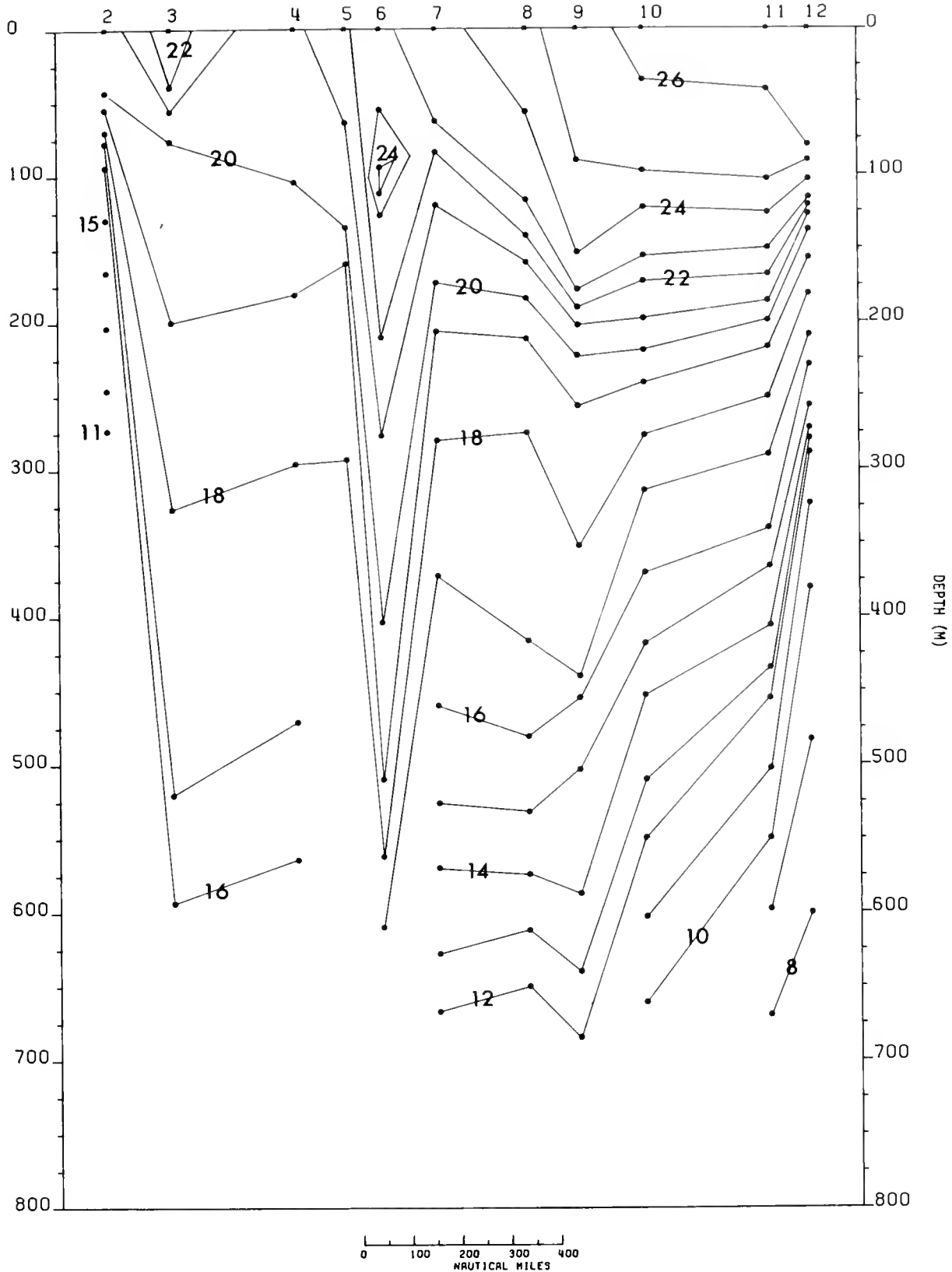
Figure 37.—Vertical distribution of temperature (°C) in the upper 750 m. Contour interval 1°C. Santa Cruz, 4-8 April 1972.
