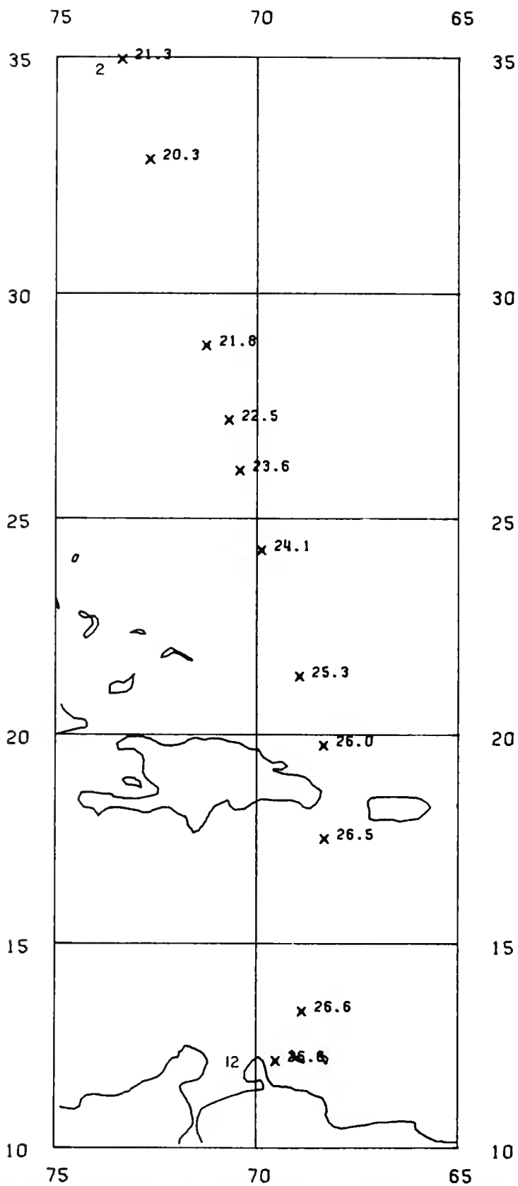
Figure 36.—Sea surface temperature (°C) along the cruise track with the first and last stations numbered. Santa Cruz, 4-8 April 1972.
