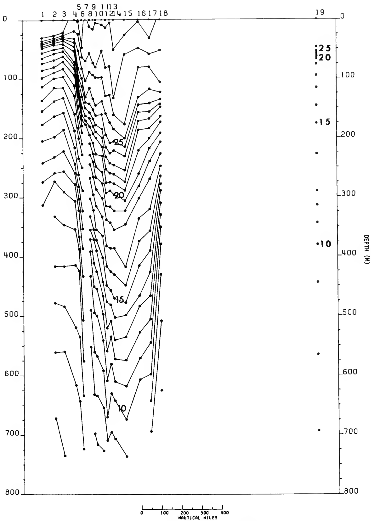
Figure 15. — Vertical distribution of temperature (°C) in the upper 750 m. Contour interval 1°C. Gulf Shipper , 21-28 August 1972.
