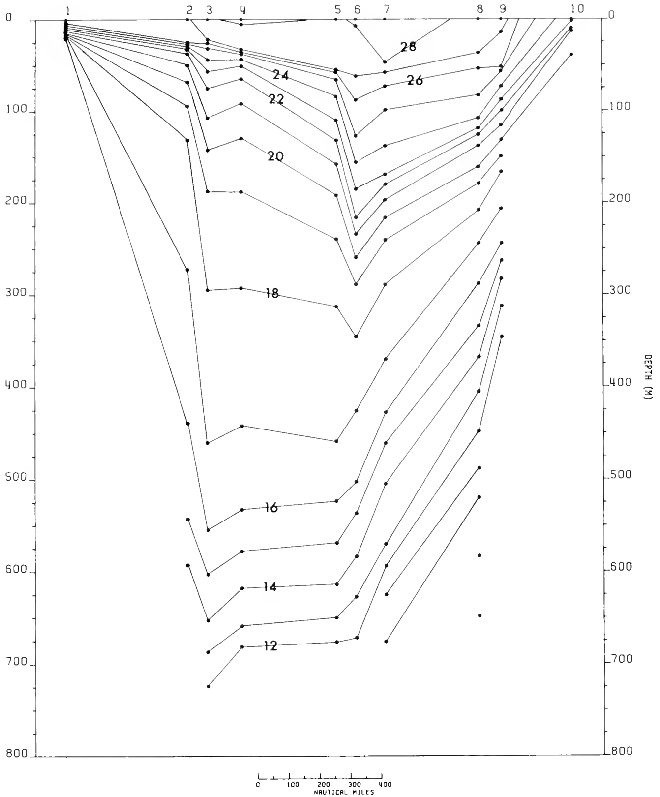
Figure 55.—Vertical distribution of temperature (°C) in the upper 750 m. Contour interval 1°C. Santa Cruz, 25-31 July 1972.
