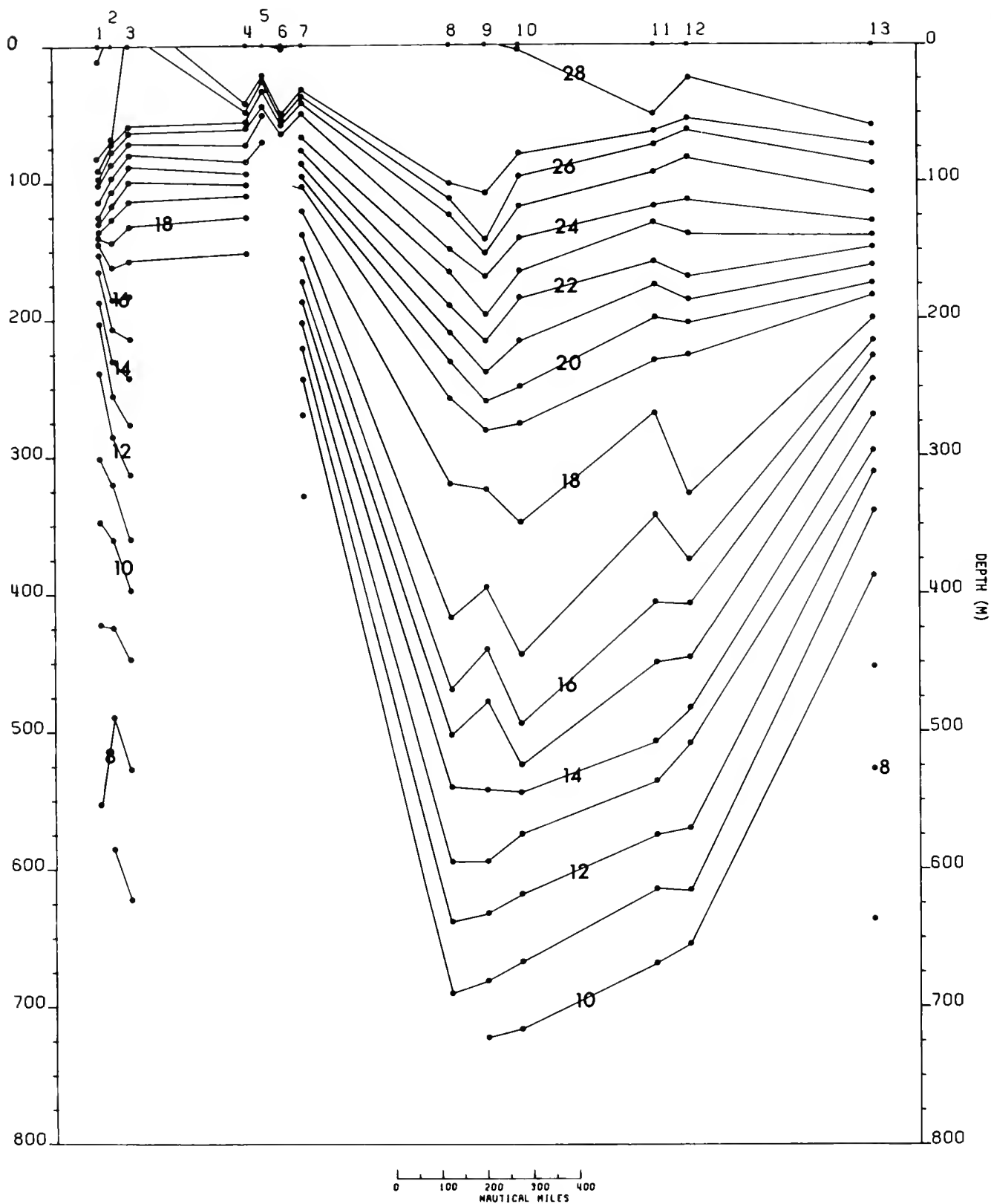
Figure 18.—Vertical distribution of temperature ( ^{\circ}\text{C} ) in the upper 750 m. Contour interval 1^{\circ}\text{C} . Delta Argentina, 14-18 November 1972.
