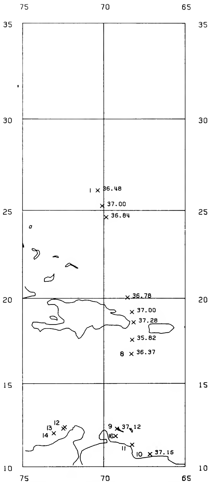
Figure 49.— Sea surface salinities (‰) along the cruise track with the first and last stations numbered. Santa Cruz, 28 June-14 July 1972.
