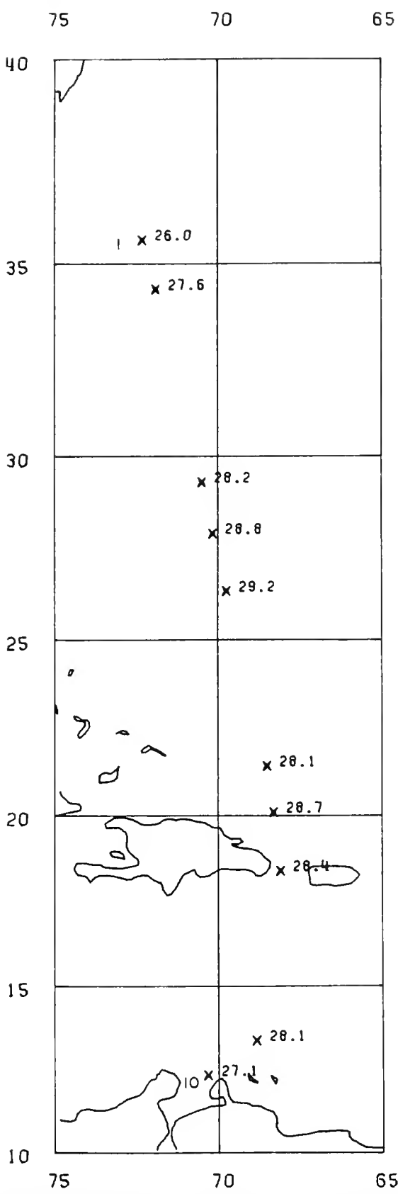
Figure 65.—Sea surface temperature ( ^{\circ}\text{C} ) along the cruise track with the first and last stations numbered. Santa Cruz , 17-30 September 1972.
