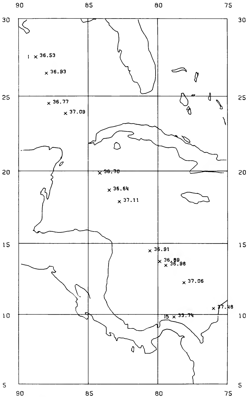
Figure 8. — Sea surface salinities (‰) along the cruise track with the first and last stations numbered. Gulf Shipper , 30 April-4 May 1972.
