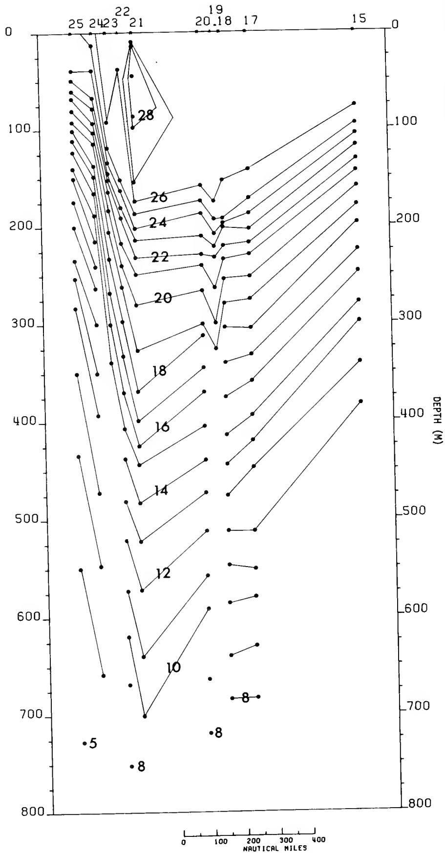
Figure 6.—Vertical distribution of temperature (°C) in the upper 750 m. Contour interval 1°C. Gulf Shipper , 26-28 March 1972.
