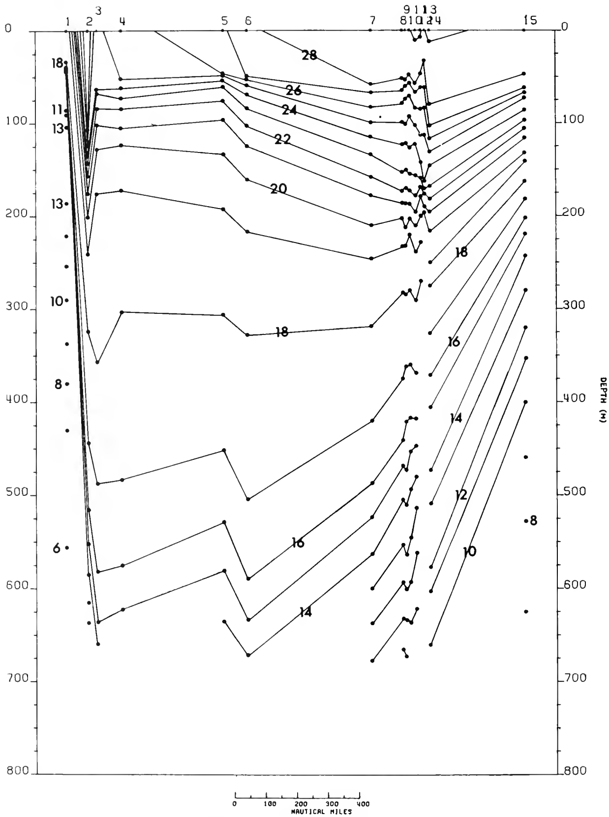
Figure 78. — Vertical distribution of temperature (°C) in the upper 750 m. Contour interval 1°C. Santa Cruz, 15-18 October 1972.
