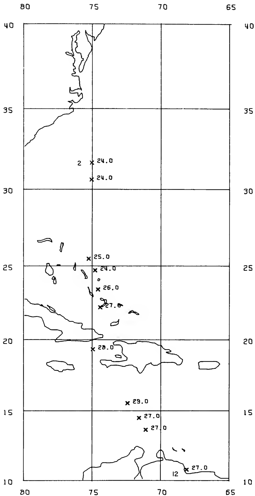
Figure 42.—Sea surface temperature (°C) along the cruise track with the first and last stations numbered. Santa Cruz , 29 May-8 June 1972.
