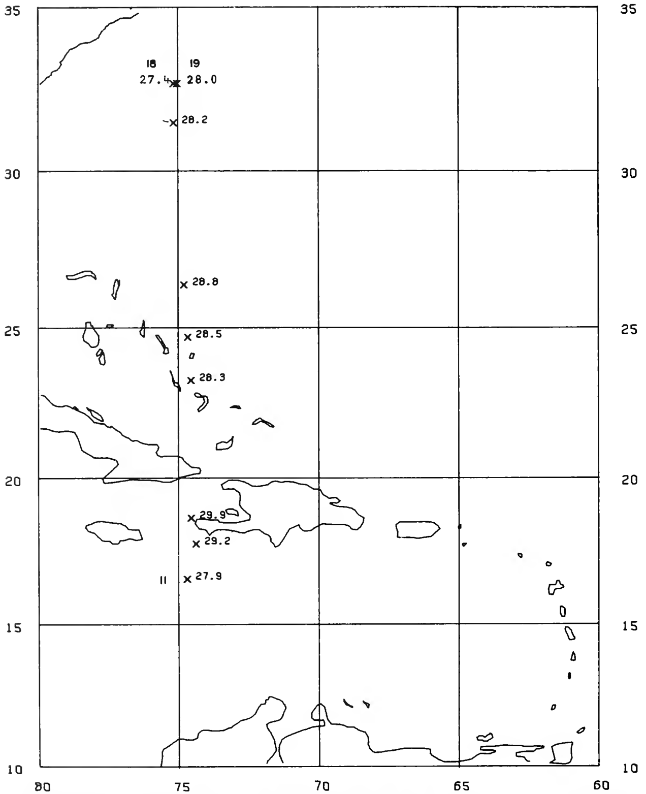
Figure 56.—Sea surface temperature (°C) along the cruise track with the first and last stations numbered. Santa Cruz , 11-14 August 1972.
