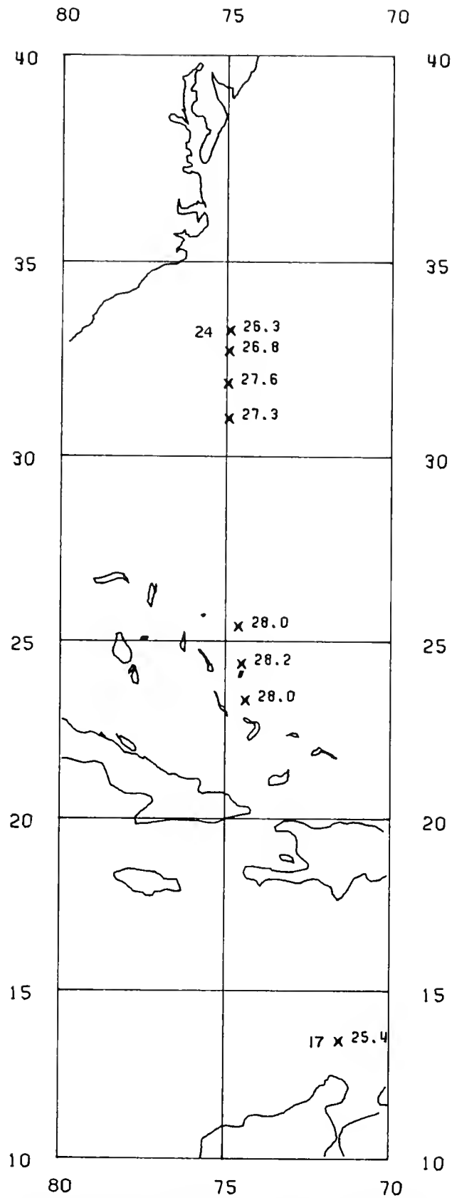
Figure 51.—Sea surface temperature (°C) along the cruise track with the first and last stations numbered. Santa Cruz, 15-18 July 1972.
