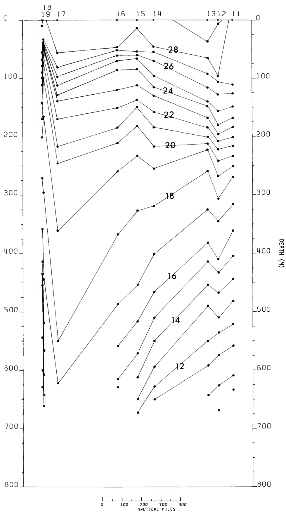
Figure 58.—Vertical distribution of temperature (°C) in the upper 750 m. Contour interval 1°C. Santa Cruz, 11-14 August 1972.
