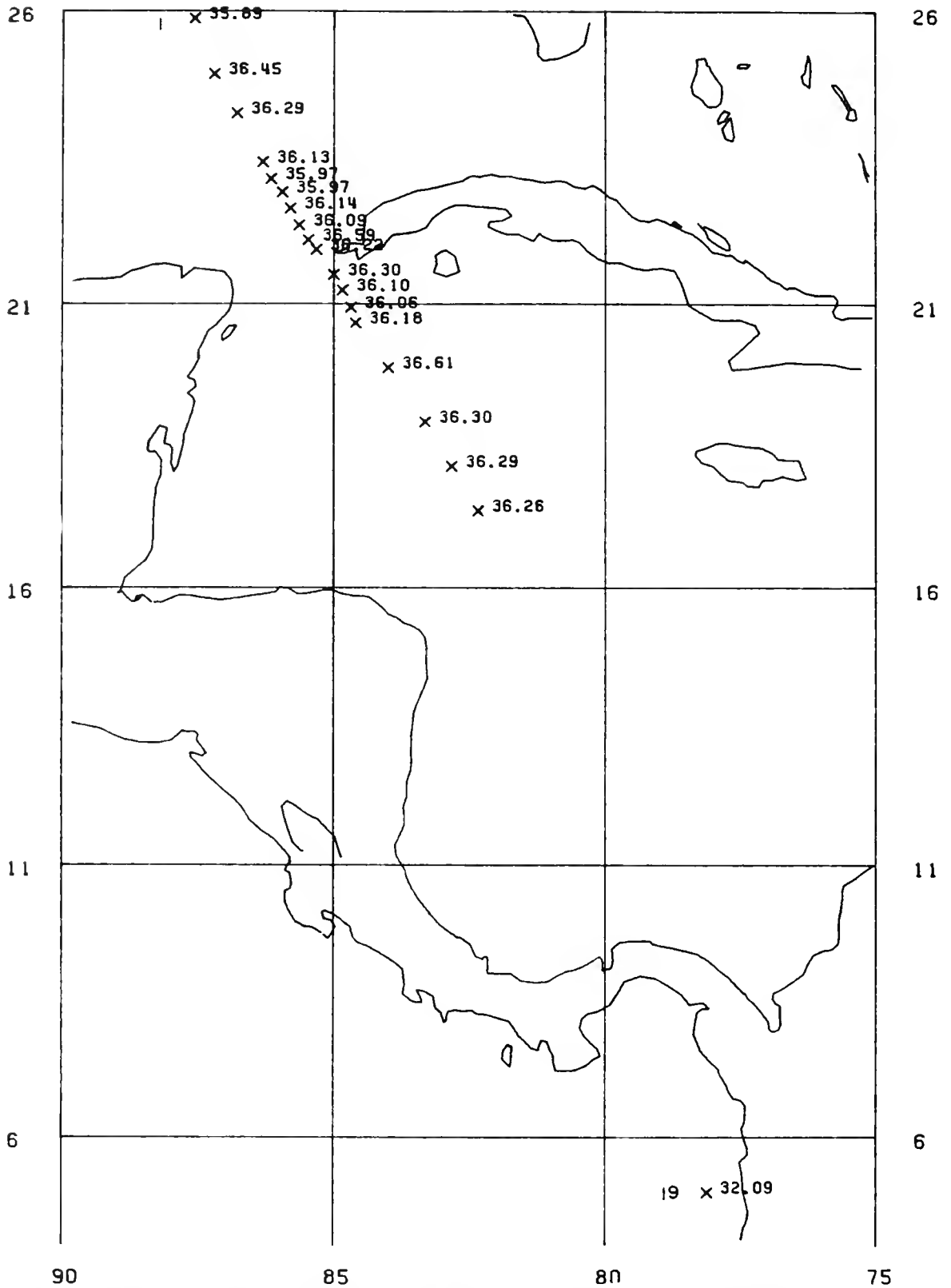
Figure 14.—Sea surface salinities (‰) along the cruise track with the first and last stations numbered. Gulf Shipper , 21-28 August 1972.
