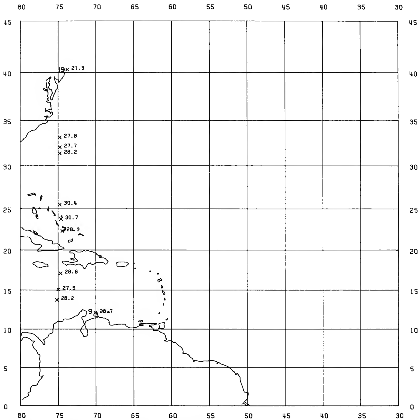
Figure 62.—Sea surface temperature (°C) along the cruise track with the first and last stations numbered. Santa Cruz , 2-13 September 1972.
