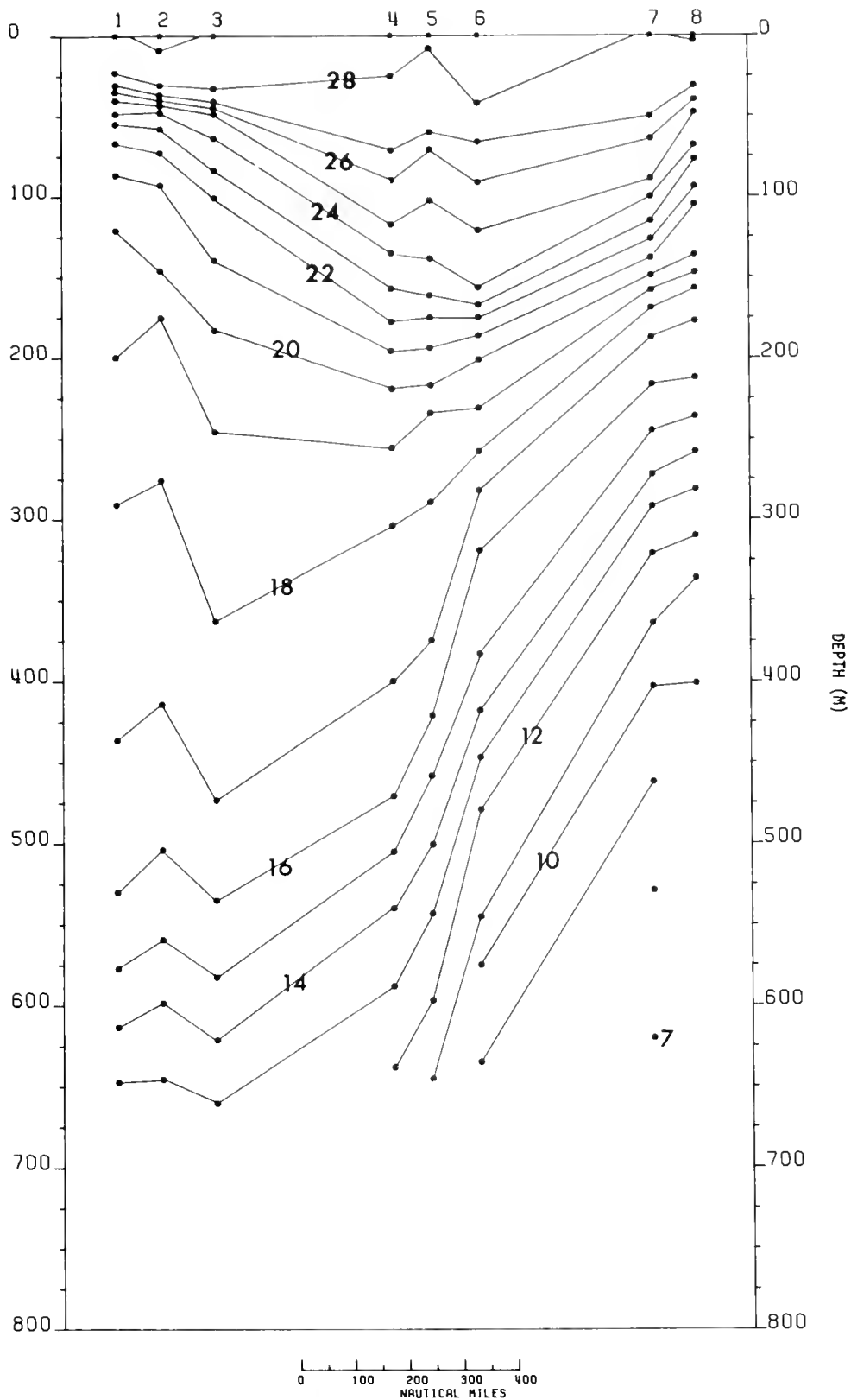
Figure 61.—Vertical distribution of temperature ( ^{\circ}\text{C} ) in the upper 750 m. Contour interval 1^{\circ}\text{C} . Santa Cruz, 21 August-1 September 1972.
