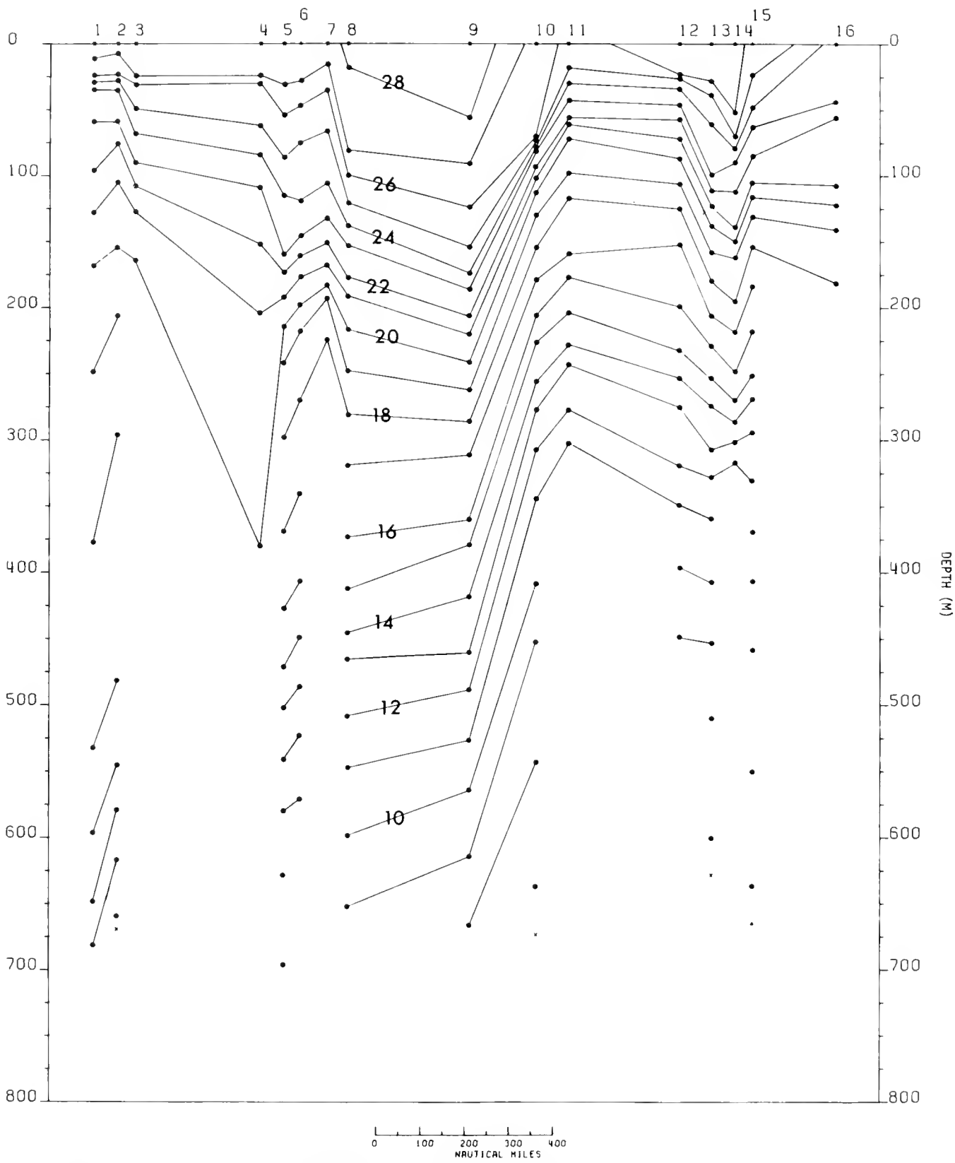
Figure 50. - Vertical distribution of temperature ( ^{\circ}\text{C} ) in the upper 750 m. Contour interval 1^{\circ}\text{C} . Santa Cruz, 28 June-14 July 1972.
