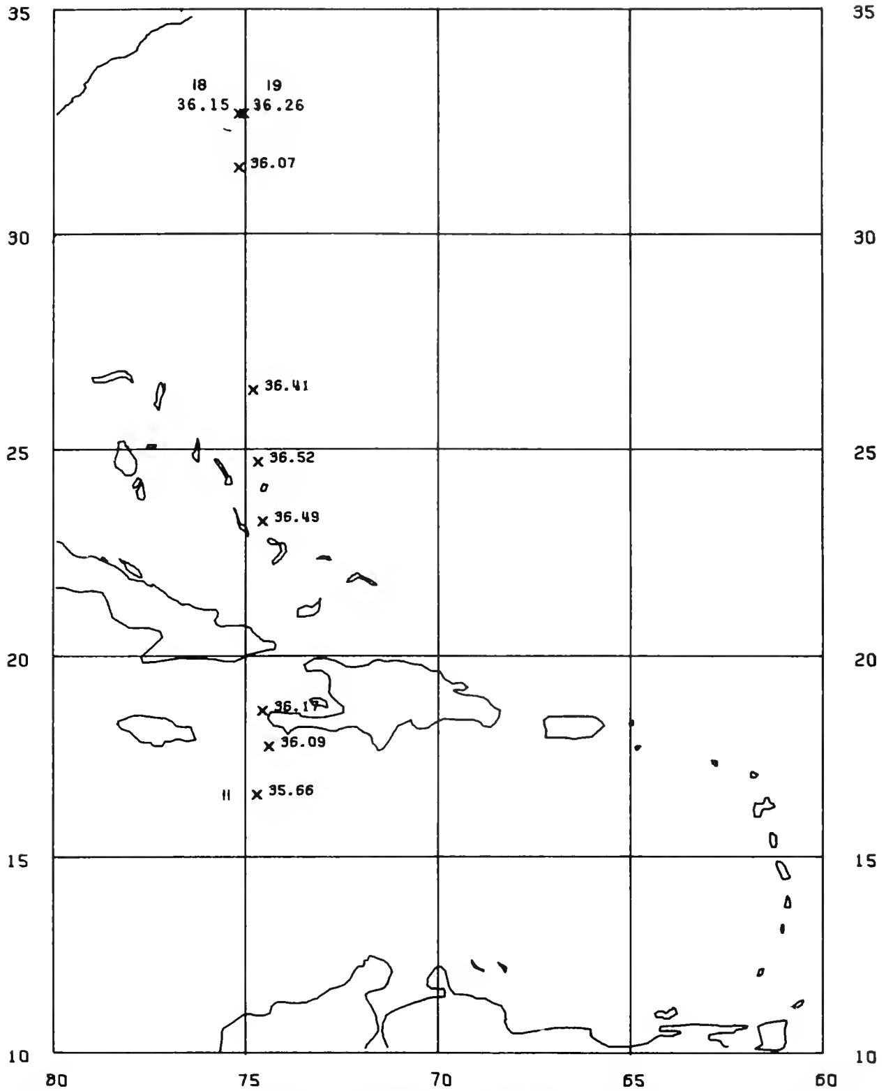
Figure 57.—Sea surface salinities (‰) along the cruise track with the first and last stations numbered. Santa Cruz , 11-14 August 1972.
