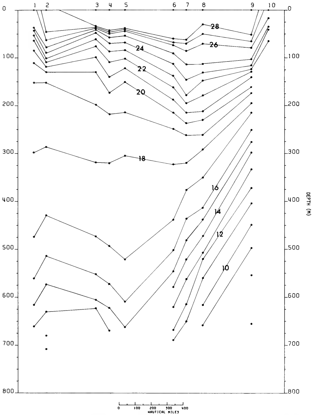
Figure 67.—Vertical distribution of temperature ( ^{\circ}\text{C} ) in the upper 750 m. Contour interval 1^{\circ}\text{C} . Santa Cruz, 17-30 September 1972.
