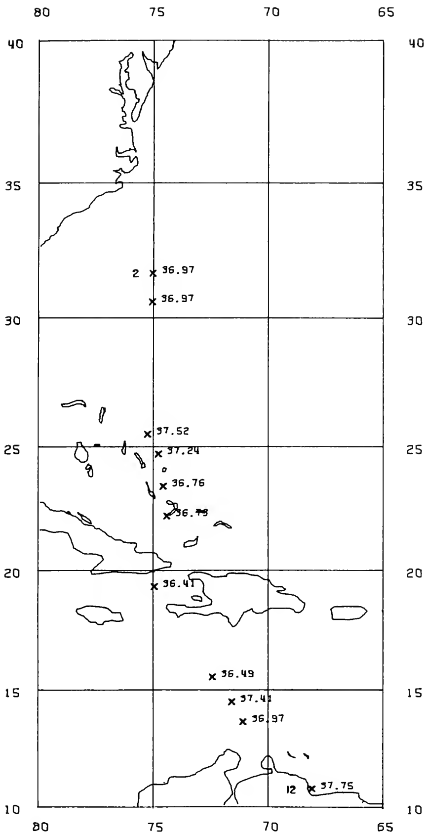
Figure 43.—Sea surface salinities (‰) along the cruise track with the first and last stations numbered. Santa Cruz, 29 May-8 June 1972.
