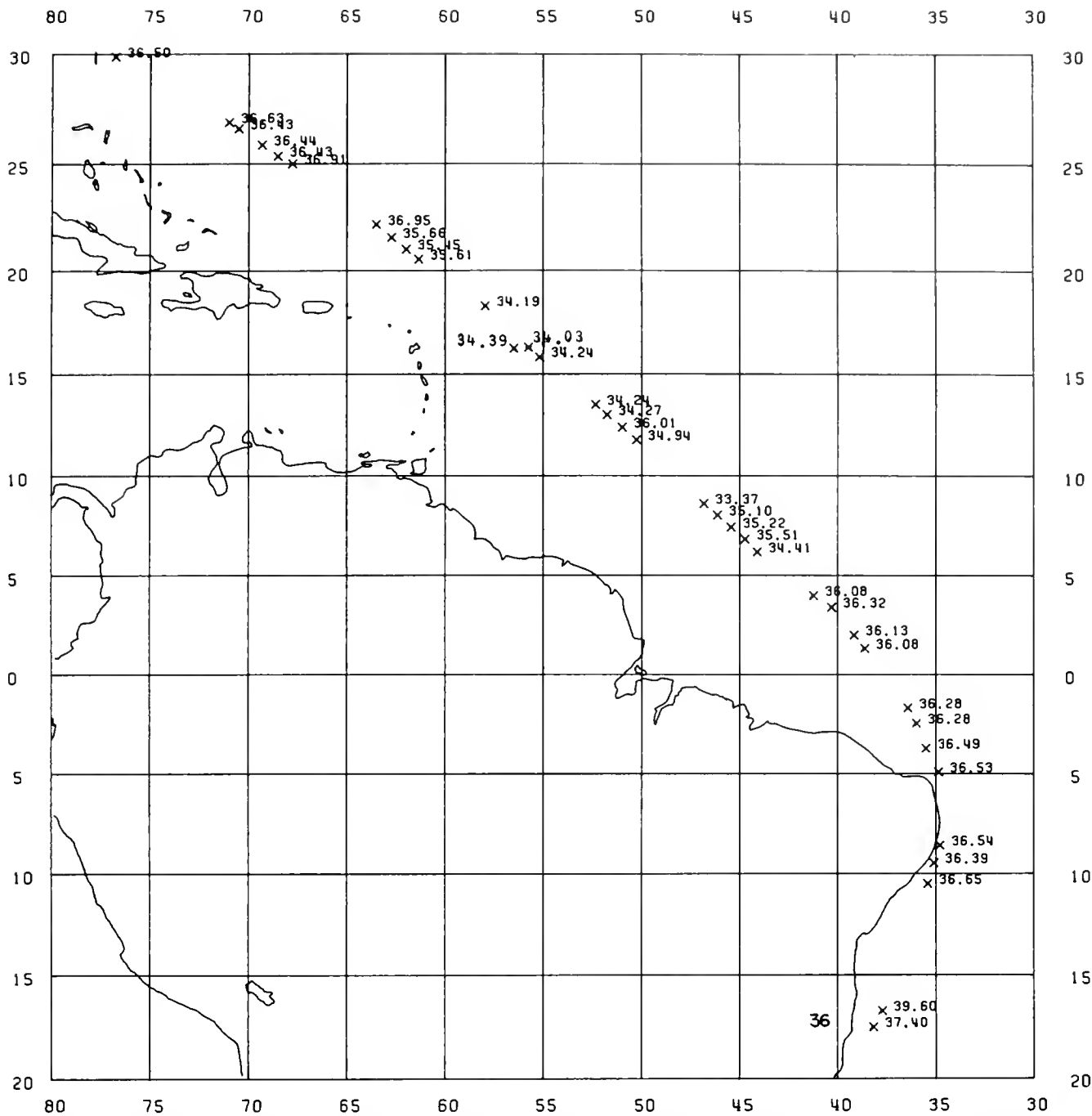
Figure 72.—Sea surface salinities (‰) along the cruise track with the first and last stations numbered. Mormac Pride , 4-13 October 1972.
