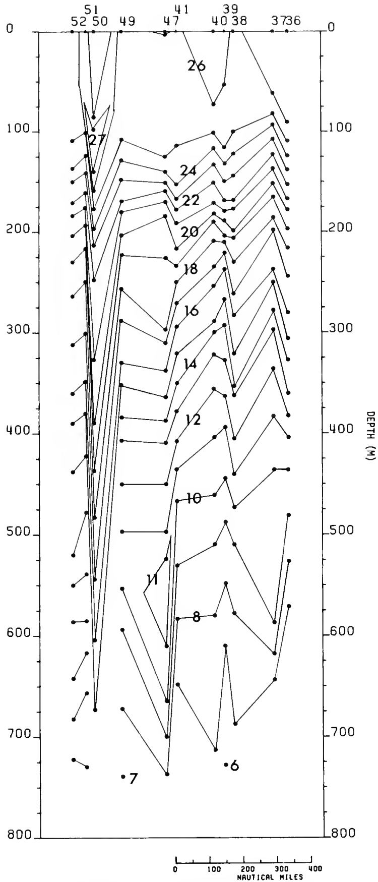
Figure 27.—Vertical distribution of temperature ( ^{\circ}\text{C} ) in the upper 750 m. Contour interval 1^{\circ}\text{C} . Bay State, 19-23 February 1972.
