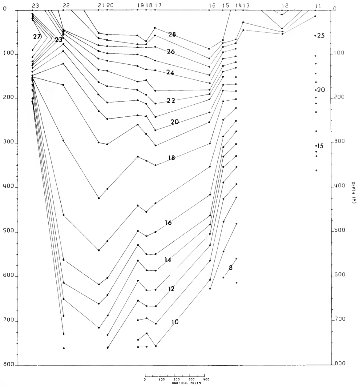
Figure 70.—Vertical distribution of temperature (°C) in the upper 750 m. Contour interval 1°C. Santa Cruz, 30 September-9 October 1972.
