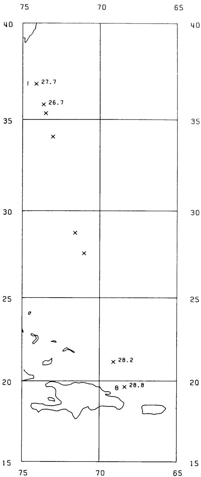
Figure 74.—Sea surface temperature (°C) along the cruise track with the first and last stations numbered. Santa Cruz , 15-18 October 1972.
