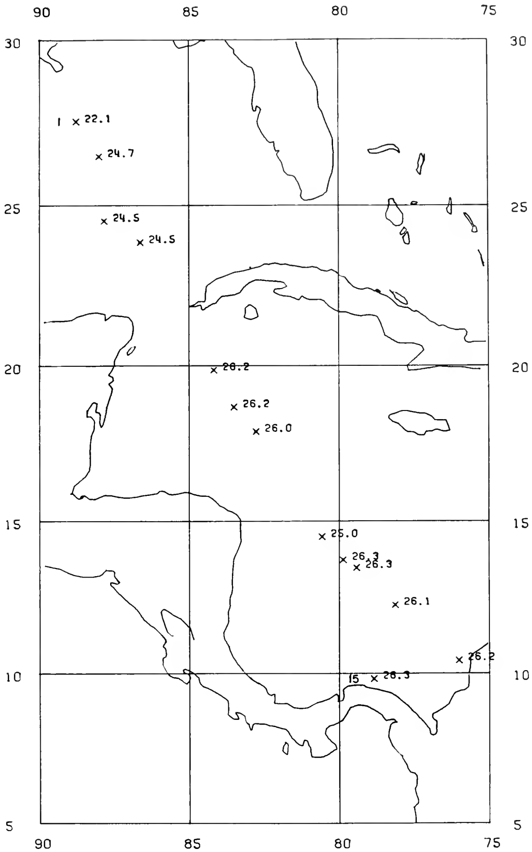
Figure 7.—Sea surface temperature (°C) along the cruise track with the first and last stations numbered. Gulf Shipper , 30 April-4 May 1972.
