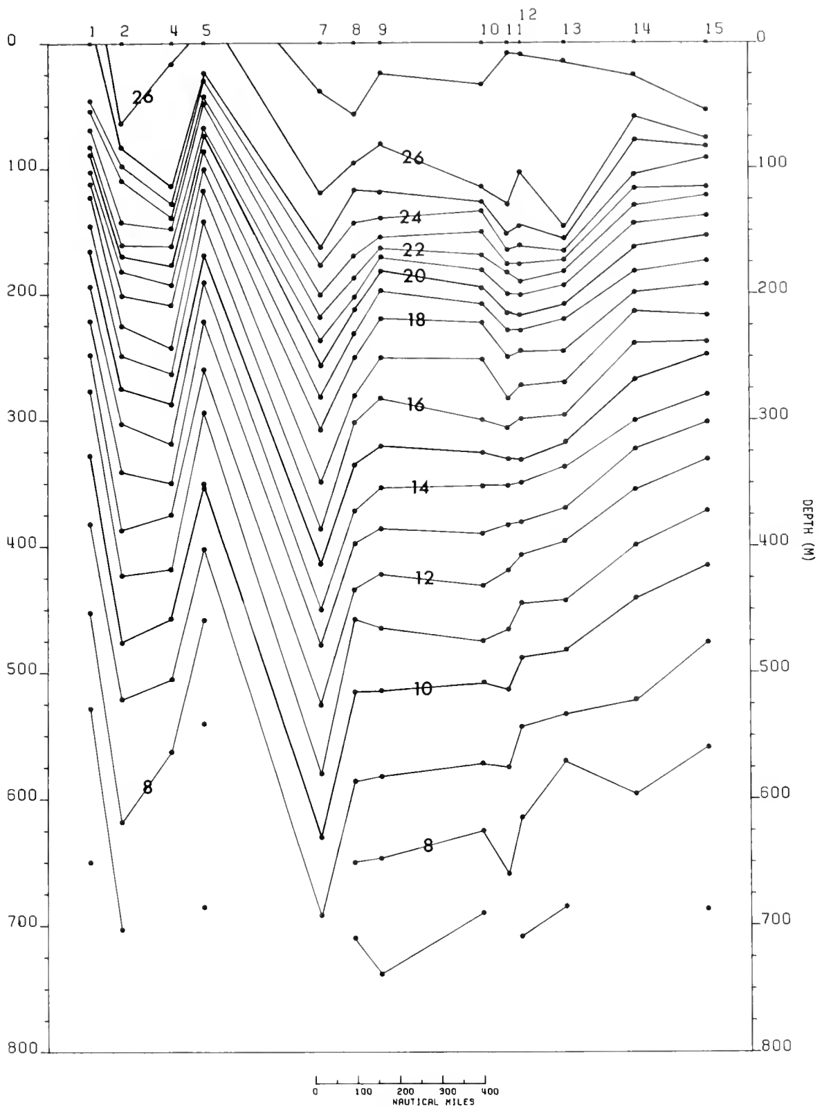
Figure 9.—Vertical distribution of temperature (°C) in the upper 750 m. Contour interval 1°C. Gulf Shipper , 30 April-4 May 1972.
