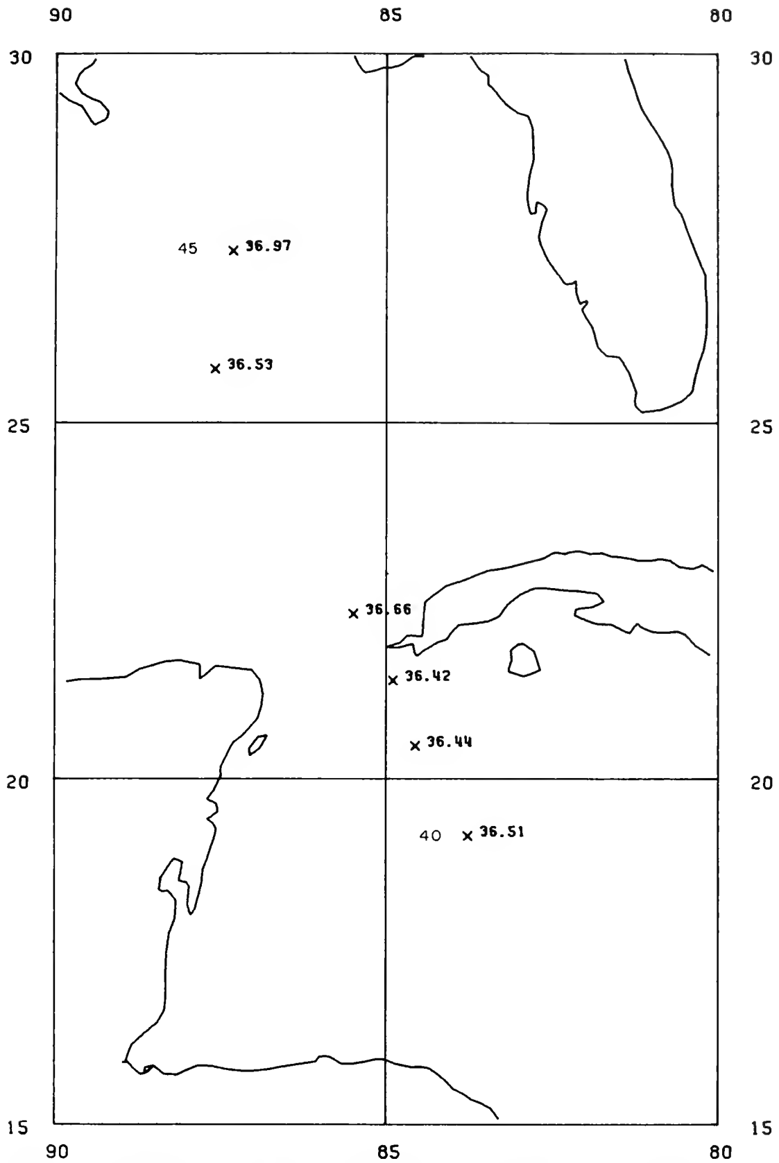
Figure 11.—Sea surface salinities (‰) along the cruise track with the first and last stations numbered. Gulf Shipper , 6-7 June 1972.
