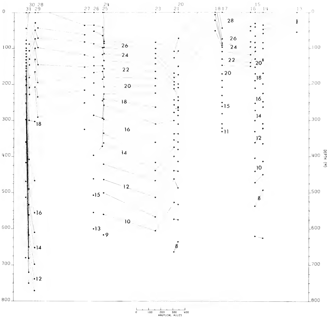
Figure 47.—Vertical distribution of temperature (°C) in the upper 750 m. Contour interval 1°C. Santa Cruz, 8-18 June 1972.
