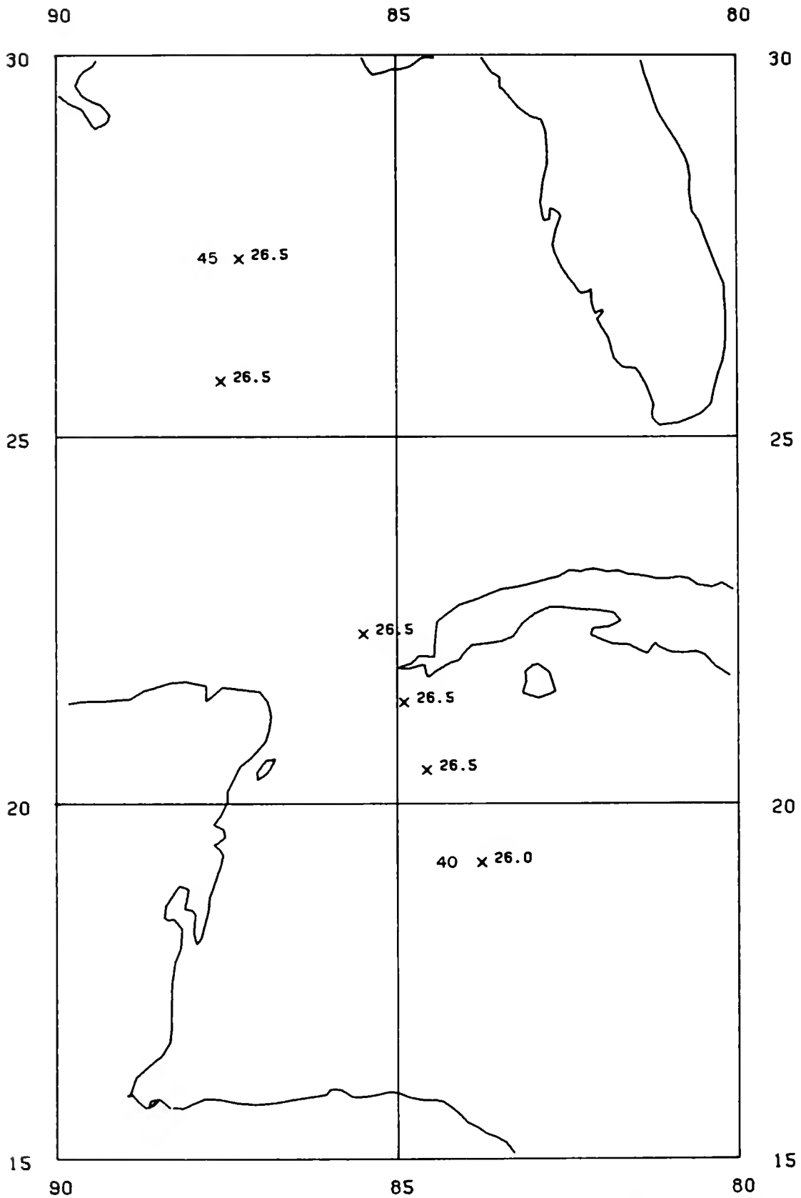
Figure 10.—Sea surface temperature (°C) along the cruise track with the first and last stations numbered. Gulf Shipper , 6-7 June 1972.
