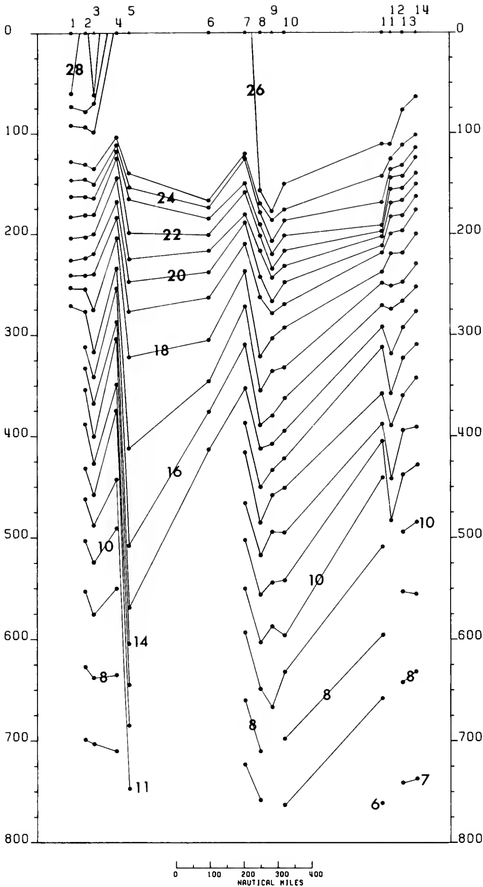
Figure 3.—Vertical distribution of temperature ( ^{\circ}\text{C} ) in the upper 750 m. Contour interval 1^{\circ}\text{C} . Gulf Shipper , 25-28 February 1972.
