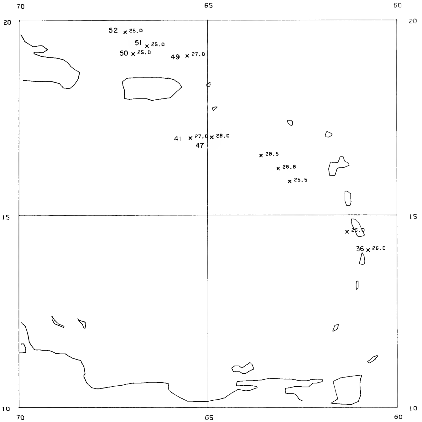
Figure 25.—Sea surface temperature (°C) along the cruise track with the first and last stations numbered. Bay State , 19-23 February 1972.
