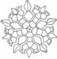
FIG. 1891. Eucalyptocrinus . (After Weller.)
