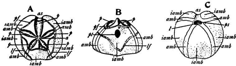
FIG. 1911. Diagram of Linthia variabilis . A , dorsal view; B , posterior view; C , ventral view. (After A. W. Slocum.) a , apical system; amb , ambulacra; as , anterior sulcus; iamb , interambulacra; lf , lateral fasciole; p , petaloid part of ambulacrum; pf , peripetalous fasciole; pi , periproct; ps , peristome.
