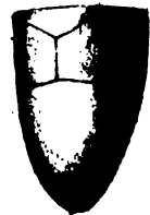
FIG. 1832. Agassizocrinus conicus , basal por-
