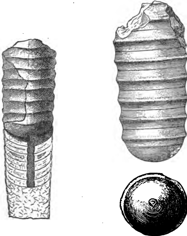
FIG. 1260. Dawsonoceras annulatum . (After Barrande.)
