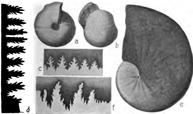
FIG. 1410. a-c. , Arcestes andersoni , \times \frac{1}{2} , and suture; d. , A. (Proarcestes) pacificus , suture; e, f. , Ussuria waageni , \times \frac{1}{2} , and suture. (After Hyatt and Smith.)
