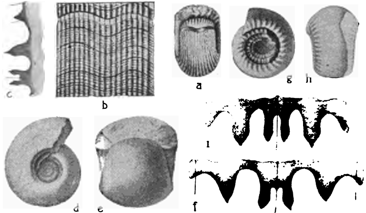
FIG. 1395. a, b , Gastrioceras entogonum , \times \frac{2}{3} , and surface enlarged; c-e , G. globulosum , suture and shell \times \frac{2}{3} ; f-h , G. listeri , suture enlarged and shell \times \frac{2}{3} ; i , G. noliense , suture enlarged. (After J. P. Smith.)
