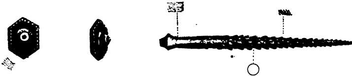
FIG. 1913. Archaocidaris shumardana , plates and spine, \times 2 . (After Hall.)
