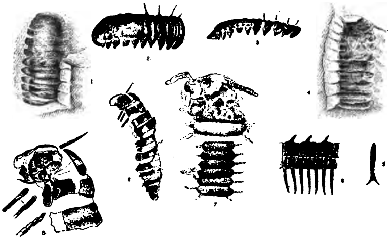
FIG. 1722. Myriopods from the coal measures: (1) Amynilispa wortheni , dorsal view, \times \frac{1}{3} ; (2) dorsolateral view of same, \times \frac{1}{3} ; (3) lateral view of same, \times \frac{1}{3} ; (4) view of rock mold of the same, \times \frac{1}{3} ; (5) Eileticus anthracinus , anterior portion of figure 6 enlarged, \times 2 ; (6) entire specimen, \times \frac{2}{3} ; (7) Euphoberia armigera ,
