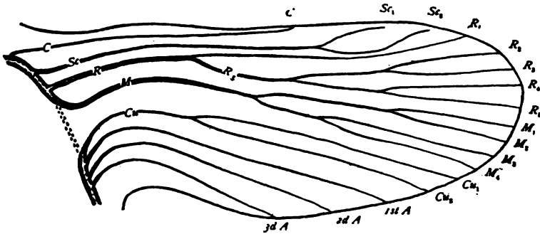
FIG. 1724. Diagram of the tracheation of a primitive insect wing. (Hypothetic. After Comstock and Needham.) C, costa; Sc, subcosta; Sc 1 , Sc 2 , first and second subcostal branches; R, radial sector; R 1 -R 5 , branches of radial groups; M, media; M 1 -M 4 , branches of media; Cu, cubitus; Cu 1 , Cu 2 , branches of cubitus; 1st A-3d A, first, second and third anal veins.
