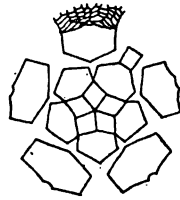
FIG. 1897. Crotalocrinus , analysis of calyx. (After Weller.)
