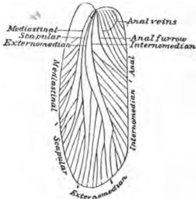
FIG. 1737. One of the tegmina of Etoblattina ( Asemoblatta ) mazona , \times 2 , with the parts named. The areas are marked along the margin, the veins are marked at the base of the tegmina. (After Scudder.)
