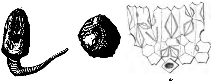
FIG. 1770. Glyptocystites multiporus . a, Anal opening.
