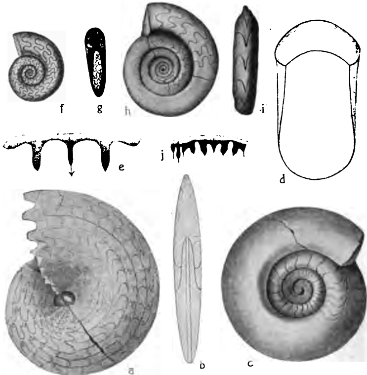
FIG. 1398. a, b, Prodrornites gorbyi , \times \frac{2}{3} ; c, d, Prolecanites compactus , \times \frac{2}{3} ; e , suture enlarged; f, g, P. greenii , \times \frac{2}{3} ; h-j, P. lyoni , shell \times \frac{2}{3} , and suture enlarged. (All after J. P. Smith.)
