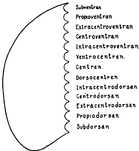
FIG. 1231. Diagram illustrating method of naming location of siphuncle. (After Hyatt.)
