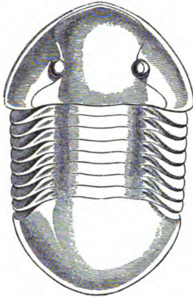
FIG. 1602. Isotelus gigas , broad form. (After Logan.)
