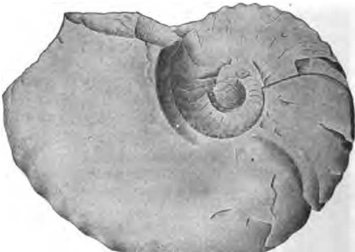
FIG. 1315. Centroceras ohioense , \times \frac{1}{2} . (After Meek, Ohio Pal.)
