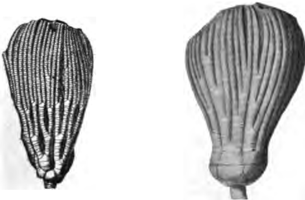
FIG. 1826. Woodocrinus æqualis , \times \frac{2}{3} . (After Meek and Worthen.)
