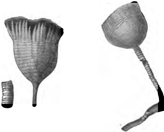
FIG. 1900. Ichthyocrinus levis , with enlargement of stem. (After Hall.)
