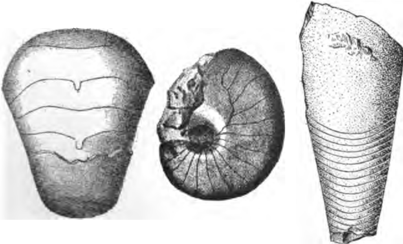
FIG. 1328. Solenocheilus collectus , views of two individuals. (After Meek and Worthen, Ill. Geol., V.)
