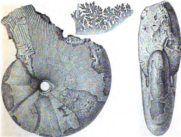
FIG. 1412. Phylloceras knoxvillense , shell \times \frac{2}{3} , and septum. This is inverted, and the finer divisions of the saddle are too narrow. (After Stanton.)
