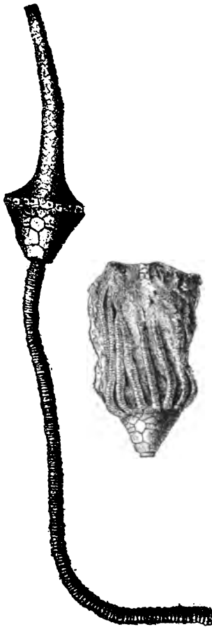
FIG. 1875. Macrocrinus verneuillianus , two specimens, one with arms, the other with proboscis and stem. (After Meek and Worthen.)
