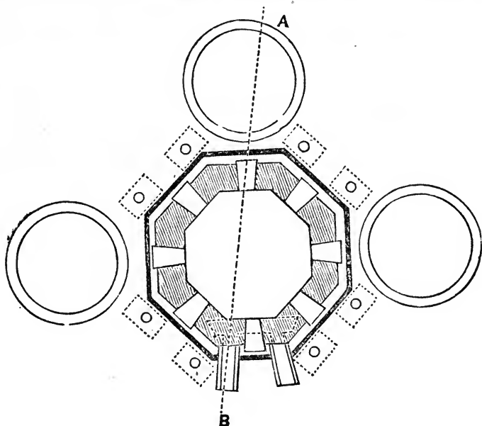
Figure 11.--Horizontal Section.
