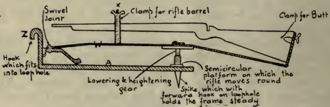
SECTIONAL ELEVATION.
