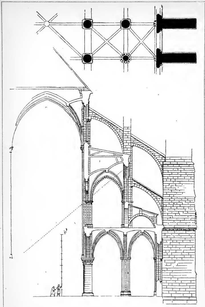
SECTION OF NAVE AND DOUBLE AISLE, AND A PLAN OF ONE BAY. SCALE 1 INCH = 29 FEET.
