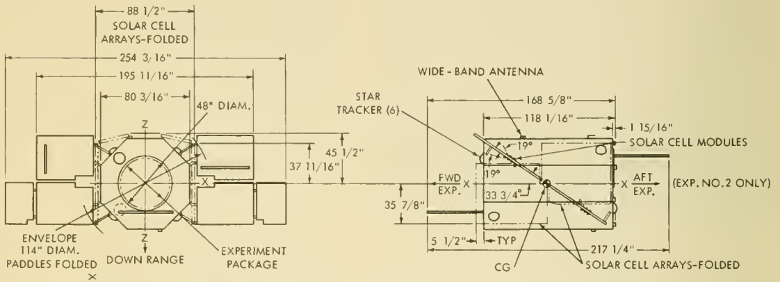
FIGURE 6-1. OAO general arrangement (double-ended experiment, spacecraft no. 1).
