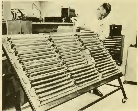
FIGURE 2-8. Thermal control louvers.
