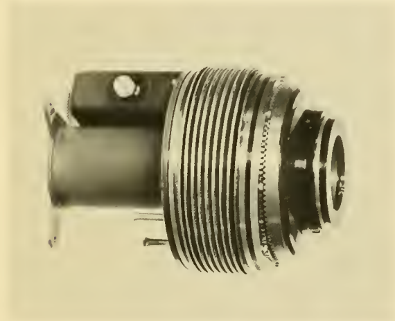
FIGURE 2-13. Wobble gear.
