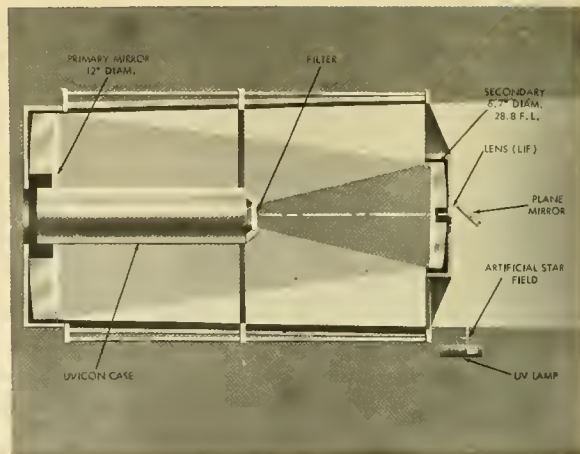
FIGURE 5-4. Schwarzschild camera as used in Celeste.
