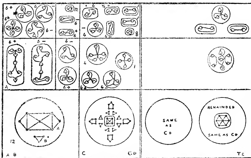
CADMIUM (Plate IX, 3).
