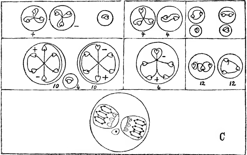
TITANIUM (Plate III, 6, and XV, 2, 3).
