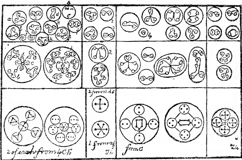
ZIRCONIUM (Plate XV, 2, 5).
