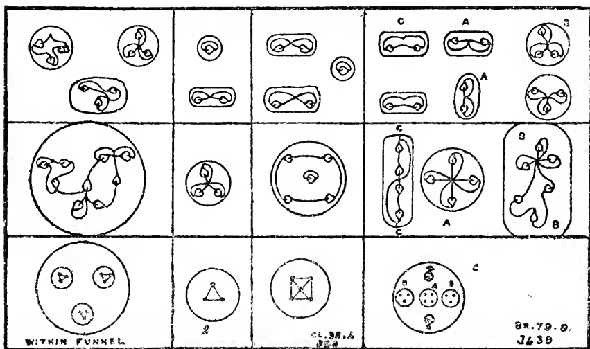
BROMINE (Plate V, 3).
