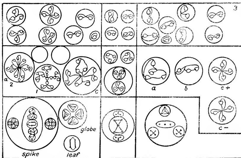
POTASSIUM (Plate XIX, 2).
