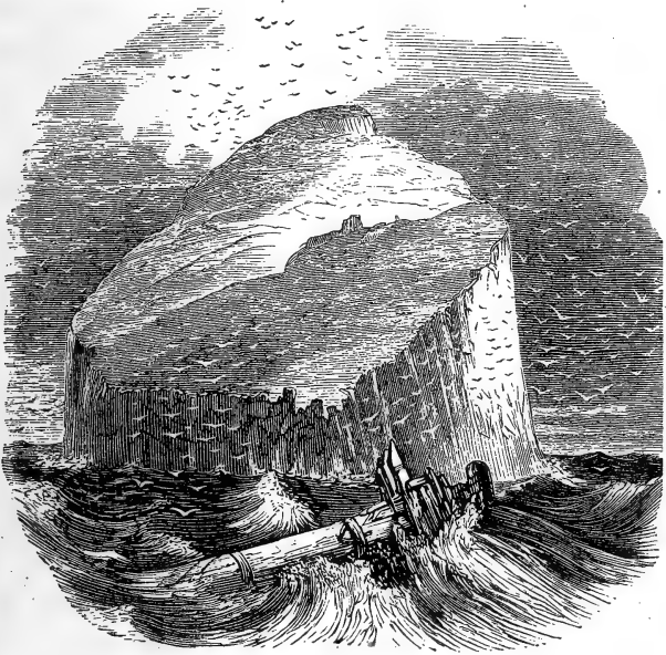
THE BASS ROCK.
