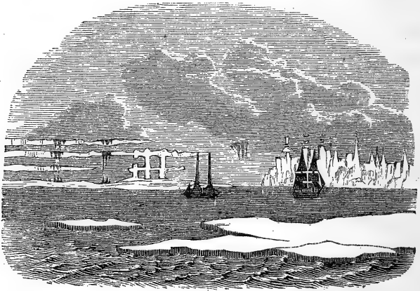
DISTORTIONS OF IRREGULAR REFRACTION.
