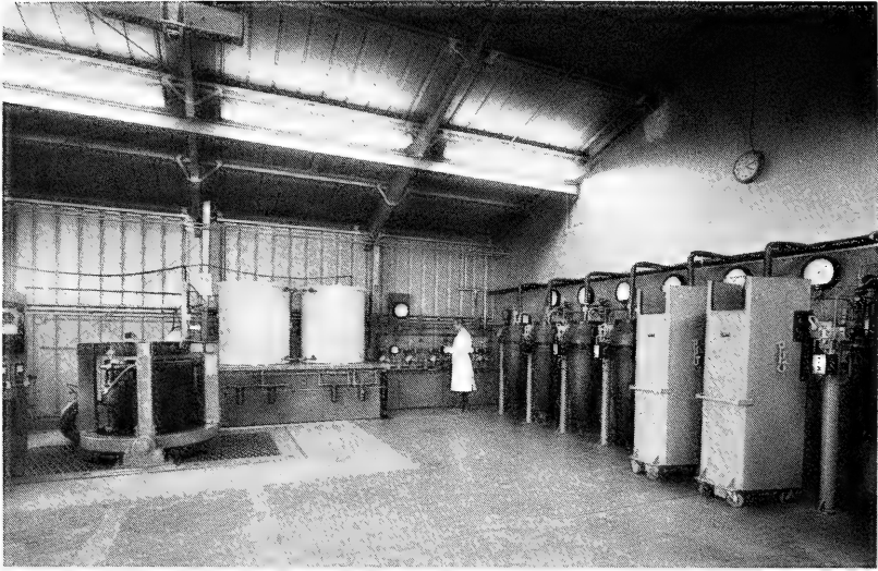
The Deep Ocean Simulation Laboratory at NCEL, showing six 9-in.-ID pressure vessels and one 18-in.-ID pressure vessel used to simulate the deep-ocean environment. Tanks in the background are for sea water storage.
