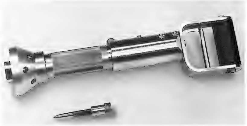
Large-velocity powered stud gun. Capable of operating to 1000 ft, this gun can drive solid steel studs into 1-1/8-in. thick mild steel plate.
