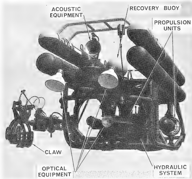
Controlled Underwater Recovery Vehicle (CURV). CURV, an unmanned recovery vehicle, was used to pick up the unarmed nuclear weapon at Palomares, Spain, in 1966. The claw and propulsion motors are controlled from the surface by personnel using closed-circuit TV for direction.
