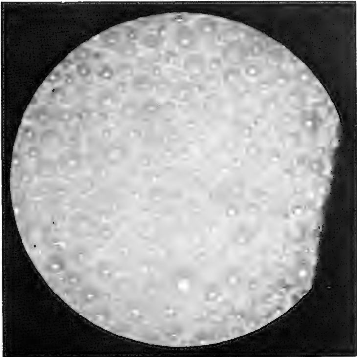
Syntactic foam, one of the low-density materials being developed for use as auxiliary buoyancy for deep-submergence vehicles. It is composed of hollow glass microspheres embedded in a plastic matrix and has a density of 40 to 46 lb/ft 3 .
