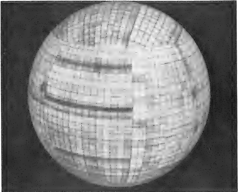
Fiberglass reinforced plastic sphere, a recently developed low-density material for use as auxiliary buoyancy in deep-submergence vehicles
