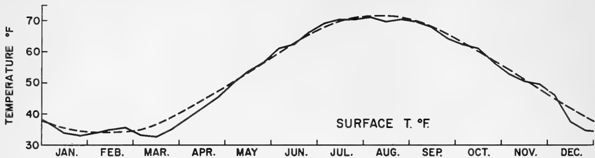
Figure 8.--Woods Hole, Massachusetts. (Dashed line mean for period 1950-59.)
