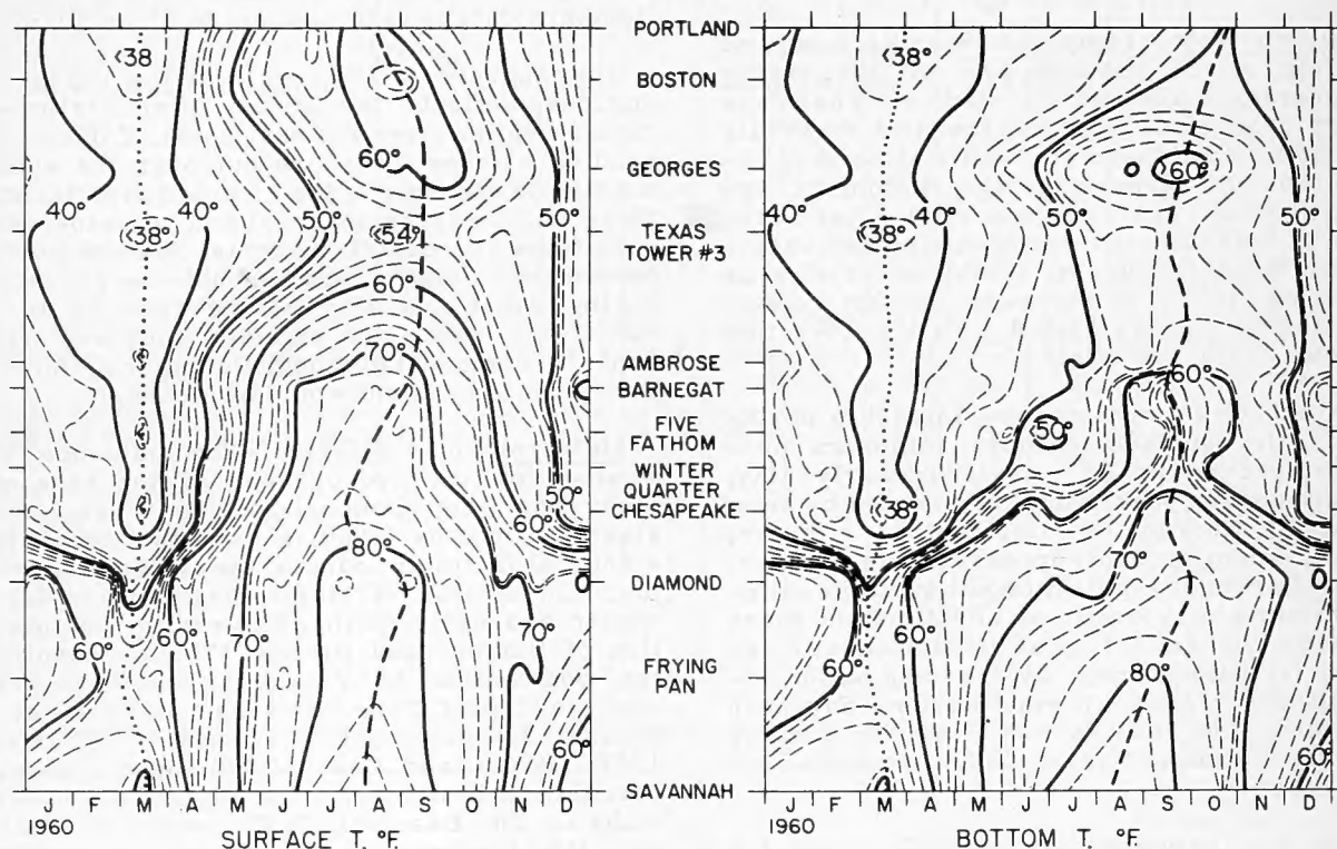
Figure 1.--The cycle of temperature at the surface (left) and bottom (right) along the series of observation posts for 1960. Heavy dotted and dashed lines indicate minimum and maximum temperatures respectively.
