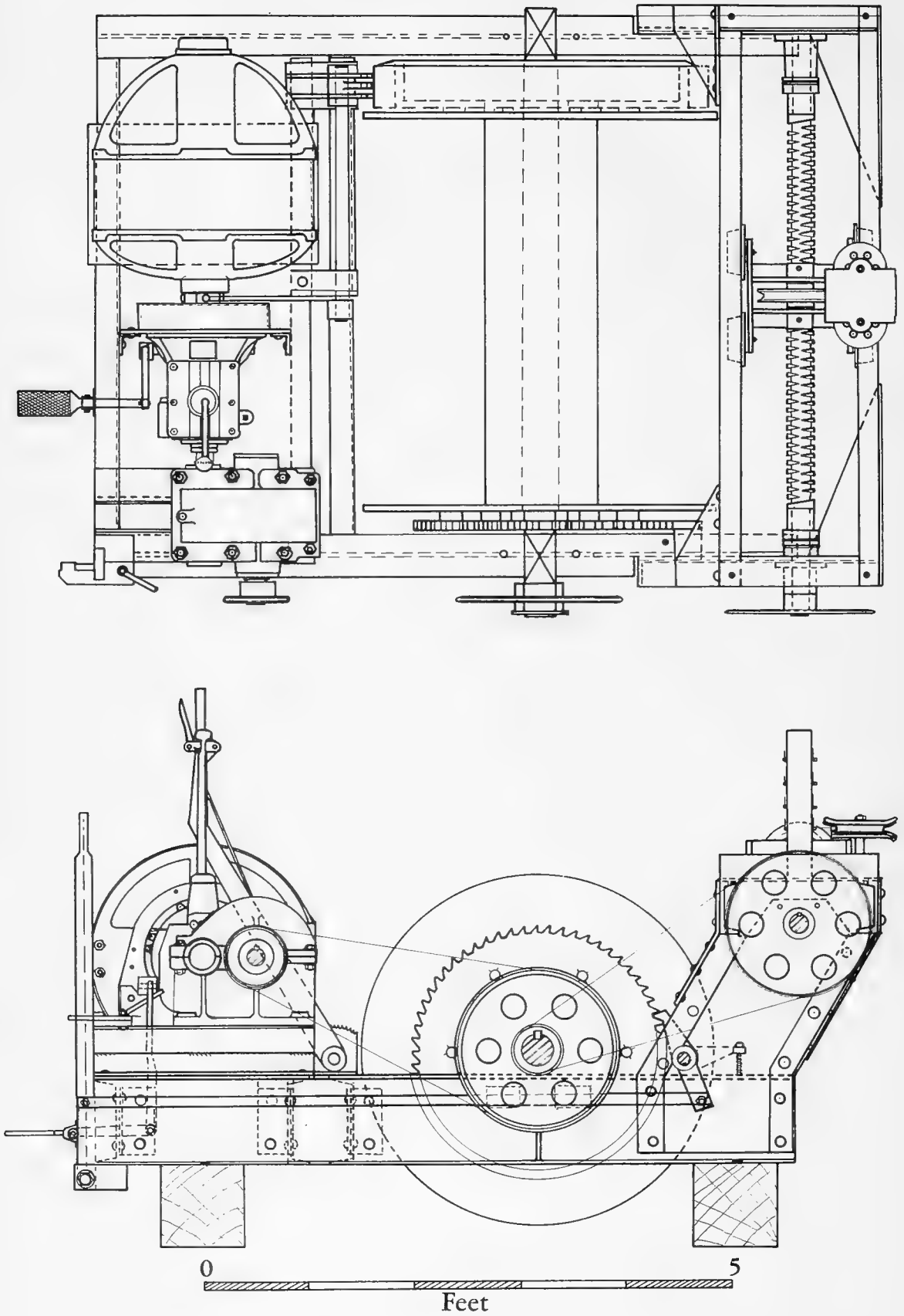
Fig. 8. Dredging winch.
