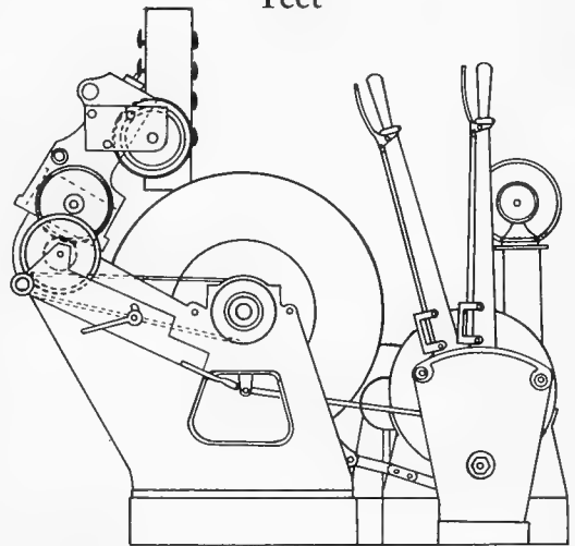
Fig. 7. Hydrographic winch.
