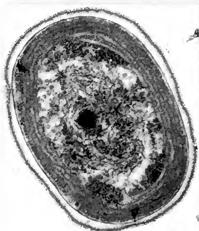
0.5 micrometers Transmission electron micrograph of a thin section of Prochlorococcus sp.
