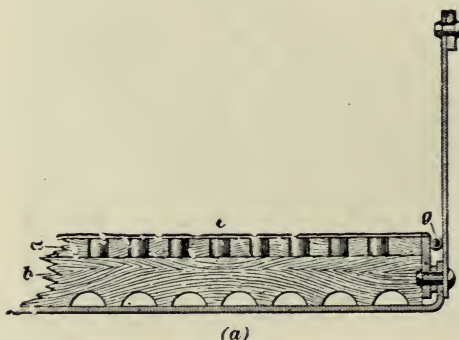
FIG. 71. SECTION OF STEEL LEACHING VAT.
