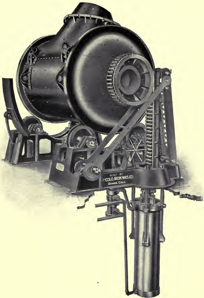
FIG. 121. COPPER CONVERTER.
