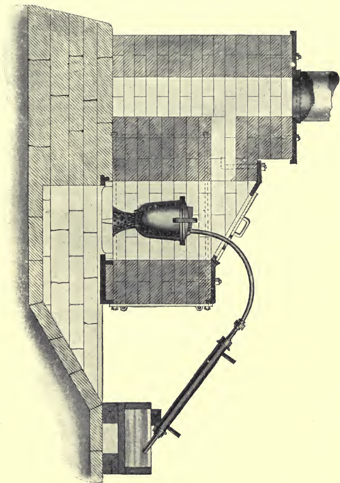
FIG. 52. GOLD RETORT.
