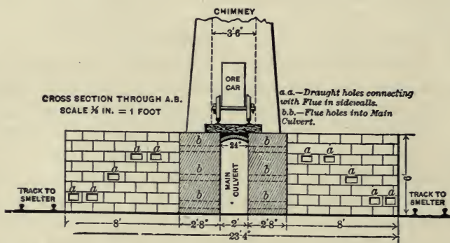
FIG. 25. ROASTING STALLS FOR LUMP ORE (SECTIONAL ELEVATION).
