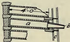
FIG. 142. ZINC-SMELTING RETORTS.
