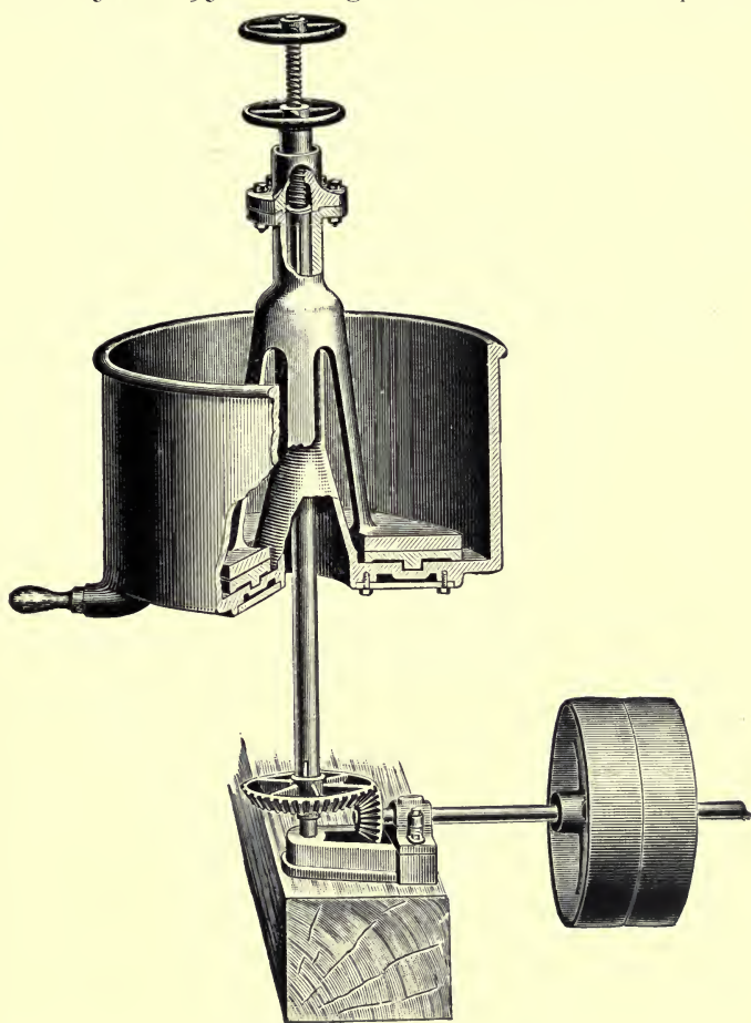
FIG. 51. CLEAN-UP PAN.
