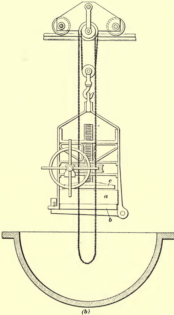
FIG. 147. HOWARD PRESS.
