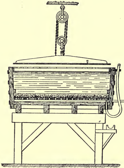
FIG. 54. CHLORINATION LEACHING TANK.
