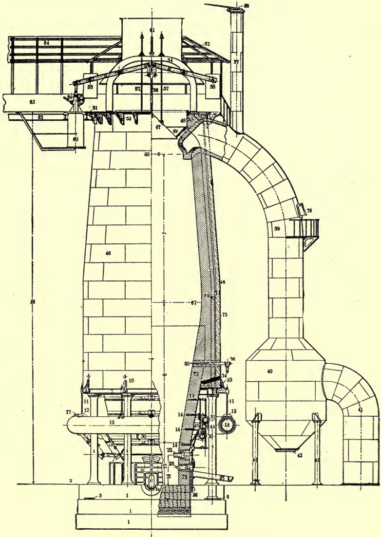
FIG. 96. IRON BLAST-FURNACE.
