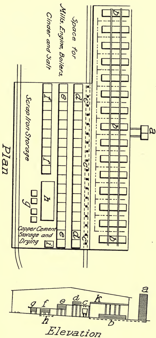
FIG. 119. HENDERSON-PROCESS PLANT.
