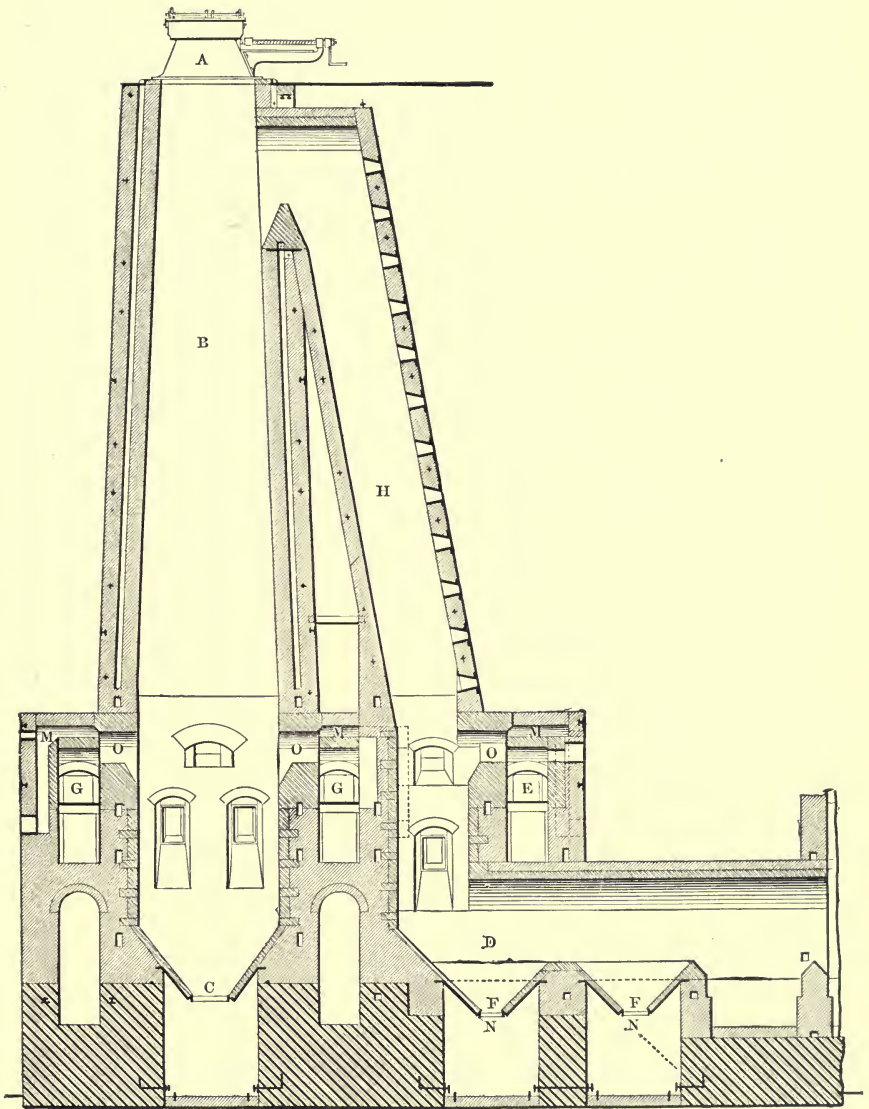
FIG. 42. STETEFELDT ROASTING FURNACE.
