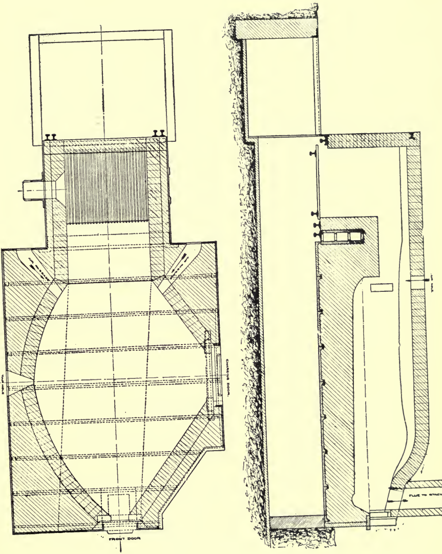
FIG. 159. COPPER REFINING FURNACE. (Sectional Elevation.) FIG. 158. COPPER REFINING FURNACE. (Plan.)
