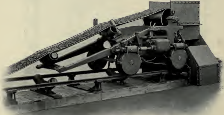
FIG. 167. CONVEYING BELT WITH TRIPPER.
