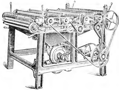
COTTON SHEAR.
