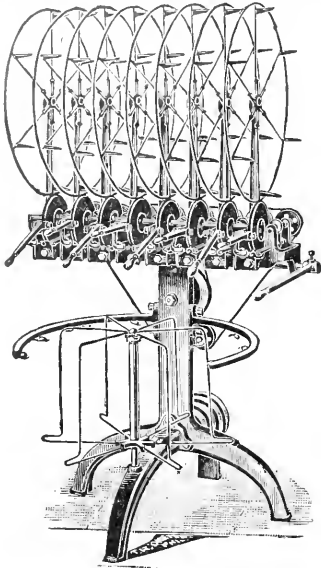
Back-winding Machine for winding the yarn from imperfect pieces back into skeins.
