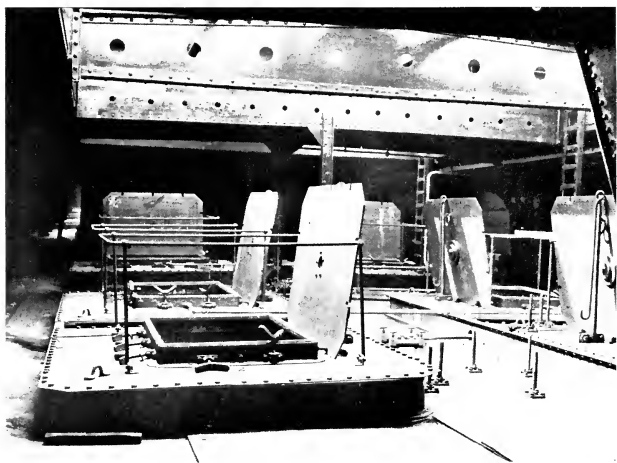
OIL-TANKS OF THE "SAN FRATERO."
