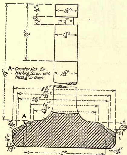
FIG. 84.—McIntosh & Seymour Diesel exhaust valve.
