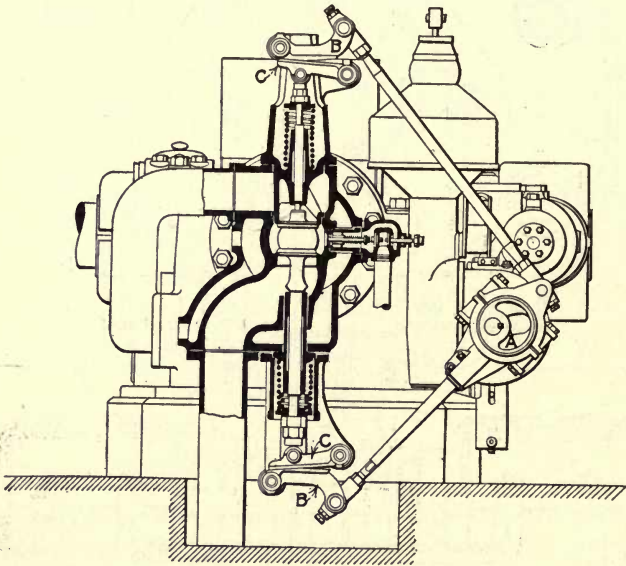
FIG. 97.—Allis-Chalmers Diesel valves and rockers.
