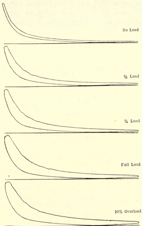
FIG. 200.—Indicator cards. Allis-Chalmers Diesel.
