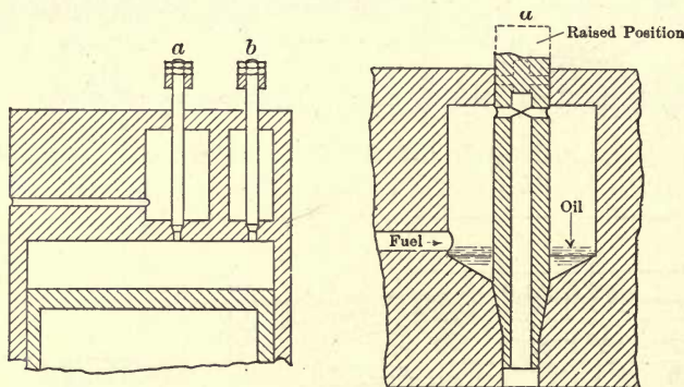
FIG. 231.—Müller super compression ignition device.
