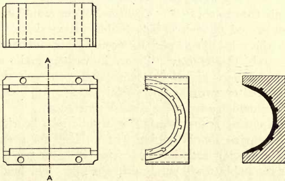
FIG. 270.—Big-end rod bearing.
