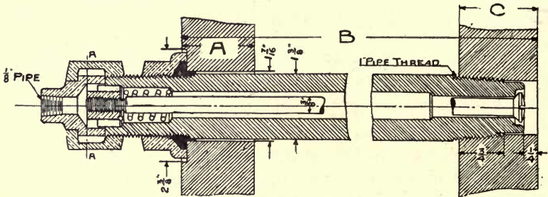
Fig. 174.—Cylinder lubrication check valve.
