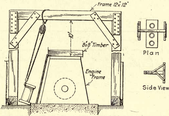
FIG. 24A.—Scaffolding.
