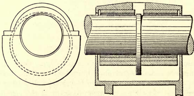
FIG. 284.—Main bearing.
