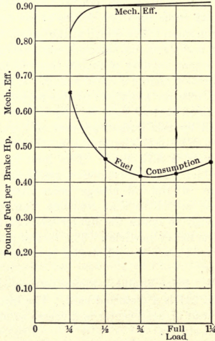
FIG. 242.—Test on 19x24 Price engine.
