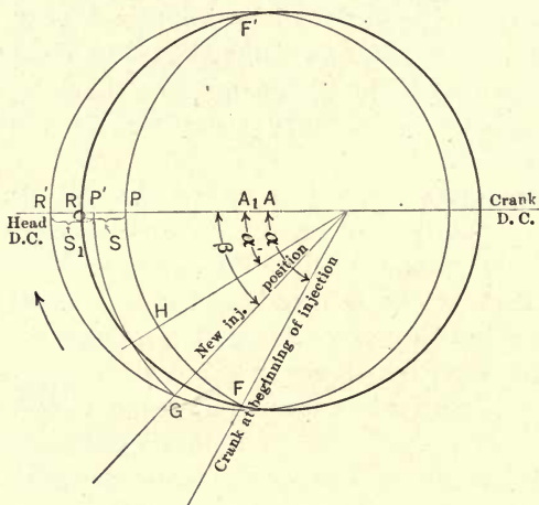
FIG. 307.—Fuel timing control.
