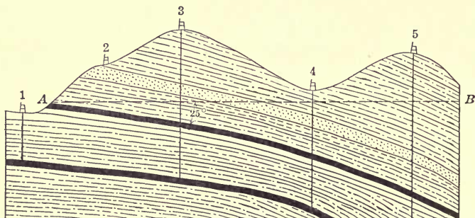
FIG. 37.—Shows effect of topography in choosing well sites.
