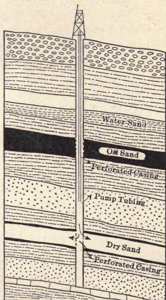
FIG. 67.—Shows oil entering dry sand below.
