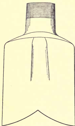
FIG. 56.—Fish tail rotary bit.
