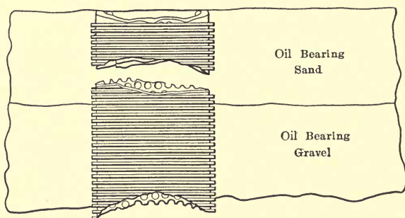
FIG. 63.—Oil well screen.
