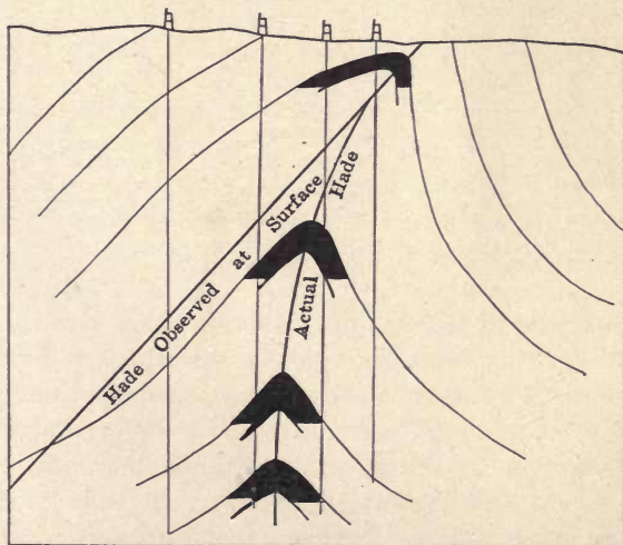
FIG. 50.—Shows curving of axis underground. (After Craig.)
