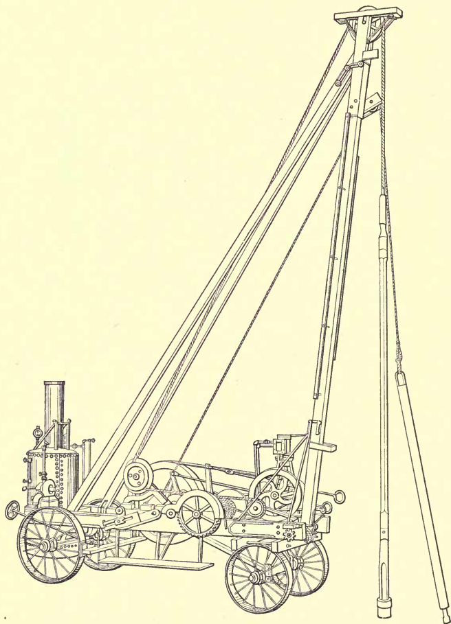
FIG. 51.—Portable drilling rig.
