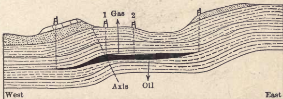
FIG. 15b.—Cross-section of a terrace.
