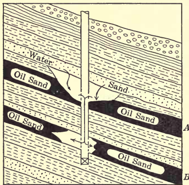
FIG. 72.—Water from top stratum entering zones A and B due to caving of shale above A resulting from withdrawal of sand.
