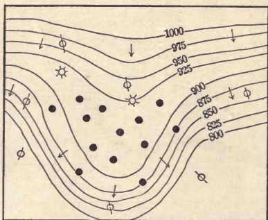
FIG. 15a.—Contour map of a terrace.
