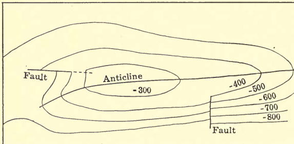
FIG. 30.—Contour map of faulted anticline. (After U. S. G. S.)
