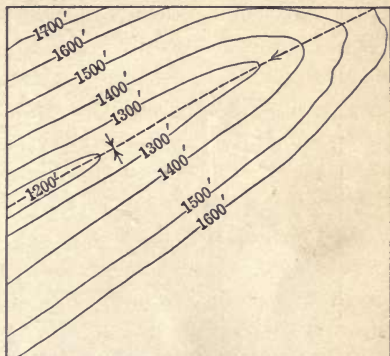
FIG. 27b.—Shows method of expressing syncline by contours.
