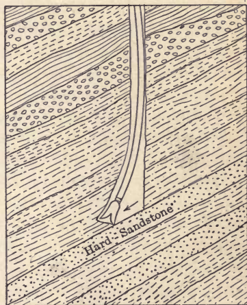
FIG. 54.—Rotary bit following hard stratum.
