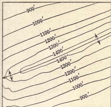
FIG. 27a.—Shows method of expressing an anticline by contours.
