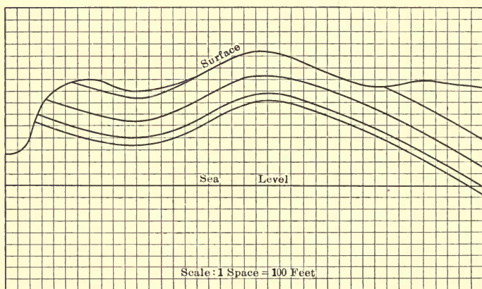
FIG. 48.—Graphic method of finding depth.
