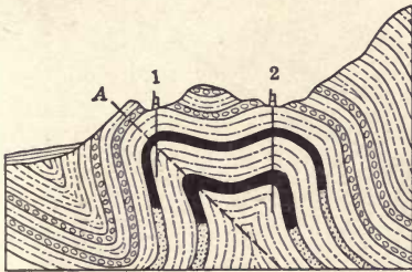
FIG. 43.—Illustrates well locations on minor folds of a highly compressed structure.
