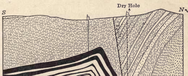
FIG. 24.—Shows effect of faulting. Dry hole to right of fault. (After U. S. G. S.)
