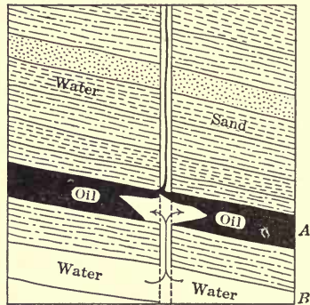
FIG. 69.—Water in full control of B and entering A.
