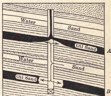
FIG. 71.—Water between A and B entering both sands. Water above A .
