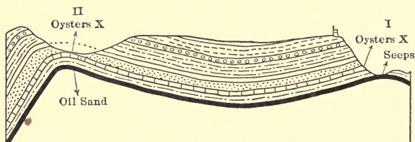
FIG. 6.—Illustrates the use of fossils in correlating formations.
