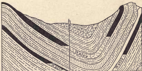
FIG. 12.—Illustrates an asymmetrical syncline.
