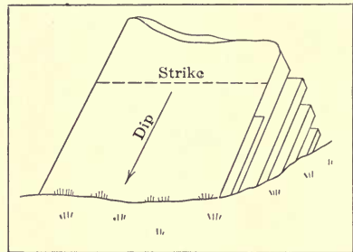
FIG. 36.—Strike and dip. (After Geikie.)
