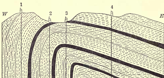
FIG. 38.—Illustrates locating wells on an asymmetrical anticline.
