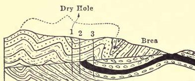
FIG. 25a.—Illustrates thrust fault.
