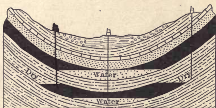
FIG. 11.—Illustrates possibility of finding oil in synclines.
