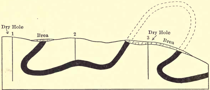
FIG. 13.—Illustrates complex folding. (After U. S. G. S.)
