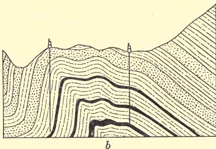
FIGS. 9a and 9b.—Types of asymmetrical anticlines.
