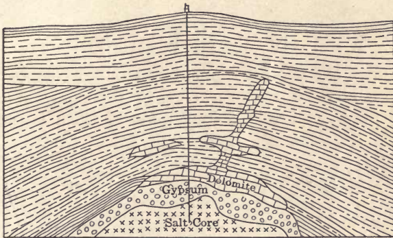
FIG. 20.—Illustrates saline dome. Oil occurs in the dolomite. (After Lee Hager.)
