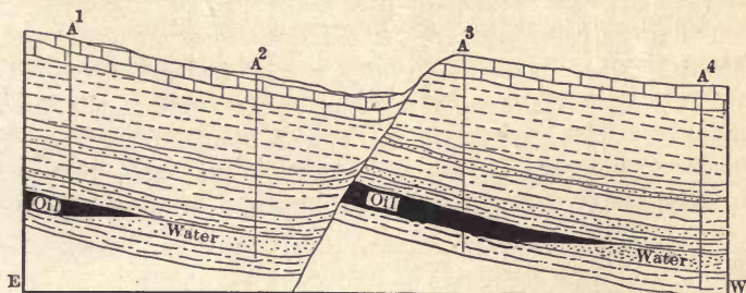
FIG. 40.—Illustrates how the upthrow side of a fault acts as an anticline; the downthrow side, as a syncline.
