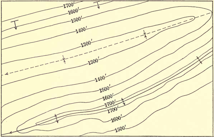
FIG. 29.—Anticline, syncline, and monocline.
