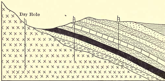
FIG. 14.—Illustrates wells on a monocline.
