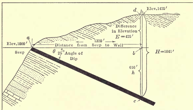
FIG. 47.—Method of estimating the dip of a bed.
