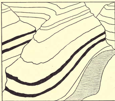
FIG. 39.—Shows how erosion exposes oil sands to drainage.
