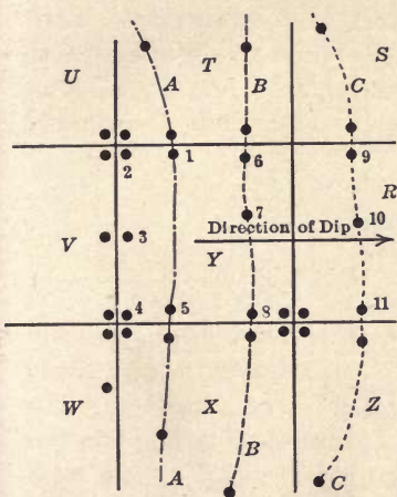
FIG. 61a.—Shows plan of wells and limits of sands, A , B , and C .
