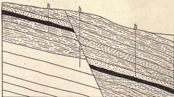
FIG. 41.—Illustrates how normal faulting may leave barren spaces.
