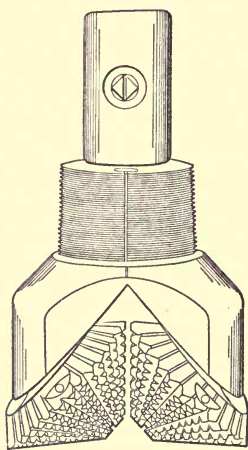
FIG. 57.—Sharp and Hughes hard rock rotary bit.
