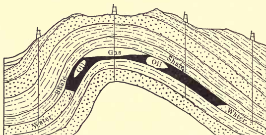
FIG. 1.—Illustration of ideal anticlinal conditions. 1
