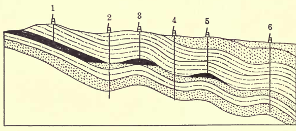
FIG. 42.—Shows lower fold non-productive; folds higher on slope increase in quantity of oil.
