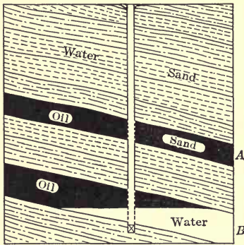
FIG. 68.—Water in partial control of zone B.
