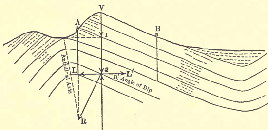
FIG. 59.—Illustrates direction of resultant L , which tends to collapse casing.
