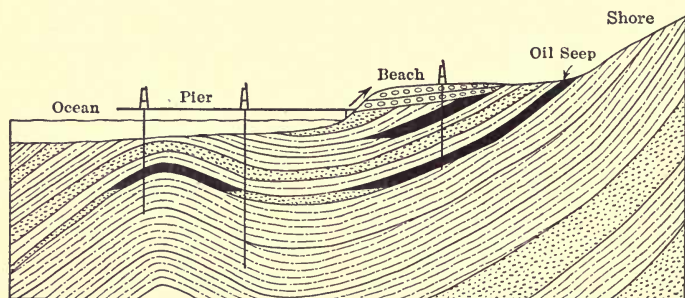
FIG. 45.—Illustrates oil out in ocean; derricks on piers.
