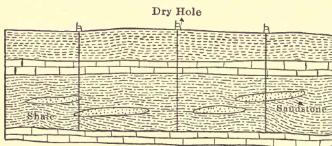
FIG. 16.—Illustrates sand lenses in a shale formation.
