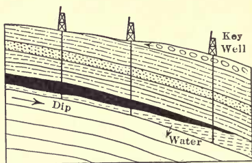
FIG. 66 b .—Cross-section showing drainage by key well.
