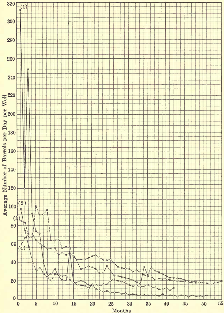
FIG. 61c.—Typical production curves of wells in the Mid-continent oil field. Curves represent production under leases as follows: 1, Muskogee district, Oklahoma; 2, Bartlesville district, Oklahoma; 3 and 4, Glenn pool, Oklahoma. (After U. S. Bureau of Mines.)
