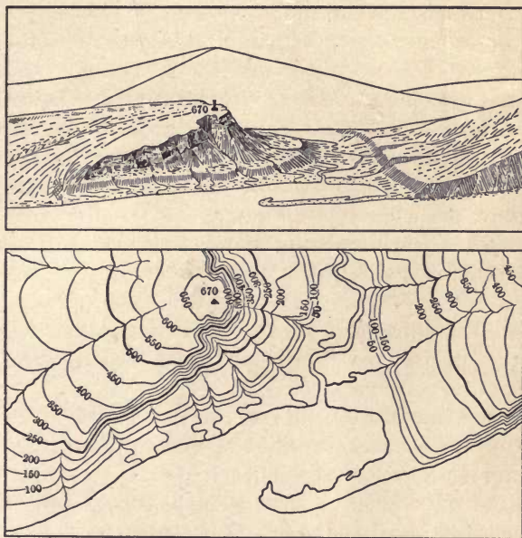
FIG. 26.—Ideal sketch and corresponding contour map. (After U. S. G. S.)
