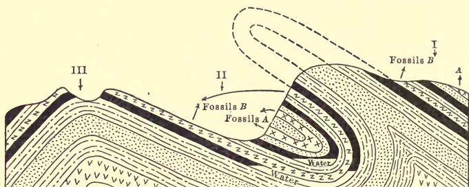
FIG. 5.—Illustrates the use of fossils in correlating formations.
