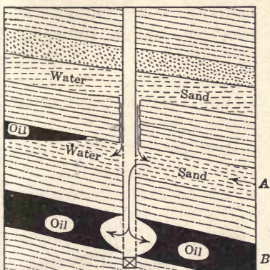
FIG. 70.—Water in partial control of A and beginning to flood B .
