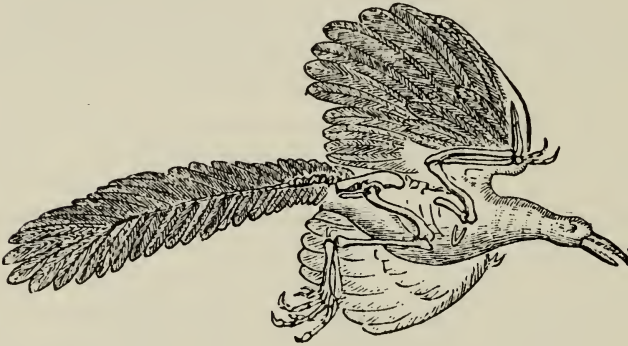
THE ARCHEOPTERYX (OF THE OOLITE STRATA).
