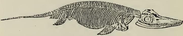
SKELETON OF AN ICHTHYOSAURUS.
