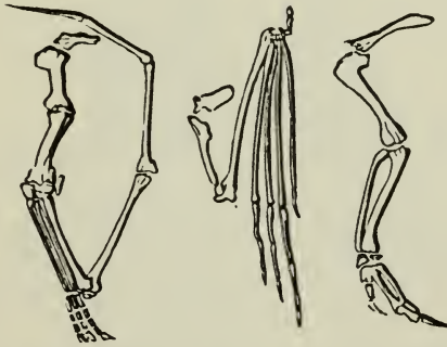
WING-BONES OF PTERODACTYL, BAT, AND BIRD.
