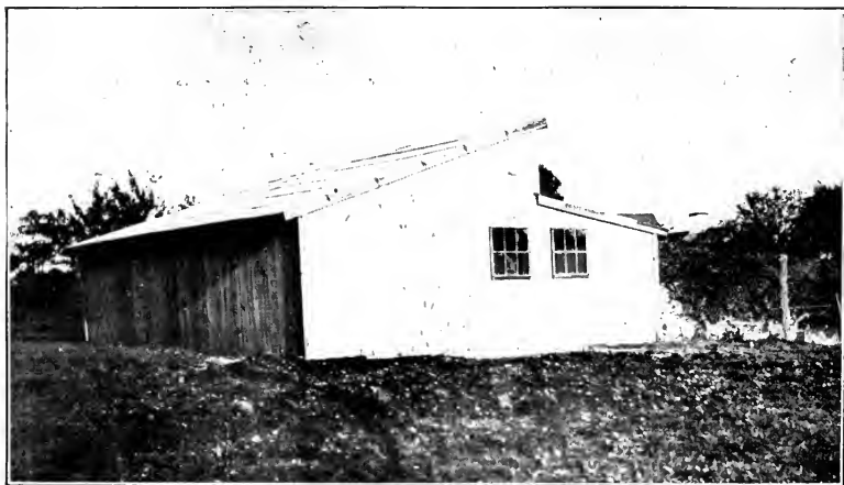
View of north and west sides of Dr. P. T. Woods' Improved Open-air Poultry House as completed and ready for painting. Roof is covered with Amatite. (Photo by Dr. Woods.)
