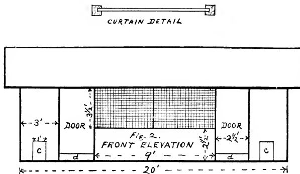
Fig. 18. Front elevation and curtain detail Gillette open-air poultry house. Wire front, 3\frac{1}{2}\times 9 feet, always open; "c, c" poultry slides; "d, d" movable boards to keep litter or sand out of doorway.
