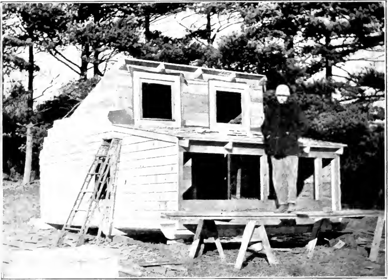
Building a portable colony type Woods' open-air poultry house, 10x16 ft., Wozelma Farms Producing Company, Silver Lake, Mass.
