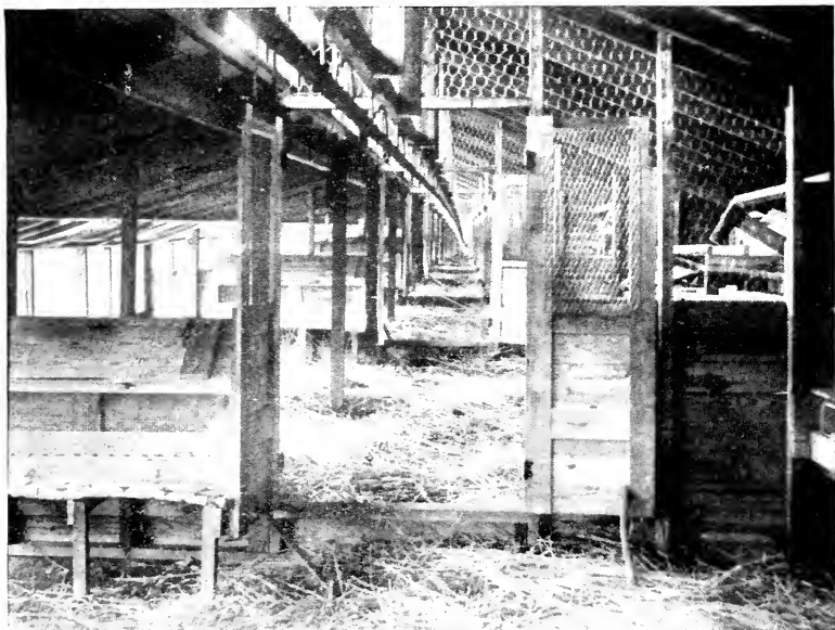
Interior view of F. M. Peasley's fresh-air house for 2,000 layers, Cheshire, Conn. Shows arrangement of track for feed car, hoppers, roosts, partitions, etc. (See page 64.)
