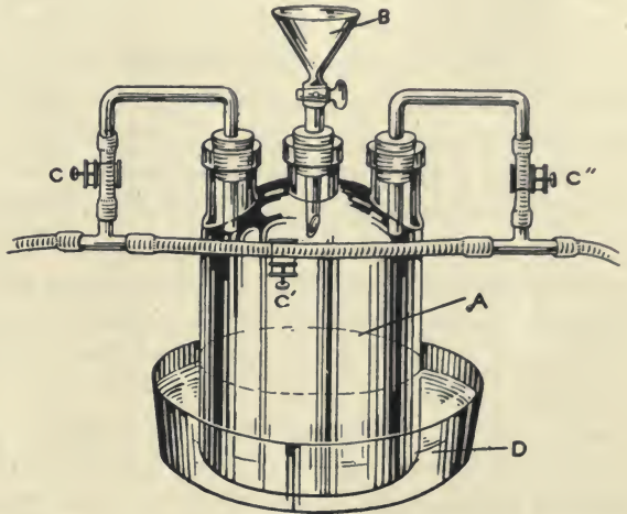
FIG. 21.—SURFACE VAPORIZER. A, Wolf bottles, containing ether; B, filling funnel; C, C', C'', control clamps; D, basin of water.
