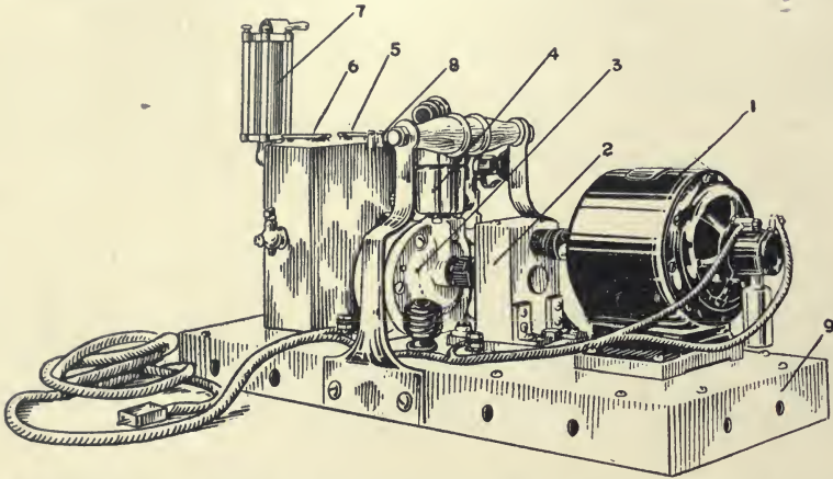
FIG. 20.—GENERATOR FOR COMPRESSED AIR: CONNELL PORTABLE MODEL. 1, Electric motor; 2, gears, oil-housed; 3, rotary compressor; 4, muffler; 5, oil tank and separator; 6, humidifier and air filter; 7, instantaneous air flow gauge; 8, safety valve; 9, hollow bottom with control rheostat.
