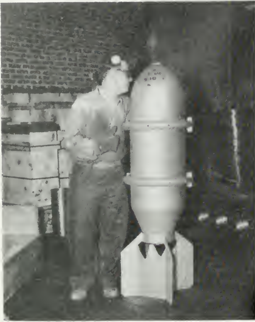
A 500-POUND DEMOLITION BOMB ready for shipment to a loading plant to be filled with high explosives. (Fins are attached for photographic purposes.)
