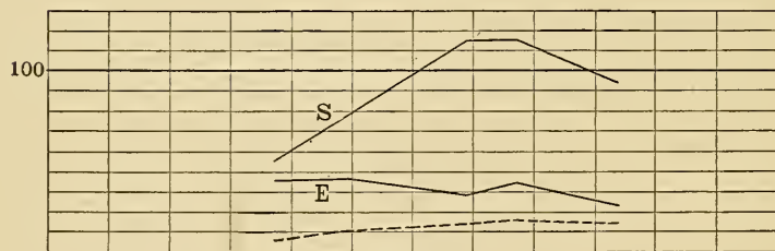
FIG. 45.—Sun-box records for south and east exposures. The dotted lines show the temperature of the air; the full lines the temperatures within the boxes. The figures at the top denote the hours of the day. The divisions of the vertical scale are equal to ten degrees of temperature.
