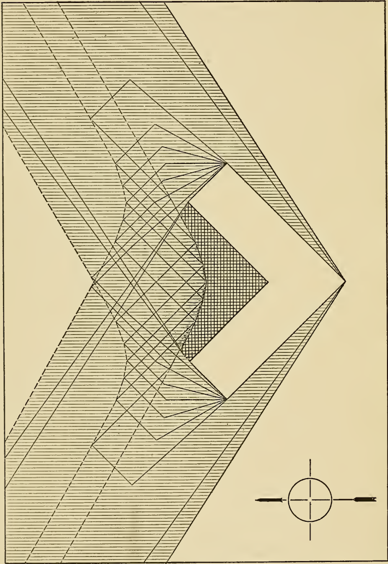
FIG. 21. — Showing method of obtaining the area of complete shadow. The height of the block is taken at one-half its width. Note that in Fig. 19 the height of the block is taken as equal to its width. Winter solstice. Lat. 42^{\circ} - 0' N.
