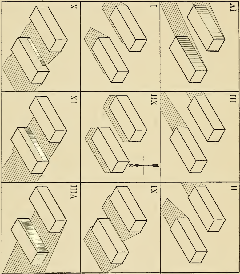
FIG. 29. — Showing the shadows cast by two single straight blocks side by side; winter solstice; Lat. 42^{\circ} N.
