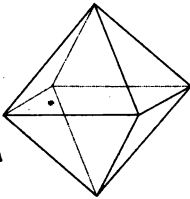
2. Octaeder.
