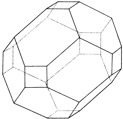
Octo-Tetraeder.
