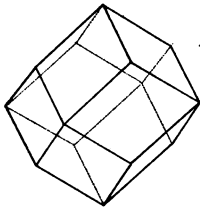
5. Dodecaeder.
