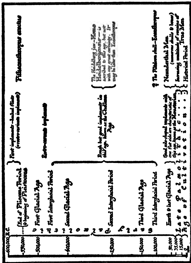
TIME DIAGRAM OF THE GLACIAL AGES.
