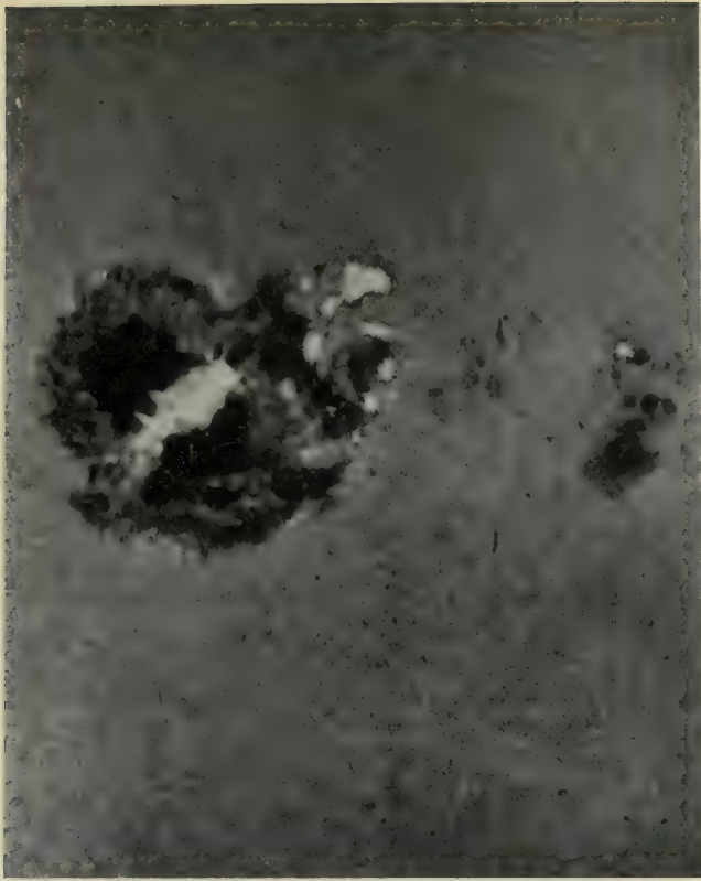
FIG. 9.—THE GREAT SUN-SPOT OF JULY 17, 1905
