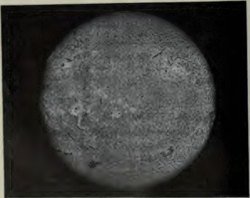
FIG. 8.—THE SUN
