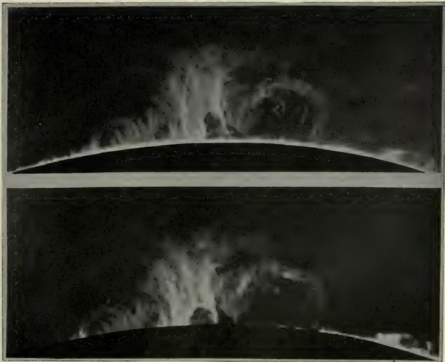
FIG. 10.—SOLAR PROMINENCES
