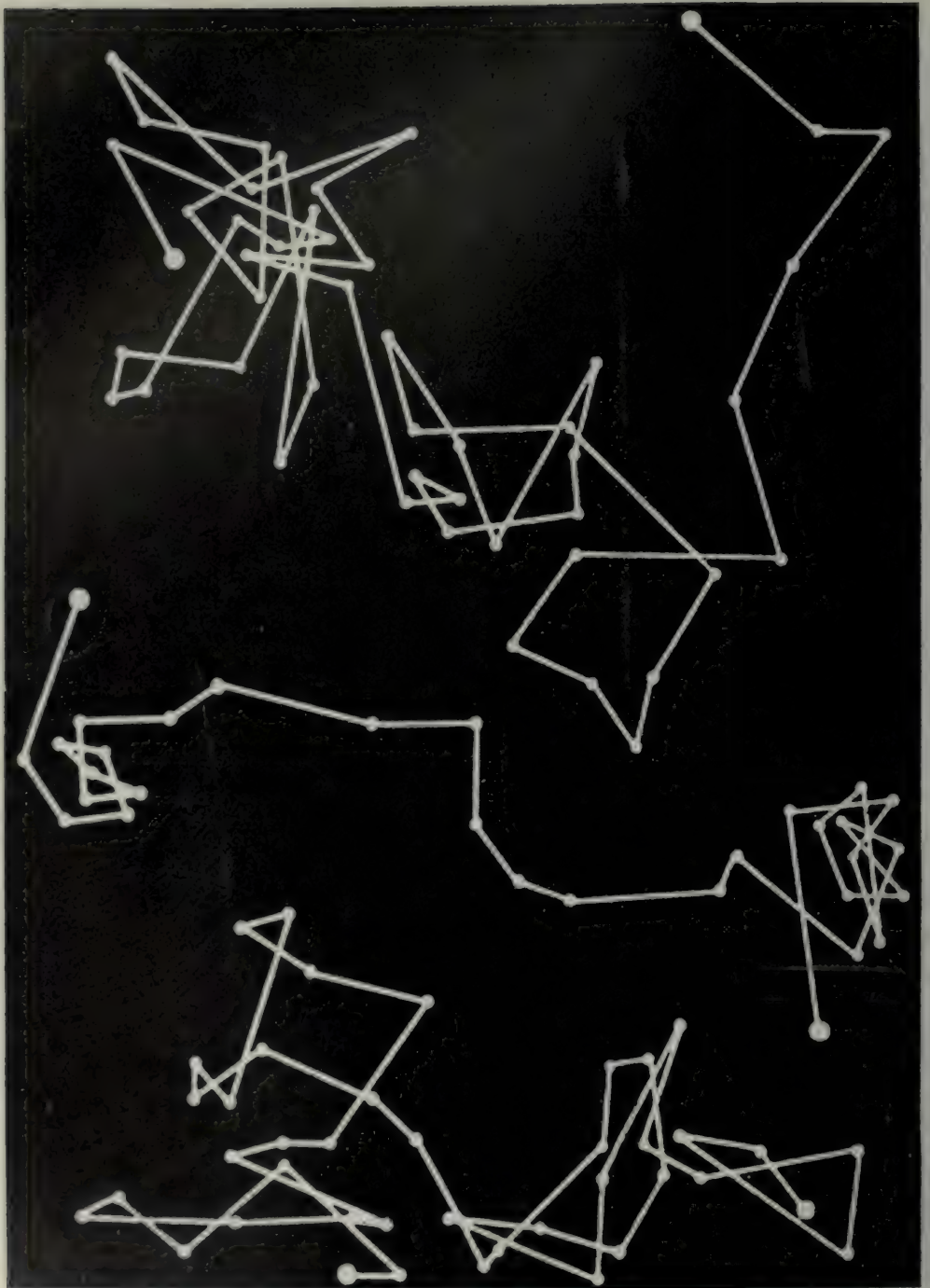
THE BROWNIAN MOVEMENT
