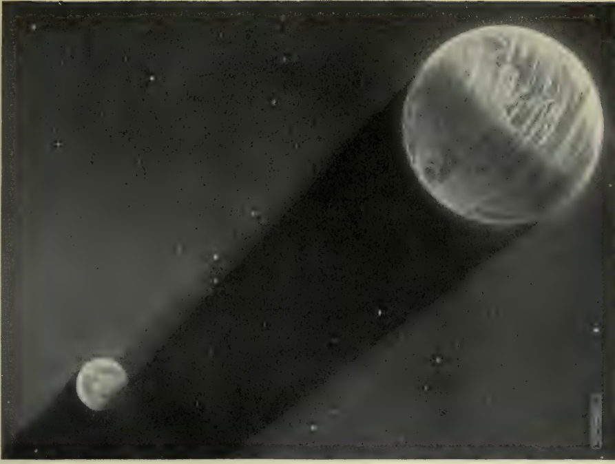
FIG. 3 —THE MOON ENTERING THE SHADOW CAST BY THE EARTH The diagram shows the Moon partially eclipsed.
