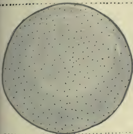
THE RELATIVE SIZES OF ATOMS AND ELECTRONS
