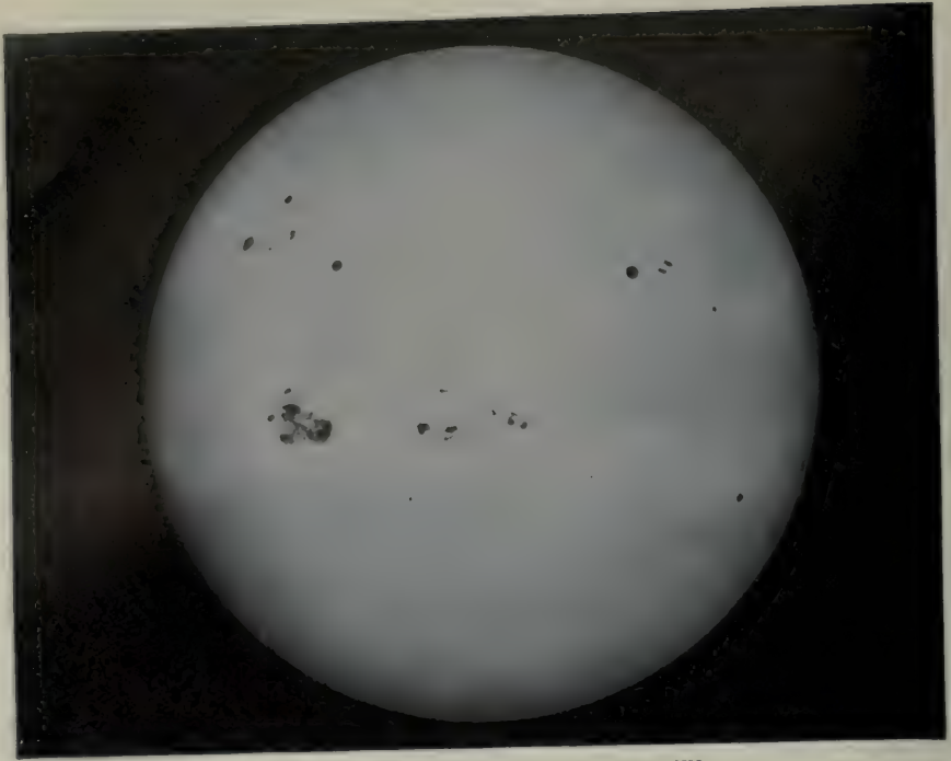
FIG. 7.—THE VISIBLE SURFACE OF THE SUN
