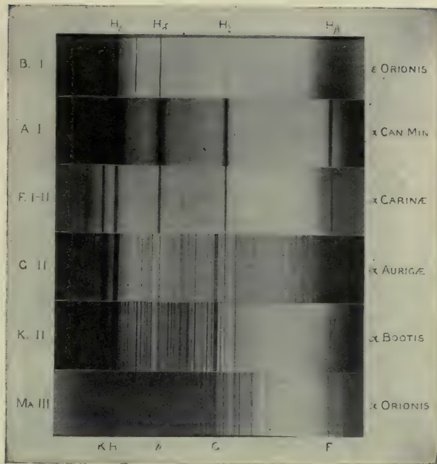
FIG. 21.—TYPICAL SPECTRA
