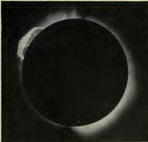
FIG. 6.—SOLAR PROMINENCES SEEN AT TOTAL SOLAR ECLIPSE, May 29, 1919. TAKEN AT SOBRAL, BRAZIL.
