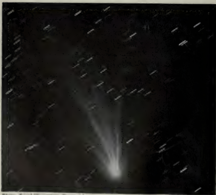
FIG. 20.—COMET, October 3, 1908
