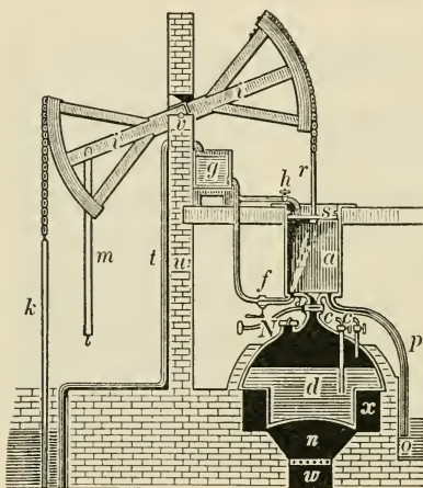
FIG. 93. NEWCOMEN'S STEAM ENGINE
